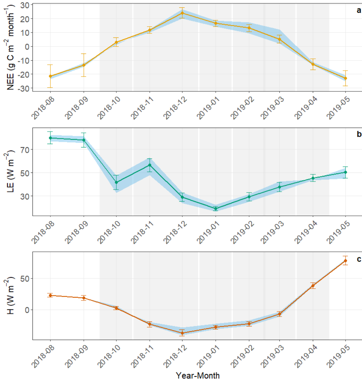
Figure 5. Monthly aggregated fluxes at the Nam Co site from August 2018 to May 2019:(a) net ecosystem exchange of CO 2 (NEE, g C m -2 month -1 ), (b) latent heat flux (LE, W m -2 ), and(c) sensible heat flux (H, W m -2 ). Shaded blue ribbons indicate the spread between the 5 % and 95 % u* filtering scenarios. Orange (NEE), green (LE), and red (H) lines and points represent the median estimate (50 % scenario). Vertical error bars denote the total monthly uncertainty, including random error and gap-filling uncertainty. Grey background shading highlights the non-growing season (NGS, October–April), while unshaded periods represent the growing season (GS, May–September). Partial months (July 2018 and June 2019) were omitted to avoid bias.
