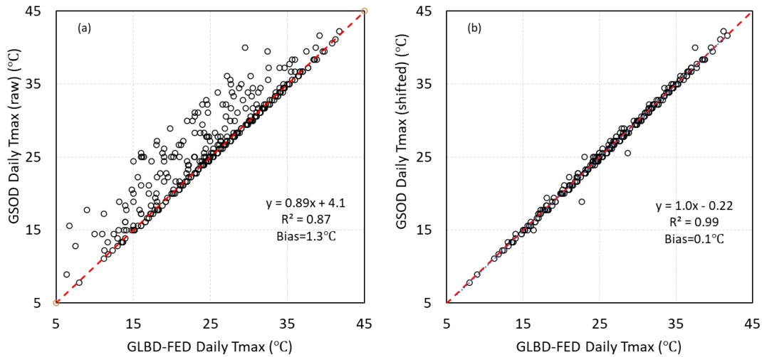
648 Figure 18 The comparison of daily Tmax at Villa Reynolds Argentina (873280-99999) between 649 GLBD-FED and GSOD in 2022. Panel a is the comparison between GLBD-FED and original GSOD 650 data, while panel b is the comparison between GLBD-FED and date shifted (forward moving) GSOD 651 data.
