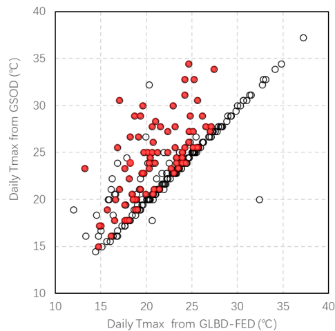
592 Figure 16 A comparison of daily Tmax values at the Plettenberg Bay station (689310-99999), South 593 Africa, for the year 2024. The abscissa and ordinate represent the daily values from the GLBD-FED 594 and GSOD datasets, respectively. The red solid dots indicate the data that are repeated with their 595 previous ones (86 points), while the black hollow dots represent non-repeating values (172 points).
