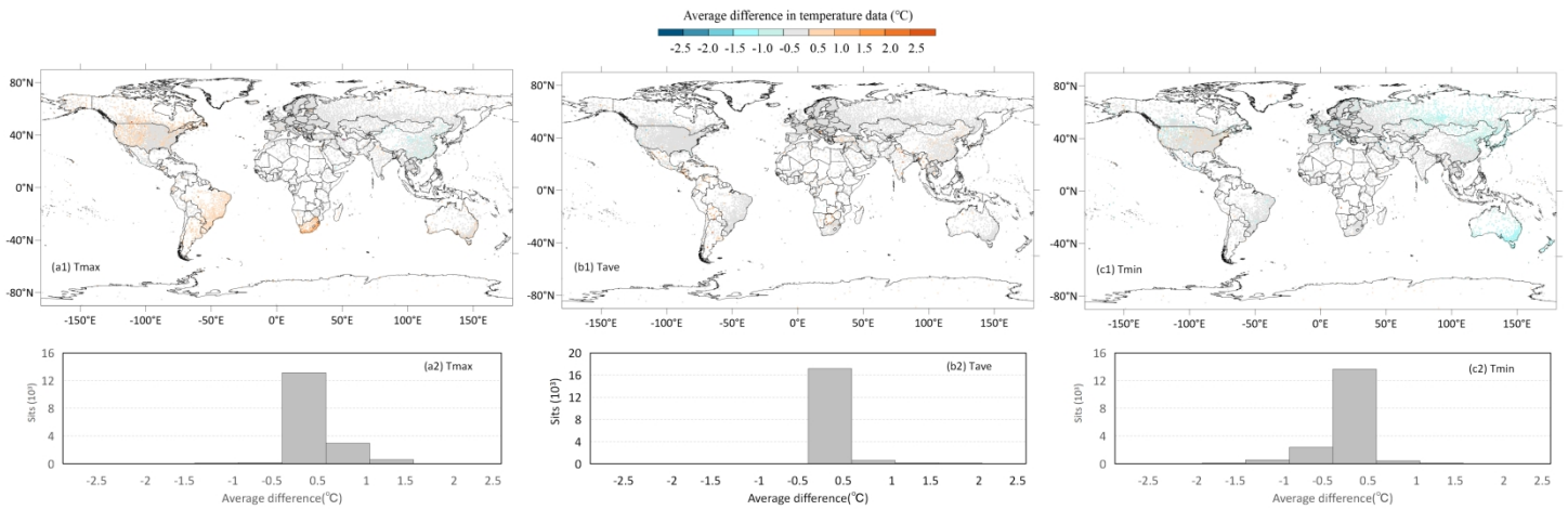
Figure 14 Spatial distribution of the difference in in-situ daily temperature data between GLBD-FED and GSOD during 1981–2024 (GSOD minus GLBD-FED). Panels a1, b1, c1 show the difference in Tmax, Tave and Tmin at each site. Panels a2, b2, c2 represent the site number distribution with diversities.
