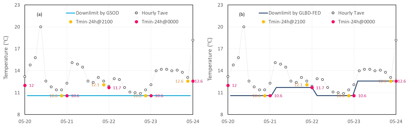
568 Figure 15 The lower-bound estimate of air temperature derived from the daily Tmin values based on 569 GSOD (light blue, panel a) and GLBD-FED (dark blue, panel b) at the SINPO station (470460), North 570 Korea, May 20–23, 2014.
