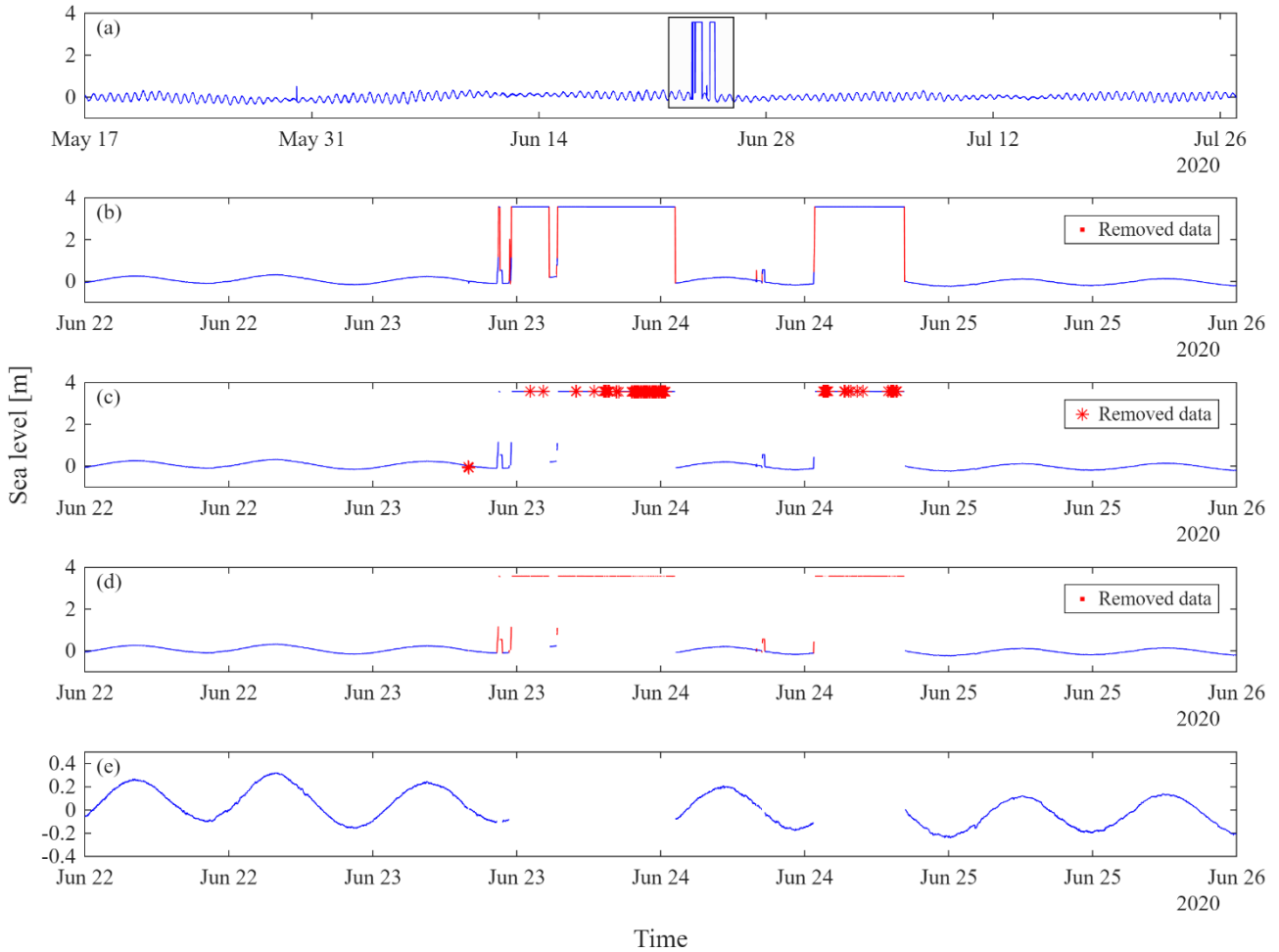
315 Figure 5. The key steps involved in data processing using the example of Aigio station in Greece. (a) The raw record adjusted to a regular time interval, with the mean value subtracted. The portion of the record that is zoomed in in (b)-(e) is indicated within the rectangle. Erroneous data points, indicated in red, are identified during the following procedures: (b) the out-of-range correction method, (c) the automatic spike detection and (d) visual inspection. (e) The final record after quality control steps.
