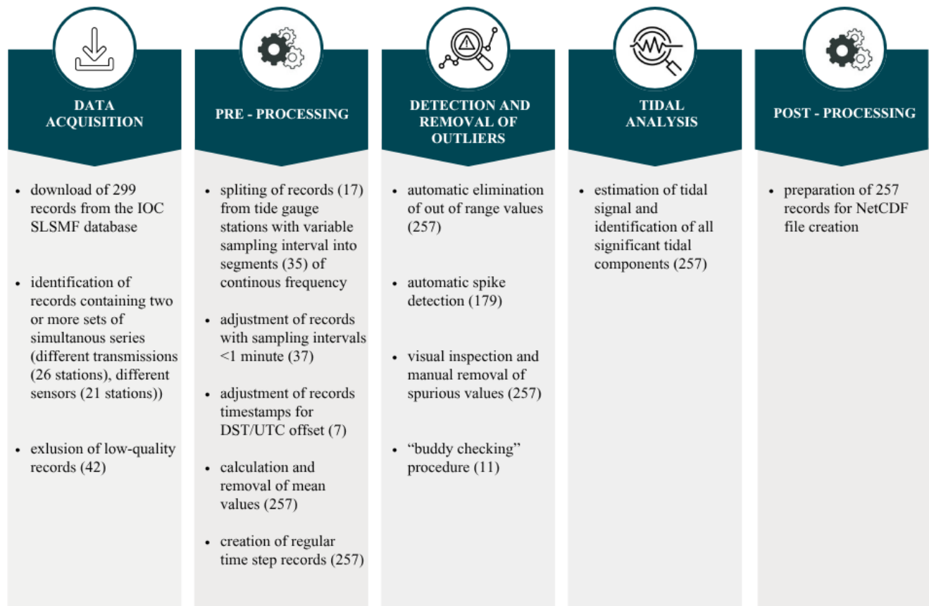
Figure 4. Flow chart of data processing. The numbers in parentheses indicate how many records have passed each step. Automatic spike detection (179) was applied only to 1-minute time series.
