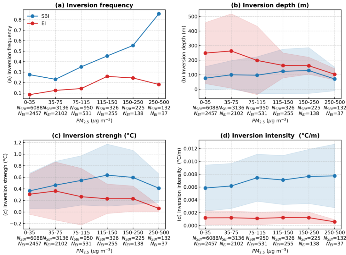
545 Figure 11: Statistics of inversion characteristics across different PM_{2.5} concentration bins at XH during 2018-2019. Panels show (a) inversion frequency, (b) inversion depth, (c) inversion strength ( \Delta T ), and (d) inversion intensity ( \Delta T/\text{depth} ) for surface-based inversions (SBI, blue) and elevated inversion (EI, red). The specific number of inversion layers used for statistical analysis ( N_{SBI} and N_{EI} ) is indicated on the x-axis for each bin. Error bands indicate \pm 1 standard deviation.
