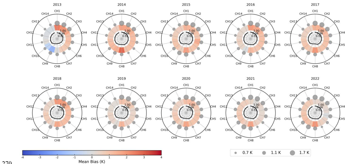
Figure 4: Ten-year (2013–2022) polar summary of the agreement between observed and ERA5-simulated brightness temperatures for all 14 channels. Each subplot shows one year, with the inner black solid curve representing the R , the middle colour shaded ring indicating the mean bias, and the circle marker sizes in the outer ring representing the standard deviation of differences. The bottom horizontal colorbar denotes the bias scale, and the adjacent legend explains the marker sizes for standard deviation
