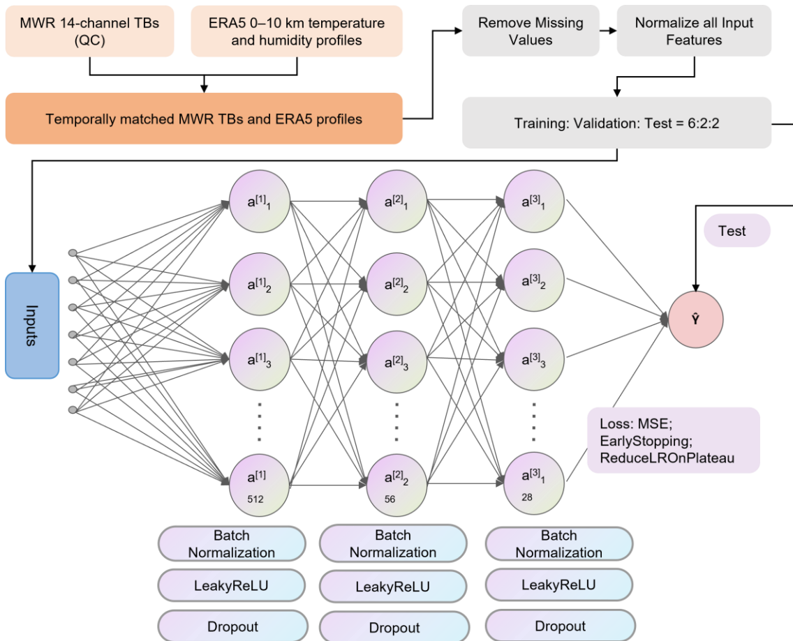
Figure 5: Flowchart of DNN model construction.
