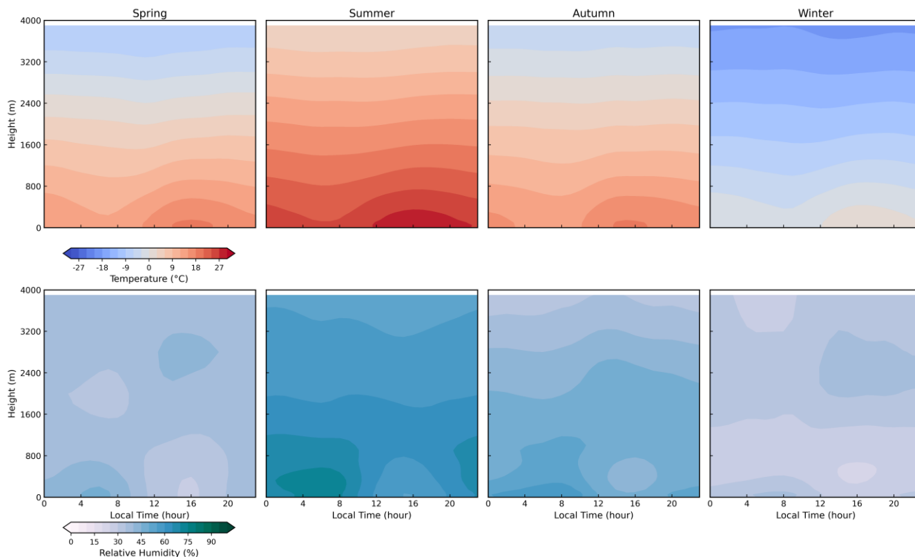
Figure 9: Seasonal diurnal variations of temperature and relative humidity at XH during 2013–2022. The statistics are based on the merged 495 retrieval dataset (OE for clear-sky and DNN for cloudy-sky conditions). Upper panels show temperature profiles (°C) and lower panels show relative humidity profiles (%). Data are averaged by hour in local standard time (LST, UTC+8). Contour shading indicates the mean diurnal evolution at each vertical level, with height restricted to 0–4000 m. Colour bars at the bottom correspond to the respective variables. Seasonal panels are arranged from spring (March–May), summer (June–August), autumn (September–November) to winter (December–February).
