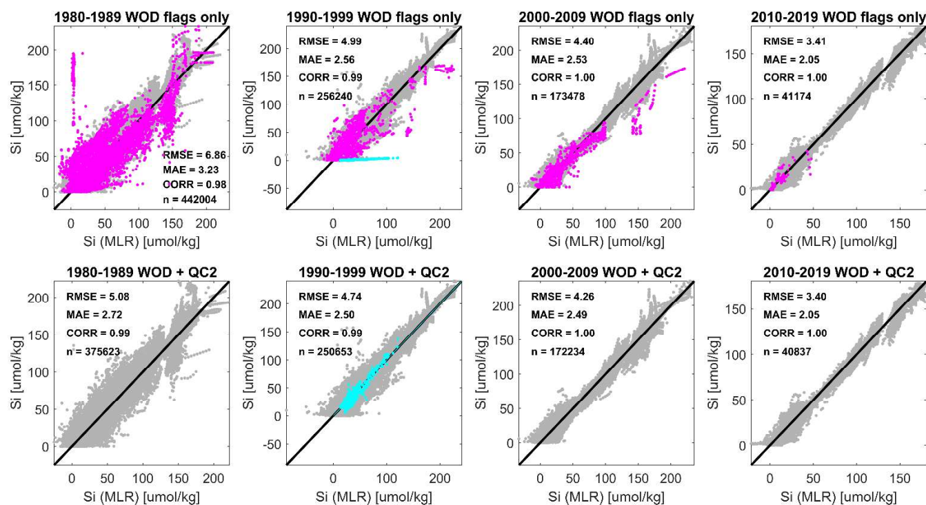
880 Figure A2. Secondary quality control (QC) comparison of silicate concentrations from the World Ocean Database (2018) bottle 885 sample dataset (OSD), showing predicted concentrations from regionalized Multiple Linear Regression (MLR) models (functions of salinity, temperature, and dissolved oxygen, x-axes) with corresponding observed values (y axes), both in mass-specific units ( \mu\text{mol} \text{kg}^{-1} ), for different decades (left to right subplots), and before/after applying the secondary QC exclusions and corrections (upper/lower subplots). Magenta color denotes suspect data based on secondary QC, and cyan denotes data that are corrected for units confusion by the secondary QC. All data shown have passed the primary QC from WOD18 (flag value = 0, 'accepted' values). Black lines are 1:1, and skill metrics measuring agreement level between observed and modelled values include: Root Mean Square Errors (RMSE), Mean Absolute Errors (MAE), Pearson correlations (CORR), and the number of model-observation pairs (n).
