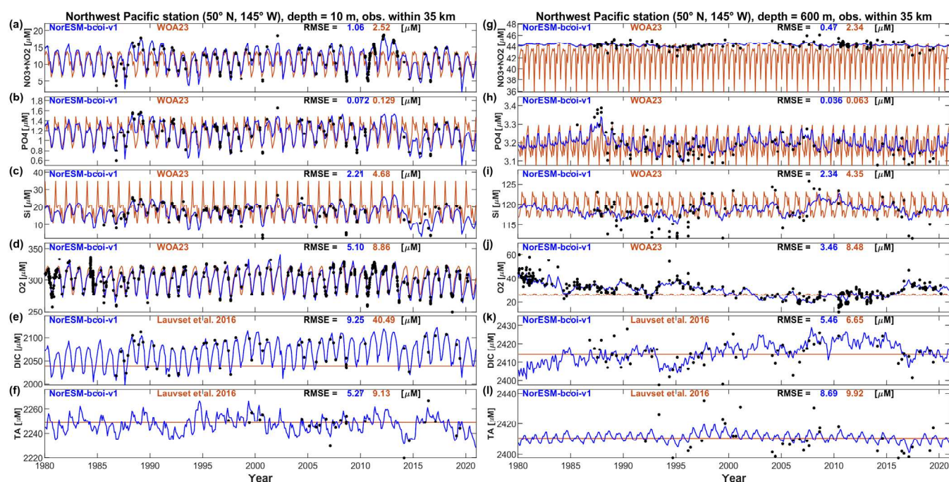
505 Figure 7. Northwest Pacific station time series comparison, showing monthly estimates from the NorESM-bcoi-v1 product (blue lines), the World Ocean Atlas 2023 or GLODAP gridded (Lauvset et al., 2016) climatologies (orange lines), and all in situ observations within 35 km of the nominal station location ( 50^\circ \text{N} , 145^\circ \text{W} ) (black dots). Rows from top to bottom show data for nitrate-plus-nitrite ( \text{NO}_3+\text{NO}_2 ), phosphate ( \text{PO}_4 ), silicate (Si), dissolved oxygen ( \text{O}_2 ), dissolved inorganic carbon (DIC), and total alkalinity (TA), all in in-situ volume specific units ( \mu\text{mol L}^{-1} ). Columns show data at 10m depth (left) and 600m depth (right), applying linear vertical interpolation to product and observational profiles where necessary. Each subplot shows Root Mean Square Error (RMSE) values relative to observational values for the NorESM-bcoi-v1 product (blue) and the WOA23 or Lauvset et al. 2016 climatological product (orange).
