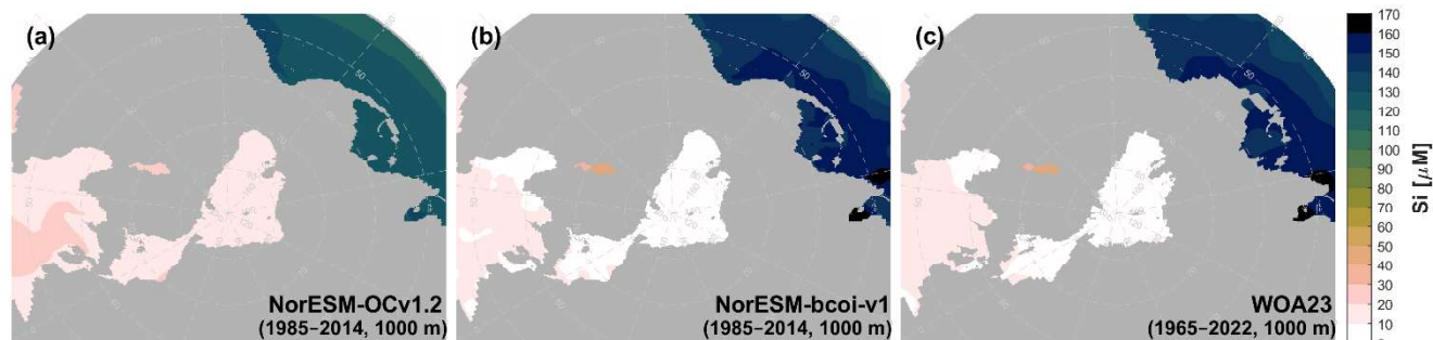
970 Figure A12. Annual climatology comparison for silicate at 1000 m depth, showing estimates from NorESM-OCv1.2 (left), NorESM-bcoi-v1 (middle), and the World Ocean Atlas 2023 (right). All concentrations are in in-situ volume-specific units ( \mu\text{mol L}^{-1} ).
