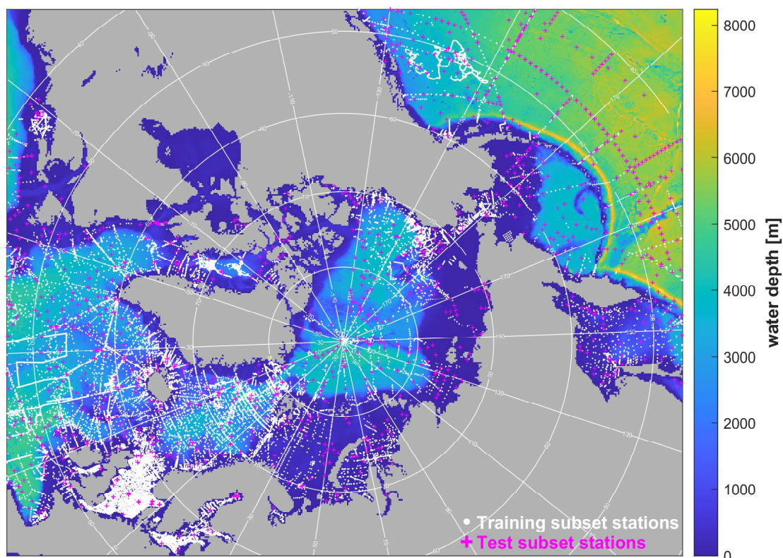
370 Figure 5. Training and test observational datasets for nitrate+nitrite (white dots and magenta crosses respectively). No test data locations (stations) overlap with training data locations, and test locations are selected to mimic the level of spatial interpolation implicit in application of the final model product. Background shows ETOPO1 bathymetry and white lines mark latitude/longitude on a polar stereographic projection.
