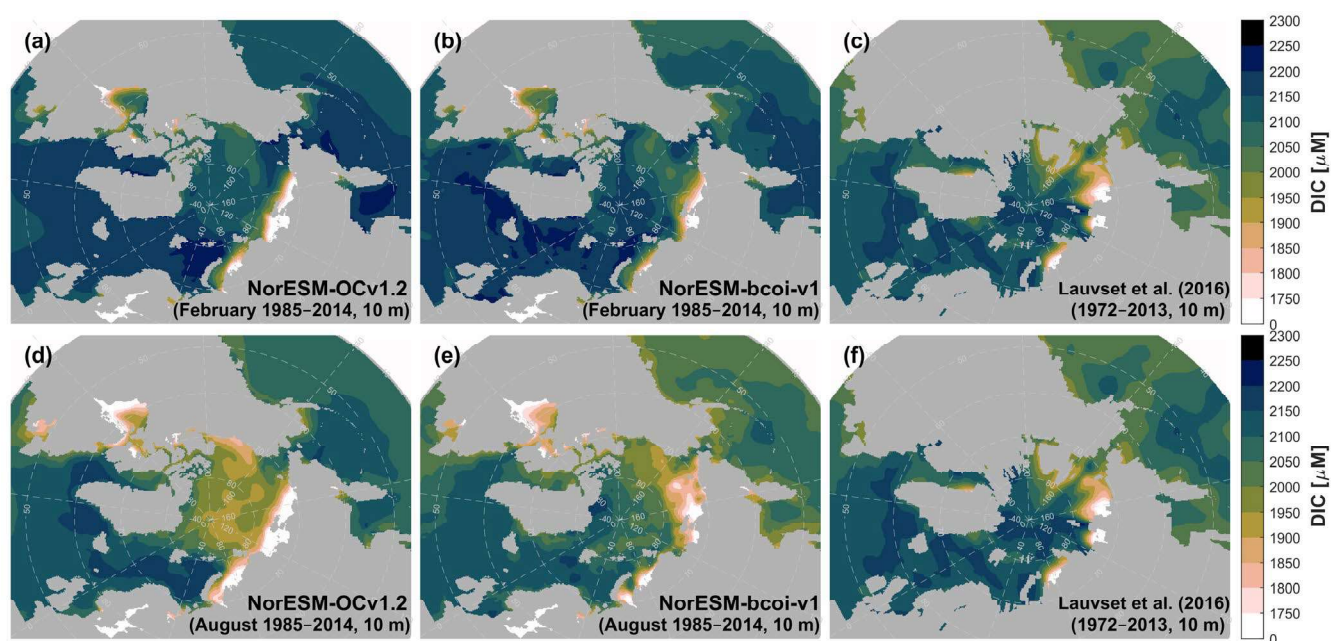
585 Figure 12. Climatology comparison for dissolved inorganic carbon at 10 m depth, for February (upper) and August (lower), showing estimates from the uncorrected hindcast NorESM-OCv1.2 (left), the final reanalysis product NorESM-bcoi-v1 (middle), and the GLODAP gridded product (Lauvset et al., 2016) (right). All concentrations are in in-situ volume-specific units ( \mu\text{mol L}^{-1} ).
