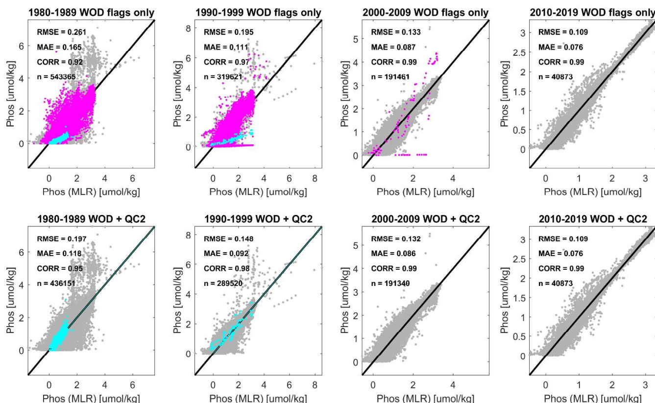
865 Figure A1. Secondary quality control (QC) comparison of phosphate concentrations from the World Ocean Database (2018) bottle 870 sample dataset (OSD), showing predicted concentrations from regionalized Multiple Linear Regression (MLR) models (functions of salinity, temperature, and dissolved oxygen, x-axes) with corresponding observed values (y axes), both in mass-specific units ( \mu\text{mol} \text{kg}^{-1} ), for different decades (left to right subplots), and before/after applying the secondary QC exclusions and corrections (upper/lower subplots). Magenta color denotes suspect data based on secondary QC, and cyan denotes data that are corrected for units confusion by the secondary QC. All data shown have passed the primary QC from WOD18 (flag value = 0, ‘accepted’ values). Black lines are 1:1, and skill metrics measuring agreement level between observed and modelled values include: Root Mean Square Errors (RMSE), Mean Absolute Errors (MAE), Pearson correlations (CORR), and the number of model-observation pairs (n).
