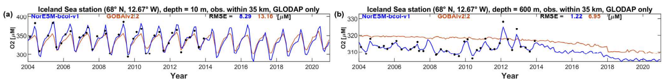
1030 Figure A21. Iceland Sea station time series comparison, showing monthly estimates of dissolved oxygen concentration (units \mu\text{mol L}^{-1} , in-situ volume specific) from the NorESM-bcoi-v1 product (blue lines) and the GOBAIv2.2 product (Sharp et al., 2023, orange lines), and all GLODAP-sourced observations from the NORBGCv1 dataset within 35 km of the nominal station location ( 68^\circ \text{ N} , 12.67^\circ \text{ W} ) (black dots). Columns show data at sampled depths of 10 m (left) and 600 m (right), applying linear interpolation to product profiles where necessary. Each subplot shows Root Mean Square Error (RMSE) values relative to observational values for the NorESM-bcoi-v1 product (blue) and the GOBAIv2.2 product (orange).
