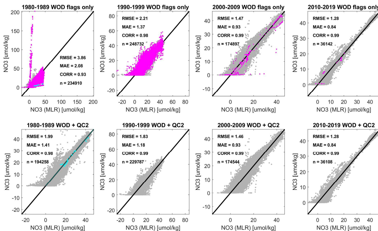
175 Figure 2. Secondary quality control (QC) comparison of nitrate-plus-nitrite concentrations from the World Ocean Database (2018) bottle sample dataset (OSD), showing predicted concentrations from regionalized Multiple Linear Regression (MLR) models (functions of salinity, temperature, and dissolved oxygen, x-axes) with corresponding observed values (y axes), both in mass-specific units ( \mu\text{mol kg}^{-1} ), for different decades (left to right subplots), and before/after applying the secondary QC exclusions and corrections (upper/lower subplots). Magenta colour denotes suspect data based on secondary QC, and cyan denotes data that are corrected for units confusion by the secondary QC. All data shown have passed the primary QC from WOD18 (flag value = 0, ‘accepted’ values). Black lines are 1:1, and skill metrics measuring agreement level between observed and modelled values include: Root Mean Square Errors (RMSE), Mean Absolute Errors (MAE), Pearson correlations (CORR), and the number of model-observation pairs (n).
