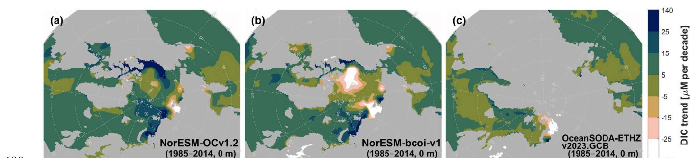
690 Figure 19. Dissolved inorganic carbon long term linear trends (30 years, 1985–2014) from annual averages at 0 m depth, showing estimates from the uncorrected hindcast NorESM-OCv1.2 (left), the final reanalysis product NorESM-bcoi-v1 (middle), and the OceanSODA-ETHZv2023.GCB gridded product (Gregor and Gruber, 2021) (right). All trends are in in-situ volume-specific units ( \mu\text{mol L}^{-1} per decade).
