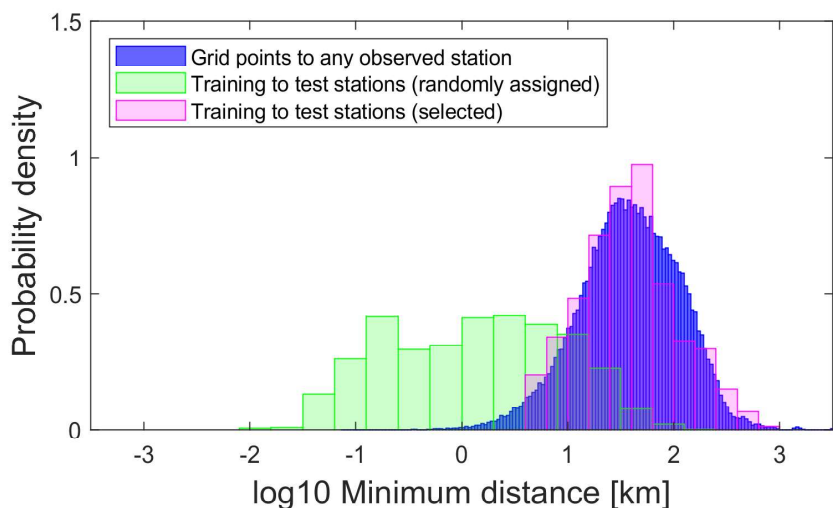
365 Figure 4. Probability distributions for nitrate-plus-nitrite of distances from model grid points to closest observational stations (blue), and of distances between test subset stations and closest training subset stations, first under simple random assignment (green) and then following our selection procedure (magenta). This latter was designed to provide more stringent cross validations that aim to measure interpolative accuracy in typical applications of the reanalysis products.
