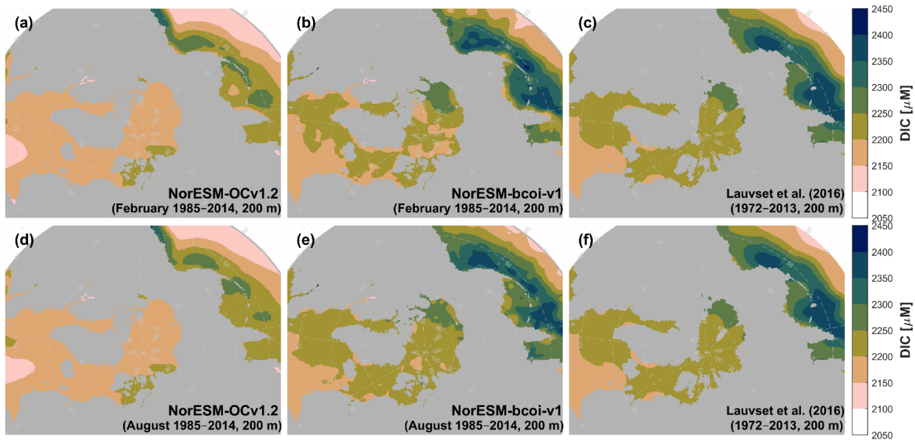
1015 Figure A17. Climatology comparison for dissolved inorganic carbon at 200 m depth, for February (upper) and August (lower), showing estimates from NorESM-OCv1.2 (left), NorESM-bcoi-v1 (middle), and the GLODAP gridded product (Lauvset et al., 2016) (right). All concentrations are in in-situ volume-specific units ( \mu\text{mol L}^{-1} ).
