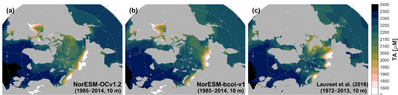
Figure A16. Annual climatology comparison for total alkalinity at 10 m depth, showing estimates from NorESM-OCv1.2 (left), NorESM-bcoi-v1 (middle), and the GLODAP gridded product (Lauvset et al., 2016) (right). All concentrations are in in-situ volume-specific units ( \mu\text{mol L}^{-1} ).
