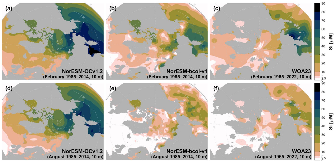
590 Figure 10. Climatology comparison for silicate at 10 m depth, for February (upper) and August (lower), showing estimates from the uncorrected hindcast NorESM-OCv1.2 (left), the final reanalysis product NorESM-bcoi-v1 (middle), and the World Ocean Atlas 2023 (right). All concentrations are in in-situ volume-specific units ( \mu\text{mol L}^{-1} ).
