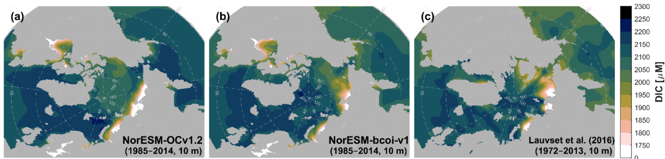
Figure A15. Annual climatology comparison for dissolved inorganic carbon at 10 m depth, showing estimates from NorESM-OCv1.2 (left), NorESM-bcoi-v1 (middle), and the GLODAP gridded product (Lauvset et al., 2016) (right). All concentrations are in in-situ volume-specific units ( \mu\text{mol L}^{-1} ).
