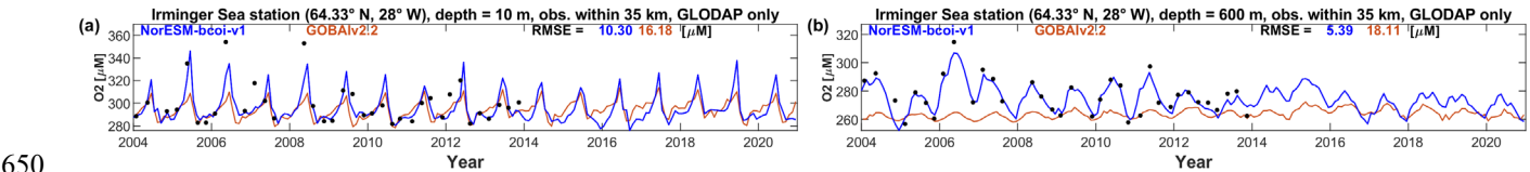
Figure 14. Irmingier Sea station time series comparison, showing monthly estimates of dissolved oxygen concentration (units \mu\text{mol L}^{-1} , in-situ volume specific) from the NorESM-bcoi-v1 product (blue lines) and the GOBAIv2.2 product (Sharp et al., 2023, orange lines), and all GLODAP-sourced observations from the NORBGCv1 dataset within 35 km of the nominal station location ( 64.33^\circ\text{ N} , 28^\circ\text{ W} ) (black dots). Columns show data at sampled depths of 10 m (left) and 600 m (right), applying linear vertical interpolation to produce profiles where necessary. Each subplot shows Root Mean Square Error (RMSE) values relative to observational values for the NorESM-bcoi-v1 product (blue) and the GOBAIv2.2 product (orange).
