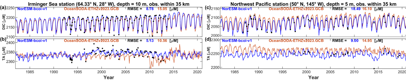
Figure 17. Time series comparisons for the Irminger Sea station (left) and Northwest Pacific station (right), at the shallowest sampled depths (10 and 5 m respectively, concentrations in units \mu\text{mol L}^{-1} , in-situ volume specific). Plots show monthly estimates of dissolved inorganic carbon (DIC, upper) and total alkalinity (lower) from the NorESM-bcoi-v1 product (blue lines) and the OceanSODA-ETHZ product (Gregor and Gruber, 2021, orange lines), and all in situ observations from the NORBGCv1 compilation within 35 km of the nominal station locations (black dots). Each subplot shows Root Mean Square Error (RMSE) with respect to observational values for the NorESM-bcoi-v1 product (blue) and the OceanSODA-ETHZ product (orange).
