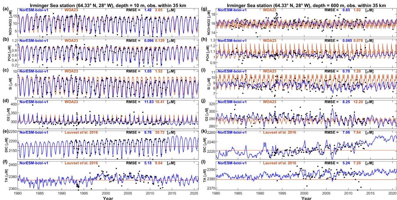
Figure A5. Irminger Sea station time series comparison, showing monthly estimates from the NorESM-bcoi-v1 product (blue lines), the World Ocean Atlas 2023 or GLODAPv2-gridded climatologies (Lauvset et al., 2016) climatologies (orange lines), and all in situ observations within 35 km of the nominal station location (64.33° N, 28° W) (black dots). Rows from top to bottom show data for nitrate-plus-nitrite (NO 3 +NO 2 ), phosphate (PO 4 ), silicate (Si), dissolved oxygen (O 2 ), dissolved inorganic carbon (DIC), and total alkalinity (TA), all in in-situ volume specific units (μmol L -1 ). Columns show data at 10 m depth (left) and 600 m depth (right), applying linear vertical interpolation to product and observational profiles where necessary. Each subplot shows Root Mean Square Error (RMSE) values relative to observational values for the NorESM-bcoi-v1 product (blue) and the WOA23 or Lauvset et al. 2016 climatological product (orange).
