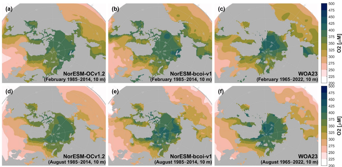
595 Figure 11. Climatology comparison for dissolved oxygen at 10 m depth, for February (upper) and August (lower), showing estimates from the uncorrected hindcast NorESM-OCv1.2 (left), the final reanalysis product NorESM-bcoi-v1 (middle), and the World Ocean Atlas 2023 (right). All concentrations are in in-situ volume-specific units ( \mu\text{mol L}^{-1} ).
