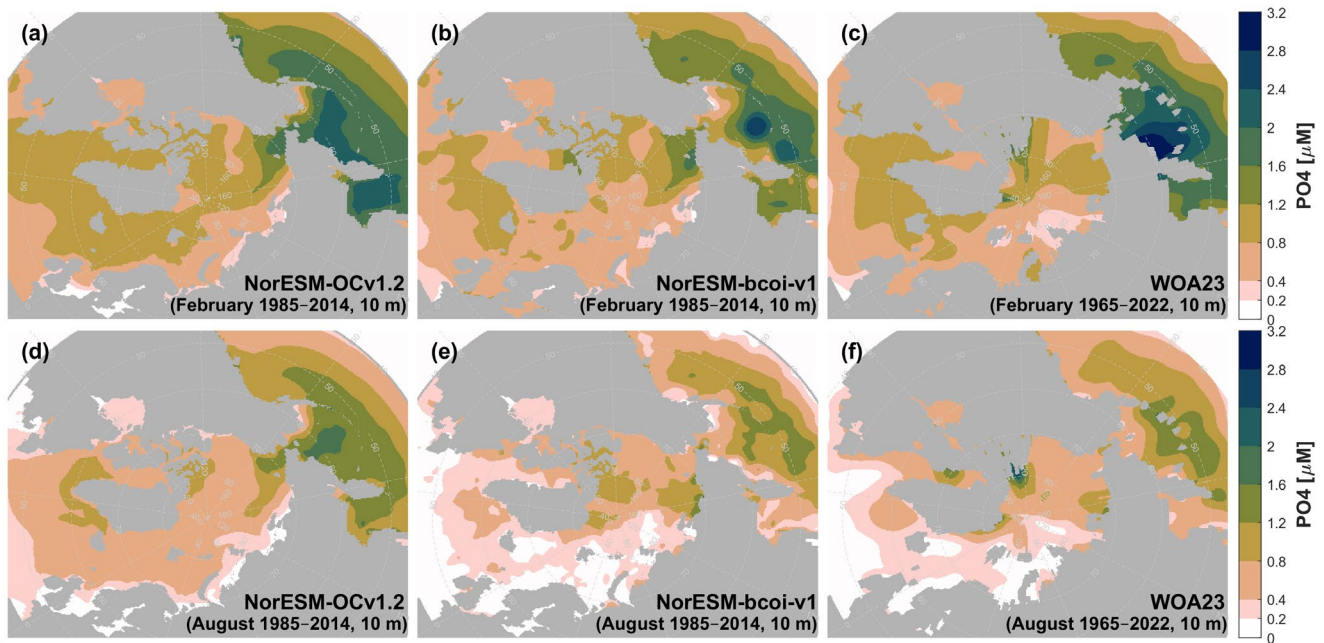
575 Figure 9. Climatology comparison for phosphate at 10 m depth, for February (upper) and August (lower), showing estimates from the uncorrected hindcast NorESM-OCv1.2 (left), the final reanalysis product NorESM-bcoi-v1 (middle), and the World Ocean Atlas 2023 (right). All concentrations are in in-situ volume-specific units ( \mu\text{mol L}^{-1} ).
