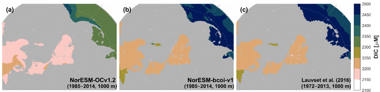
1020 Figure A18. Annual climatology comparison for dissolved inorganic carbon at 1000 m depth, showing estimates from NorESM-OCv1.2 (left), NorESM-bcoi-v1 (middle), and the GLODAP gridded product (Lauvset et al., 2016) (right). All concentrations are in in-situ volume-specific units ( \mu\text{mol L}^{-1} ).
