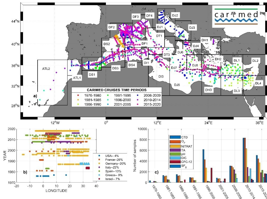
125 Figure 1: Overview of the cruises included in the CARIMED data synthesis products: (a) map showing the cruise stations included in CARIMED grouped by five year-periods with measurements; (b) spatiotemporal distribution of stations (year vs. longitude), coloured by Chief Scientist country, with the legend indicating the percentage of cruises per country; (c) histogram of the number 130 of samples per variable, grouped into five-year periods, with variables categorised as CTD (thermohaline variables), dissolved oxygen (O 2 ), dissolved inorganic nutrients represented with nitrate (NITRAT), total alkalinity (TA), pH, total dissolved inorganic carbon (DIC), and transient tracers (CFC-12, and SF 6 ). Regional areas according to Manca et al. (2004) are depicted in Fig. 1a. See Table 2 for more information.
