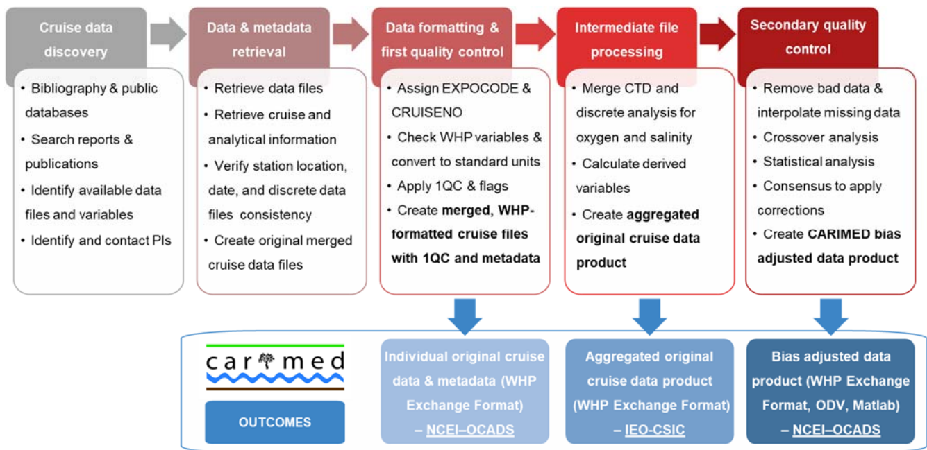
Figure 1: Summary of the CARIMED workflow, from cruise data discovery to the generation of the final data synthesis products. The workflow includes five main stages (shaded blocks) and results in three complementary outputs: individual cruise files with primary (first-level) quality control (1QC), an aggregated original data product (before bias adjustment), and the final CARIMED bias-adjusted data synthesis product (bias-adjusted after secondary quality control). All files are available in WHP (World Ocean Circulation Experiment, WOCE, Hydrographic Program) Exchange format. NCEI-OCADS and IEO-CSIC correspond to the National Oceanic and Atmospheric Administration National Center for Environmental Information - Ocean Carbon and Acidification Data System and the Spanish Institute of Oceanography-Agencia Consejo Superior de Investigaciones Científicas data repositories).
