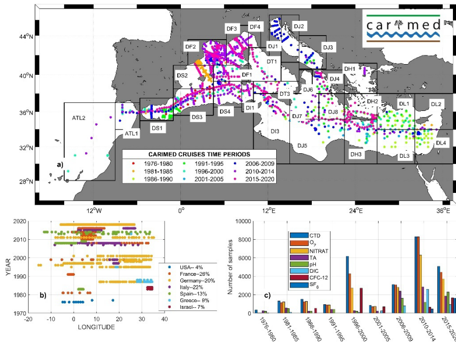
Figure 1: Overview of the cruises included in the CARIMED data synthesis products: (a) map showing the cruise stations included in CARIMED grouped by five year-periods with measurements; (b) spatiotemporal distribution of stations (year vs. longitude), coloured by Chief Scientist country, with the legend indicating the percentage of cruises per country; (c) histogram of the number of samples per variable, grouped into five-year periods, with variables categorised as CTD (thermohaline variables), dissolved oxygen (O 2 ), dissolved inorganic nutrients represented with nitrate (NITRAT), total alkalinity (TA), pH, total dissolved inorganic carbon (DIC), and transient tracers (CFC-12, and SF 6 ). Regional areas according to Manca et al. (2004) are depicted in Fig. 1a. See Table 2 for more information.
