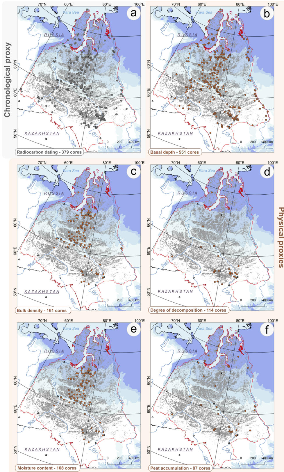
760 Figure B1. Spatial distribution of peat cores included in the Western Siberian Peat Core Database with records of proxies: (a) radiocarbon dating, (b) basal depth, (c) bulk density, (d) degree of decomposition, (e) moisture content, (f) peat accumulation, (g) peat humification, (h) plant macrofossils, (i) pollen, (j) macrocharcoal, (k) testate amoebae, (l) microcharcoal, (m) non-pollen palynomorphs, (n) diatoms, (o) oribatid, (p) arthropod peat humification, (q) mollusc, (r) zoogenic remains, (s) carbon accumulation, (t) ash content, (u) organic matter, (v) geochemistry, (w) pH, (x) stable isotopes, (y) XRF (X-ray fluorescence)/XRD (X-ray diffraction), (z) FTIR (Fourier transform infrared spectroscopy).
