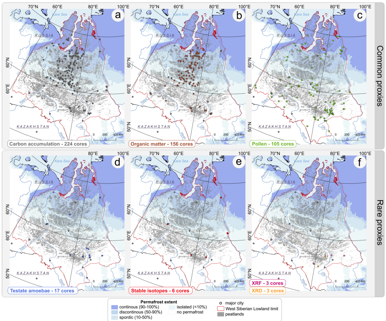
445 Figure 7. Spatial distribution of peat cores included in the Western Siberian Peat Core Database with records of selected proxies. Commonly used palaeoecological proxies are shown in panels a-c (a – carbon accumulation; b – organic matter; c – pollen), while rarely applied proxies are presented in panels d-f (d – testate amoebae; e – stable isotopes; f – XRF/XRD). Numbers indicate the total count of cores containing each proxy. Maps include peatlands extent based on Sheng et al. (2004) and permafrost extent based on Brown et al. (2002). Abbreviations: XRF – X-ray fluorescence; XRD – X-ray diffraction.
