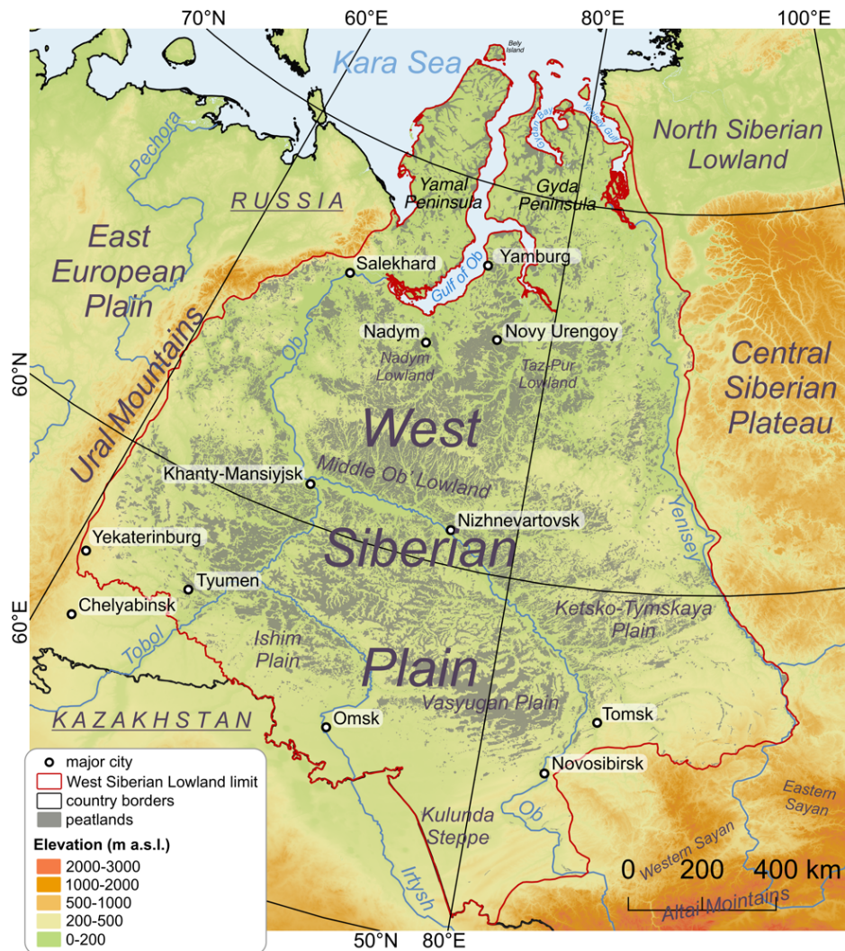
Figure 1. Topographic map of Western Siberian Lowland with the extent of peatlands based on Sheng et al (2004), main rivers, selected cities, and main geographic units and geographical extent of study area considered in this literature review. Elevation source: © DLR e.V. 2010-2014 and © Airbus Defence and Space GmbH 2014-2018 provided under COPERNICUS by the European Union and ESA; all rights reserved.
