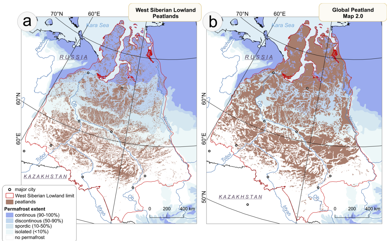
170 Figure 2. Spatial distribution of peatlands in the Western Siberian Lowland: (a) regional map by Sheng et al. (2004) with peat depth threshold >50 cm; (b) Global Peatland Map 2.0 (Greifswald Mire Centre, 2022) with peat depth threshold ≥10 cm.
