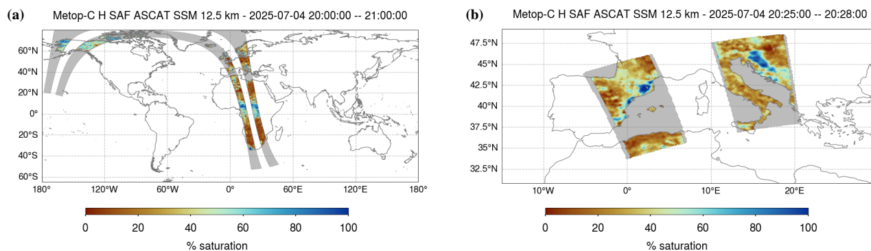
Figure 8. Example H SAF ASCAT SSM swath for a 60-minute (a) and 3-minute (b) interval. ASCAT SSM data © EUMETSAT.
