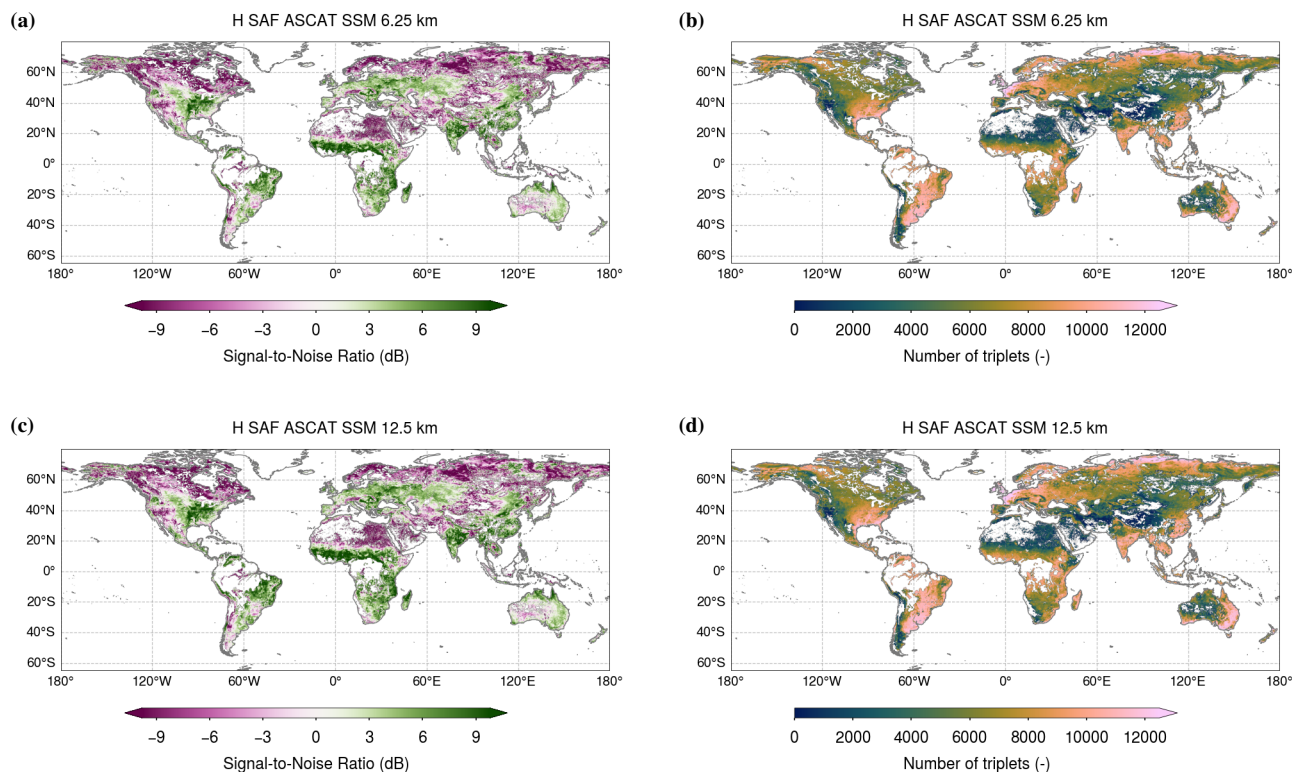
Figure 13. Global maps of SNR (a) and the number of triplets (b) between H SAF ASCAT SSM 6.25 km, Noah GLDAS-2.1 and ESA CCI Passive SM are shown in the top half, while corresponding maps for H SAF ASCAT SSM 12.5 km (c, d) are presented in the bottom half. H SAF ASCAT SSM data © EUMETSAT. GLDAS-2.1 (Noah) data © NASA. ESA CCI Passive Soil Moisture data © ESA.
