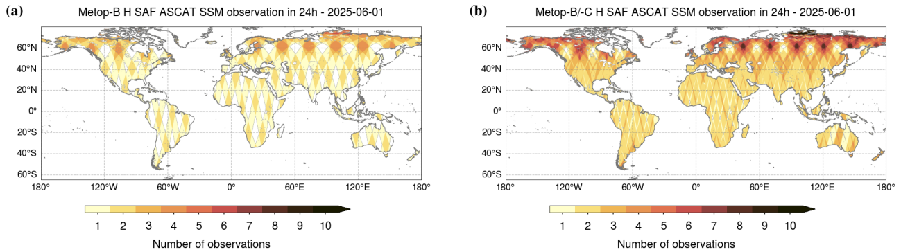
Figure 9. ASCAT observations recorded within a 24-hour period over land: (a) Metop-B only, (b) combined Metop-B and Metop-C data. ASCAT SSM data © EUMETSAT.
