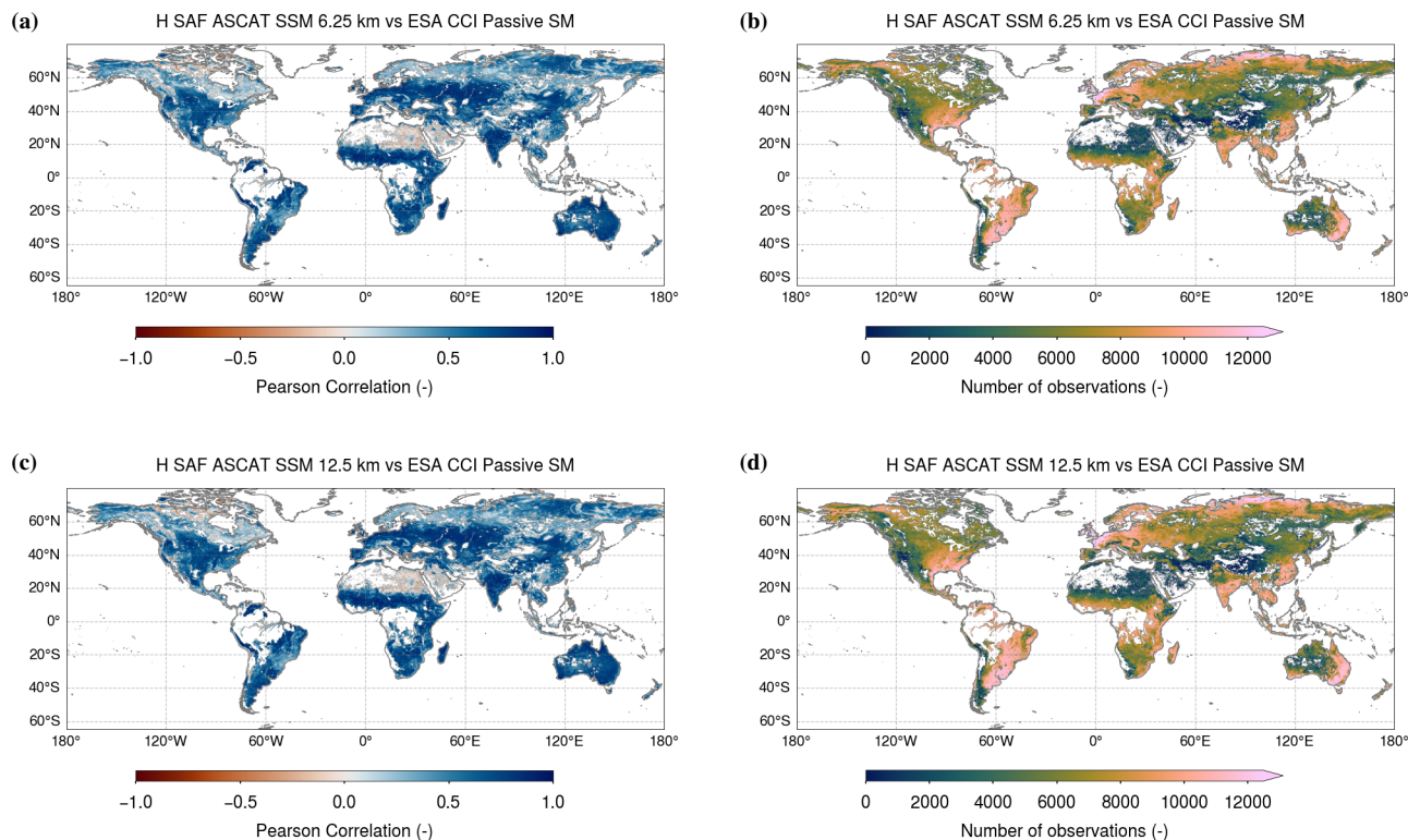
Figure 11. Global maps of the Pearson correlation coefficient (a) and the number of observation pairs (b) between ASCAT SSM at 6.25 km and ESA CCI Passive SM are shown in the top half, while corresponding maps for ASCAT SSM at 12.5 km (c, d) are presented in the bottom half. ASCAT SSM data © EUMETSAT. ESA CCI Passive Soil Moisture data © ESA.
