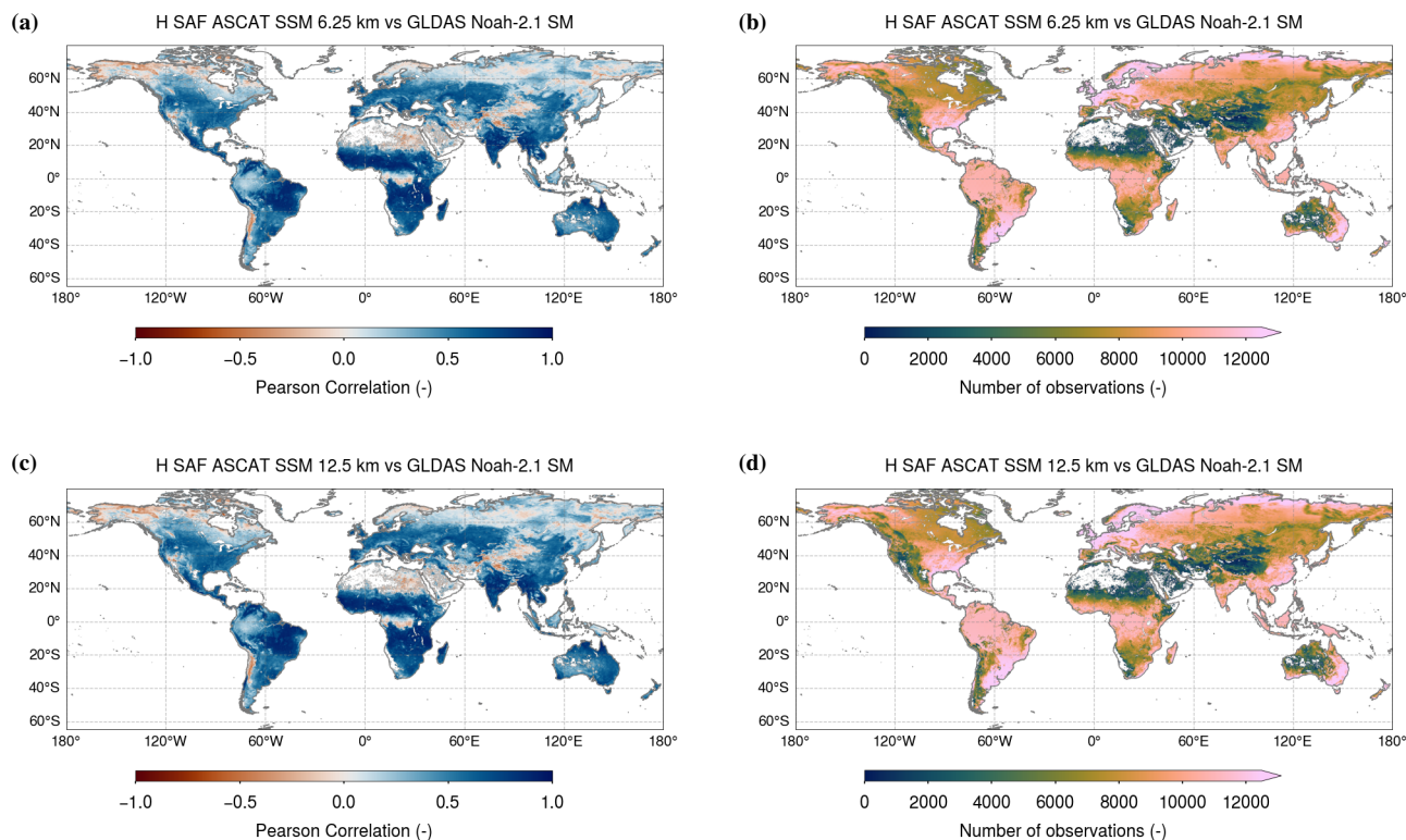
Figure 12. Global maps of the Pearson correlation coefficient (a) and the number of observation pairs (b) between ASCAT SSM at 6.25 km and Noah GLDAS-2.1 are shown in the top half, while corresponding maps for ASCAT SSM at 12.5 km (c, d) are presented in the bottom half. ASCAT SSM data © EUMETSAT. GLDAS-2.1 (Noah) data © NASA.
