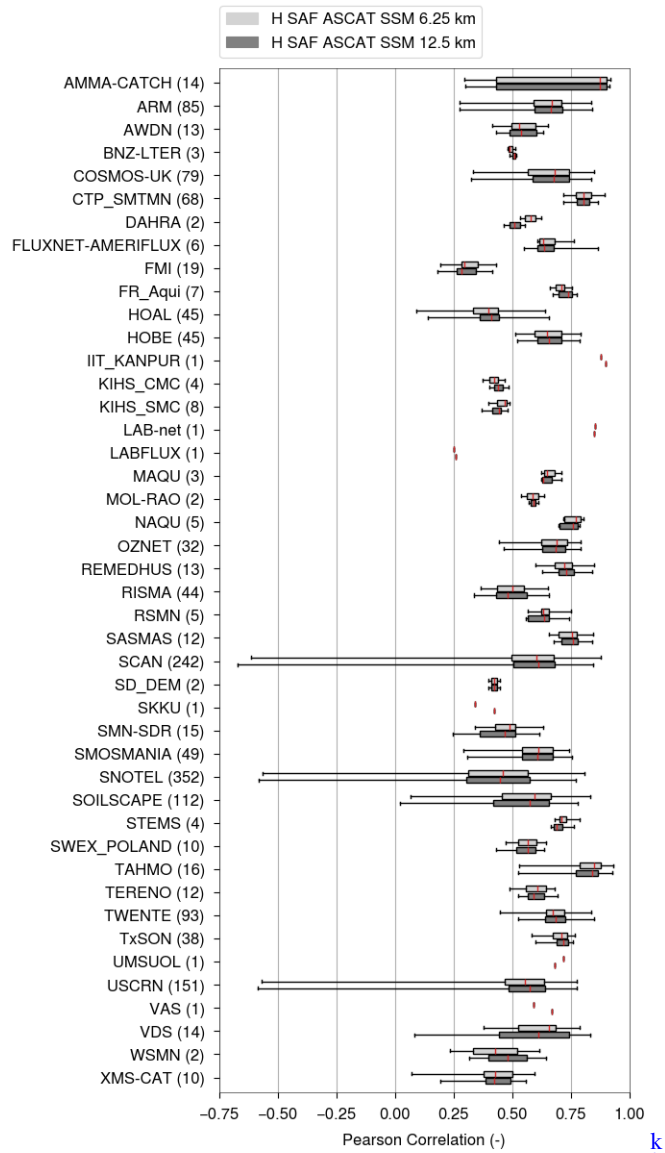
Figure 15. Pearson correlation coefficient (R) computed between H SAF ASCAT SSM (6.25 km and 12.5 km) and 44 ISMN in-situ networks. The evaluation was performed on data ranging from January 2007 to December 2024. The boxplots depict the distribution of Pearson R for each network, with the number of sensors next to the network name. Whiskers extend to the 2nd and 98th percentiles of the Pearson R distribution per network.
