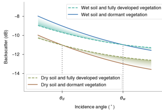
Figure 4. Cross-over angle A visualization of the cross-over concept: Backscatter-incidence angle curves for constant soil moisture and varying vegetation intersect at characteristic angles where the influence of vegetation on backscatter is minimized. These angles, called the dry and wet cross-over angles, are chosen to minimize the effect of vegetation during the estimation of the dry and wet backscatter reference.
