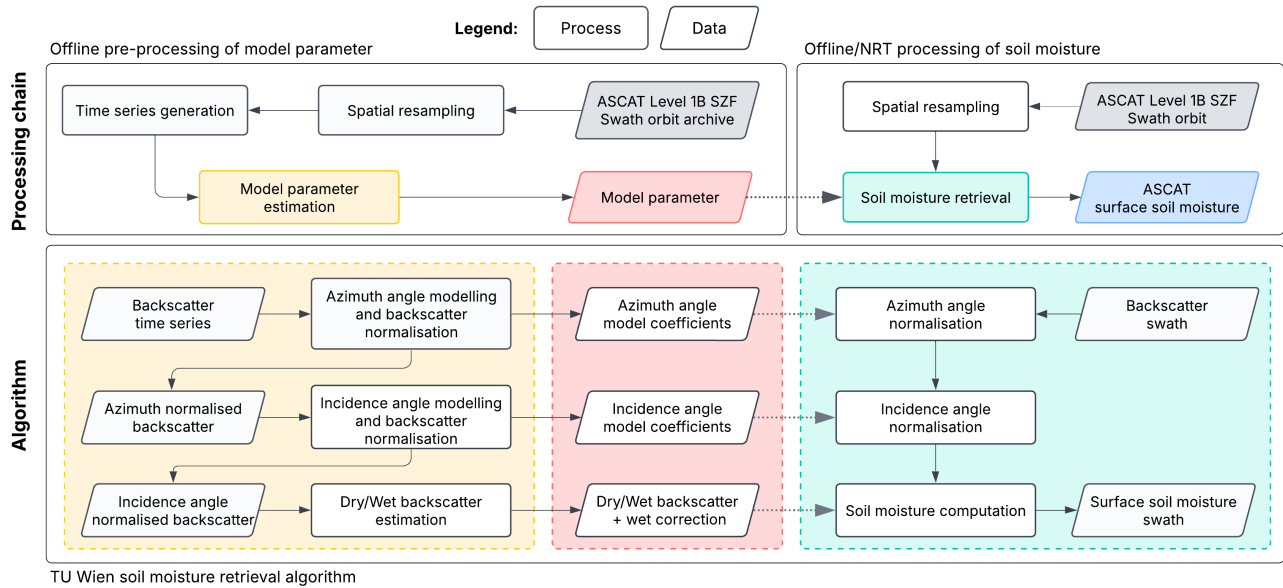
Figure 1. Processing workflow showing (i) the estimation Overview of the semi-empirical processing workflows and retrieval algorithm. The upper flowchart illustrates the offline model parameter pre-processing steps and the retrieval of offline/NRT surface soil moisture using processing chain. The lower flowchart provides a detailed summary of the TU Wien change detection soil moisture retrieval algorithm, and (iii) validation as part of the post-processing.
