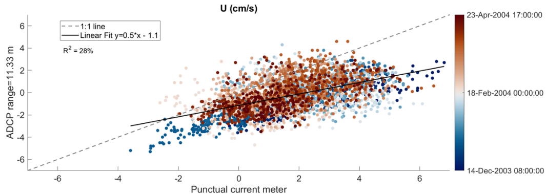
Figure 3: Comparison of the eastward velocity component (U) velocity components from punctual current meter (located approximately 1 m above the seabed) and ADCP (data refers to measurements taken at 11.33 m above the seabed) at GEOSTAR-SN3 (2003–2004). To match these two different types of data we considered the hourly time series.
