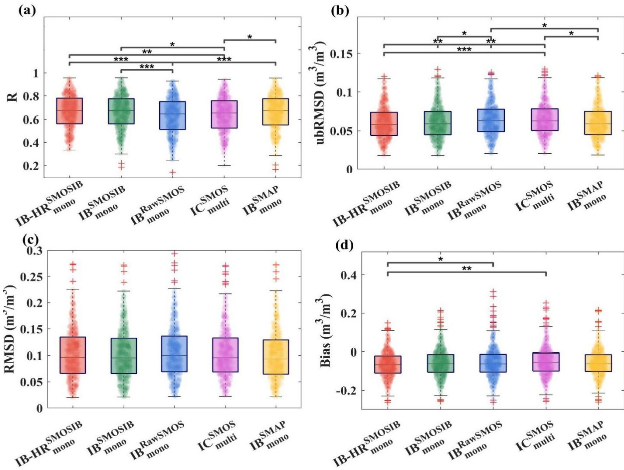
Figure 5: Boxplots summarizing the overall metrics of IB_{HR_{mono}}^{SMOSIB} , IB_{mono}^{SMOSIB} , IB_{mono}^{RawSMOS} , IC_{multi}^{SMOS} , and IB_{mono}^{SMAP} against ISMN in-situ SM regarding (a) R , (b) ubRMSD ( m^3/m^3 ), (c) RMSD ( m^3/m^3 ) and (d) Bias ( m^3/m^3 ) from 2016 to 2022. The scatter points in the boxplot represent individual data points. The symbols *, **, and *** indicate that the P -Value computed from the two-sample t -test between the metrics of each two products is below 0.05, 0.01, and 0.001, respectively.
