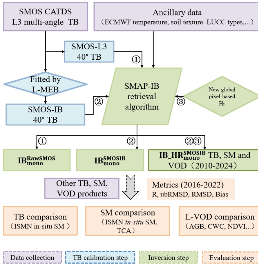
225 Figure 2: Flow chart illustrating the workflow from data production and performance assessment of ① IB_{mono}^{RawSMOS} , ② IB_{mono}^{SMOSIB} and ③ IB_{mono}^{SMOSIB} TB, SM and VOD (2010-2024): inputs (purple), SMOS-IB TB calibration (blue), SM and VOD inversion (green) and performance assessment (orange).
