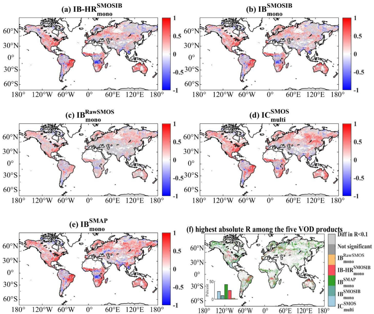
525 Figure 9: Temporal correlation between VOD and CWC (2016–2022) for (a) IB_{HR}^{SMOSIB}_{mono} , (b) IB_{mono}^{SMOSIB} , (c) IB_{mono}^{RawSMOS} , (d) IC_{multi}^{SMOS} and (e) IB_{mono}^{SMAP} . (f) maps of the above five VOD products with the highest absolute R values with CWC. Non-significant R are represented by dark grey pixels ( p > 0.05 ), and the light grey color indicates pixels with R difference for each paired VOD product < 0.1 . White areas represent “no valid data”.
