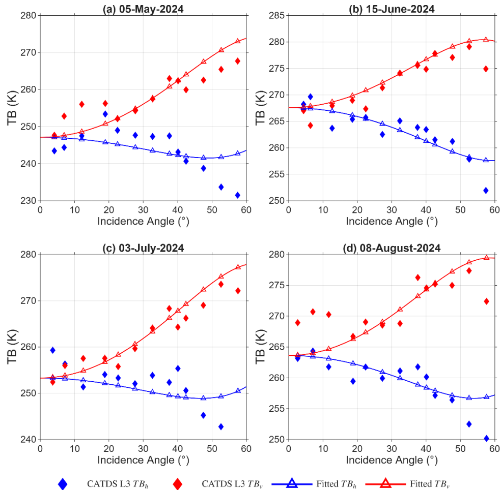
240 Figure 3: Examples of L-MEB model fitting to CATDS L3 TB at a SMOS pixel located at 83.646°E, 31.661°N. Panels (a) – (d) correspond to May 5, June 15, July 3, and August 8, 2024, respectively.
