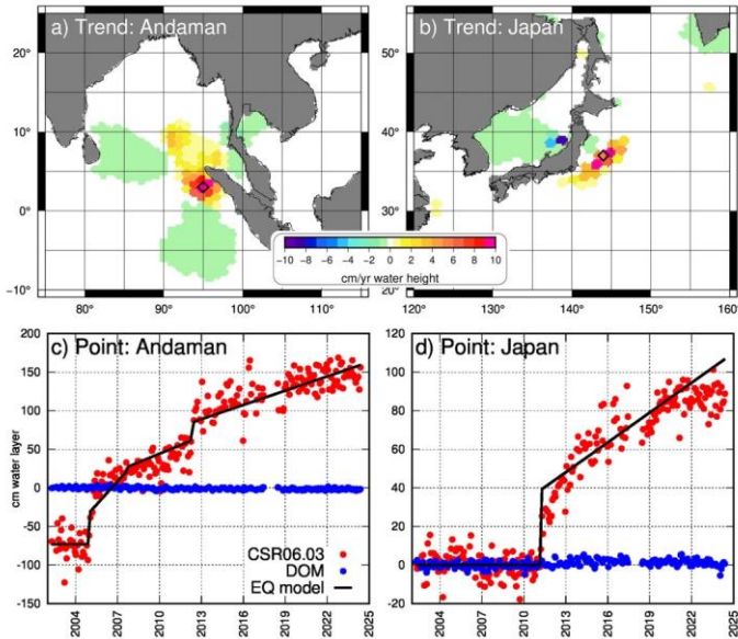
375 Figure 5: 2002-2025 Trend of CSR RL06.3 standard mascon series near (a) Andaman Bay and (b) Japan, plus timeseries (c, d) of a single mascon near each epicenter (locations shown as diamonds in a, b) for both CSR RL06.3 (red) and the DO mascons (blue). Timeseries of the earthquake model at the observed points is shown as the black line. (Global ocean means have been removed from RL06.3 each month, to approximate the removal of the GRD signal.)
