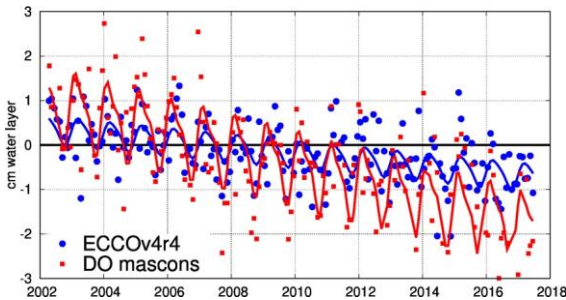
5420 Figure 10: Average mass change (in terms of water height) in the region of the northeastern Atlantic drawn in Figure 9.
