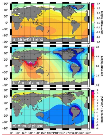
Figure B2: The linear trend (a), annual amplitude (b), and annual phase (c) of the GravIS barystatic-GRD estimate. The ocean mask used was the CSR mascon mask (to 1° resolution). Phases in (c) are defined such that 0 refers to an annual maximum in January, and \pm 6 refers to a maximum in July.
