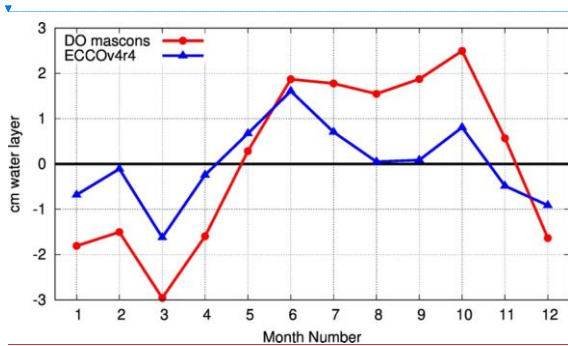
5495 Figure 12: Differences in monthly climatology of average within 5° longitude of the north pole.
