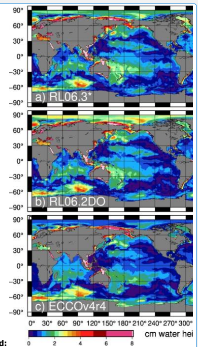
Deleted: Figure 10: 2002-2017 annual amplitudes from (a) CSR RL06.3 mascons after a uniform global ocean average is removed each month, (b) the DO mascons, and (c) the ECCOv4r4 model.¶ Deleted: 121112 Deleted: ¶
