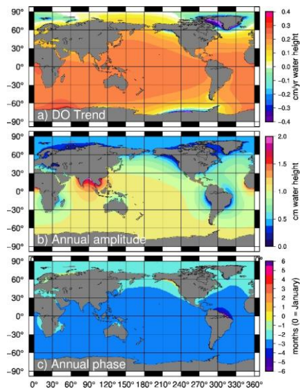
7005 Figure B3: The linear trend (a), annual amplitude (b), and annual phase (c) of the DO mascon barystatic-GRD estimate. The trend and annual amplitude are identical to those shown in Fig. 7, and are repeated here for ease of comparison. Phases in (c) are defined such that 0 refers to an annual maximum in January, and \pm 6 refers to a maximum in July.
