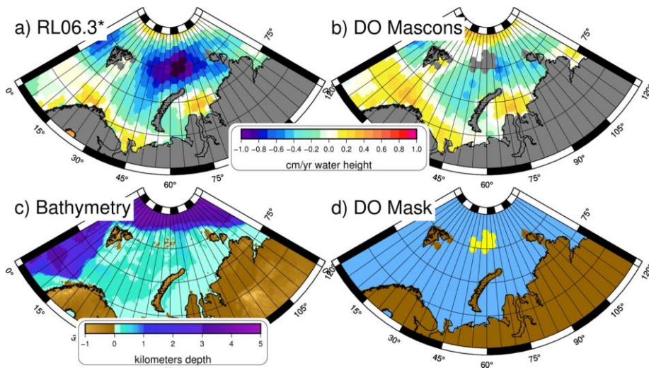
335 Figure 3: Trends of (a) the CSR RL06.3 mascons, after an appropriate GRD series and GAD_{avg} have been removed, and (b) the DO mascons. The ETOPO1 bathymetry (c) shows the location of Franz Josef Land, which is masked as “land” (yellow) in the DO mascons (d).
