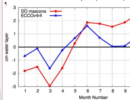
Figure 12: Differences in monthly climatology of average within 5° longitude of the north pole.¶
