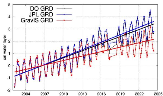
7010 Figure B4: The mean signal over the global oceans (as defined by the CSR mascon mask), for the barystatic-GRD estimates from the new DO mascons, the JPL mascons, and the COST-G GravIS spherical harmonics.
