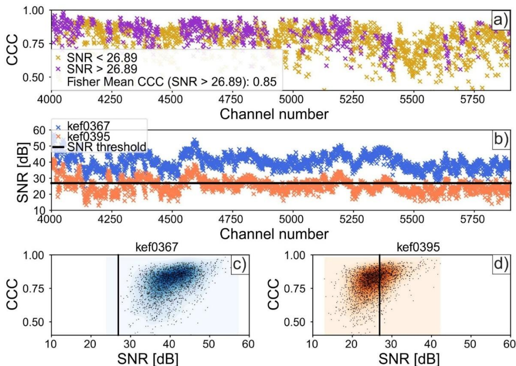
Figure 7. Waveform Crosscross-Correlation-correlation Coefficient-coefficient (CCC) analysis for event pair kef0367 ( M_L 1.76) and kef0395 ( M_L 10.09). (a) CCC of individual DAS traces from channels 4000-5900. (a) Purple and gold symbols are CCC values above and below a SNR threshold calculated from the smaller amplitude event in the pair (see text and description in panel b of this figure). (b) Signal-to-noise ratio (SNR) of each event in the pair. SNR (in dB) is calculated as the ratio between the root-mean-square of the signal in 4-second windows starting 0.5 s after the detection time and noise windows of the same length starting 5 s before the detection time (refer to Fig. 3a for SNR windows). The thick horizontal black line marks the minimum SNR threshold required for the CCC calculation, which is defined by the lower-amplitude event. The threshold corresponds to the cutoff of the top 33% of channels with the highest SNR. (c–d) CCC versus SNR for events kef0367 and kef0395. The vertical black line indicates the minimum SNR threshold. Average CCC cross-correlation-coefficient of the event pair is 0.85, estimated as the Fisher mean of the individual CCC values. Traces are band-pass-filtered 5-20 Hz. The correlation between SNR and CCC at individual traces is even clearer when showing CCC values over the entire cable (Fig. S10).
