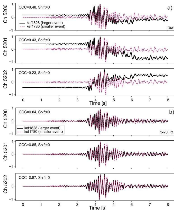
Figure 11. Waveforms of similar events (average CCC = 0.7 from DAS), one of which is affected by cycle skipping. The M_L 2.8–7 event kef1828 (black) shows waveform distortion at the S-wave arrival, while the M_L 1.4 event kef1780 (violet) does not. (a) Raw waveforms. (b) Band-pass filtered waveforms (5–20 Hz). Hypocentral locations: kef1780 – 38.4018°N, 20.4502°E, depth 3.41 km; kef1828 – 38.4018°N, 20.4547°E, depth 3.76 km. Note the high waveform similarity after filtering the traces. The events show an average CCC of 0.7 at seismic stations (Fig. S13S14)
