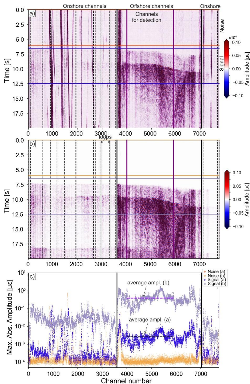
Figure 2. (a) Example of earthquakes recorded along the cable. (a) M_L 0.6 on 08 August 2024 at 10:35 UTC (NOA event-id: noa2024pmvwc). (b) M_L 3.0 Earthquake on 08 August 2024 at 19:18 UTC (NOA event-id: noa2024pnndk). (c) Maximum absolute amplitudes of signal and noise shown in panels (a-b). (c) Horizontal dashed black and purple lines indicate average amplitudes for events displayed in panel a and b, respectively. The length of the horizontal lines shows the range of channels used for calculating the average amplitudes (4000-5900). Panels (a-b) detail the location of onshore and offshore channels, the location of the channels used for the detection, and the location of the identified loops. Traces are band-pass filtered 53-30-20 Hz. The light and dark orange, and violet and blue lines in panels (a-b) highlight the noise and signal windows shown in panel (c). -
