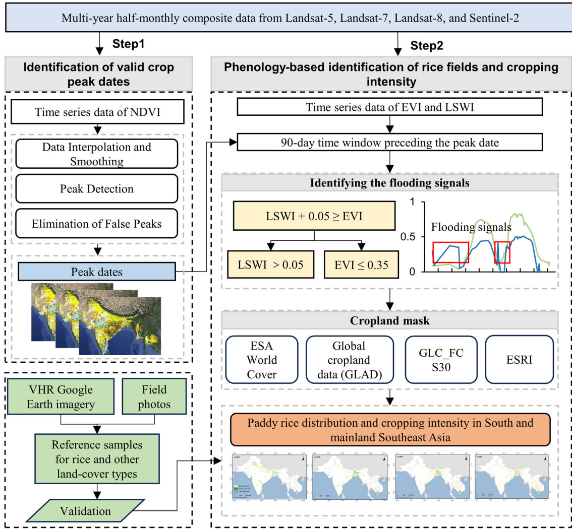
Fig. 2. Flowchart of the mapping process for long-term rice spatial distribution and cropping intensity in South and mainland Southeast Asia.
