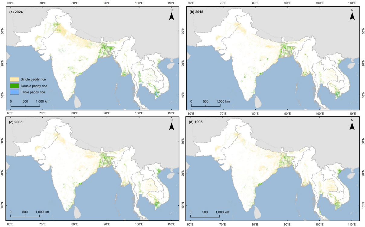
Fig. 3. Multi-year composite rice distribution and cropping-intensity products for South and mainland Southeast Asia, represented by the nominal reference years 1995, 2005, 2015, and 2024.
