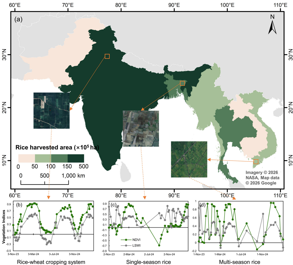
Fig. 1. (a) Spatial distribution of rice harvested area in South and mainland Southeast Asia ( \times 10^5 ha). Insets show example rice fields at the locations marked by orange squares. (b–d) Representative NDVI (green)
