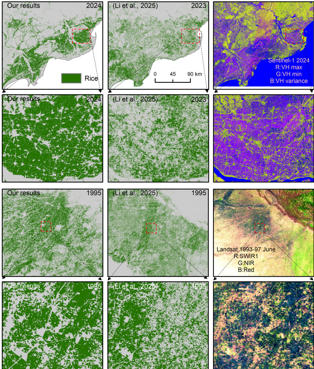
Fig. 5. Comparison of rice distribution maps in South Asia between this study and Li et al. (2025). The comparison includes this study's 2024 and 1995 products, Li et al.'s 2023 and 1995 products, and corresponding Sentinel-1 and Landsat false-color composites.
