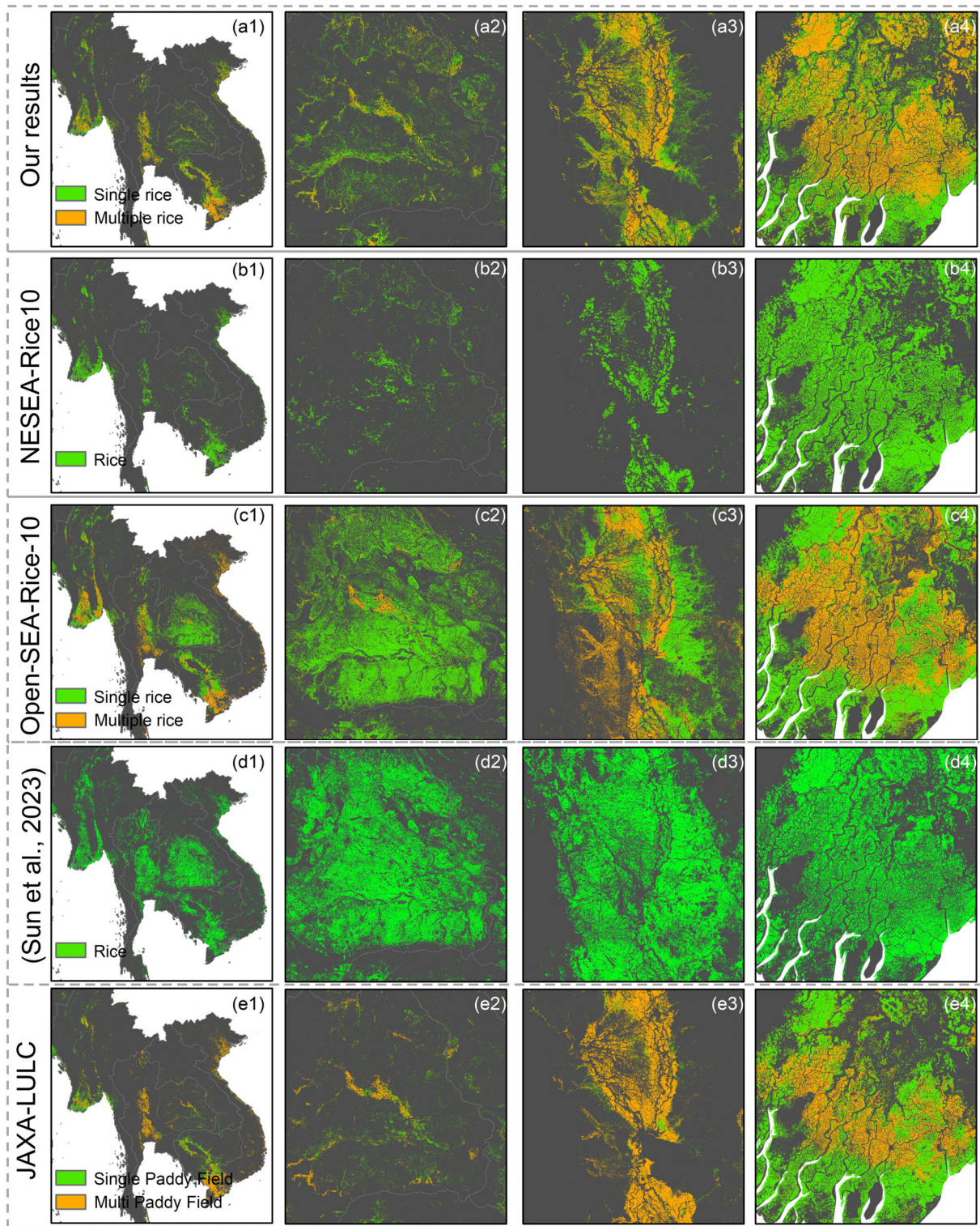
Fig. 6. Comparison of single- and multiple-season rice maps across Southeast Asia. Panels (a1)–(a4) display results from this study, (b1)–(b4) from NESEA-Rice10, (c1)–(c4) from Open-SEA-Rice-10, and (d1)–(d4) from Sun et al. (2023). Panels (e1)–(e4) show JAXA-LULC data, retaining the original land cover classifications of Single Paddy Field and Multi Paddy Field.
