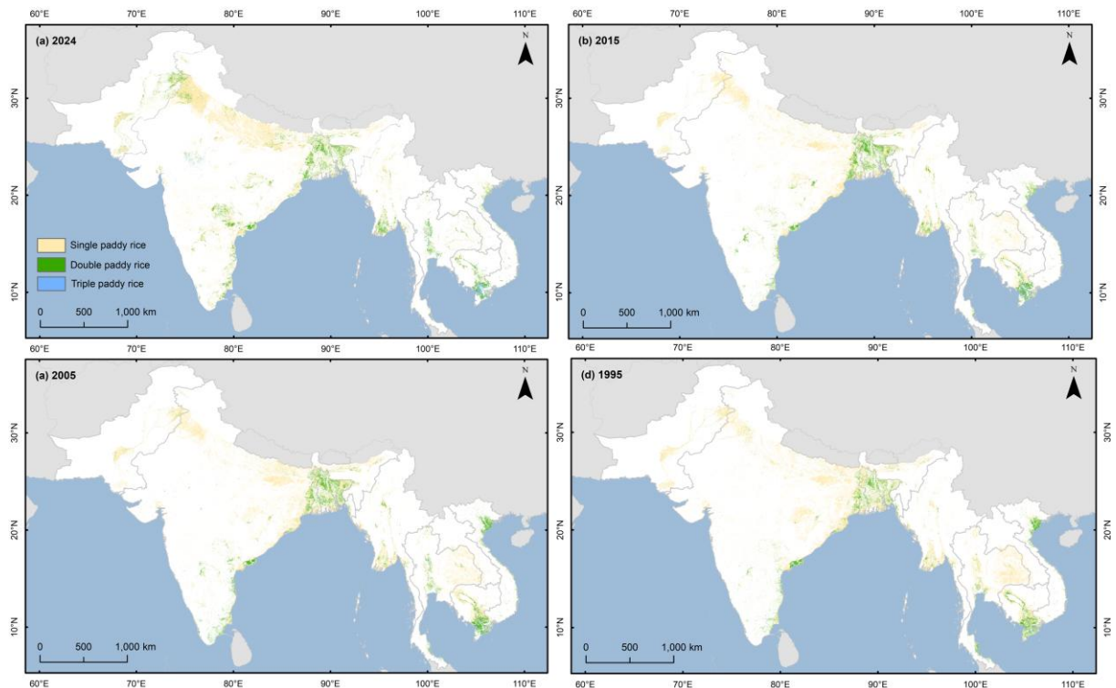
Figure 3. Long-term spatial distribution and planting intensity of rice in South and mainland Southeast Asia (1995, 2005, 2015, 2024)
