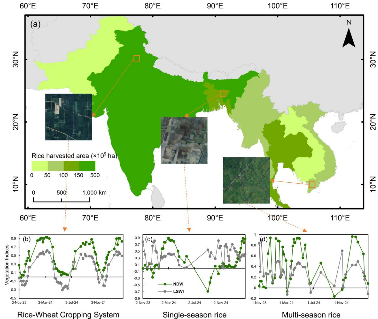
Figure 1. (a) Spatial distribution of rice harvested area in South and Southeast Asia ( \times 10^5 ha). Insets show example rice fields at the locations marked by orange squares. (b–d) Representative NDVI (green) and LSWI (gray) time series for (b) rice-wheat cropping system, (c) single-season rice, and (d) multi-season rice. The locations of the example pixels are indicated by arrows on the map.
