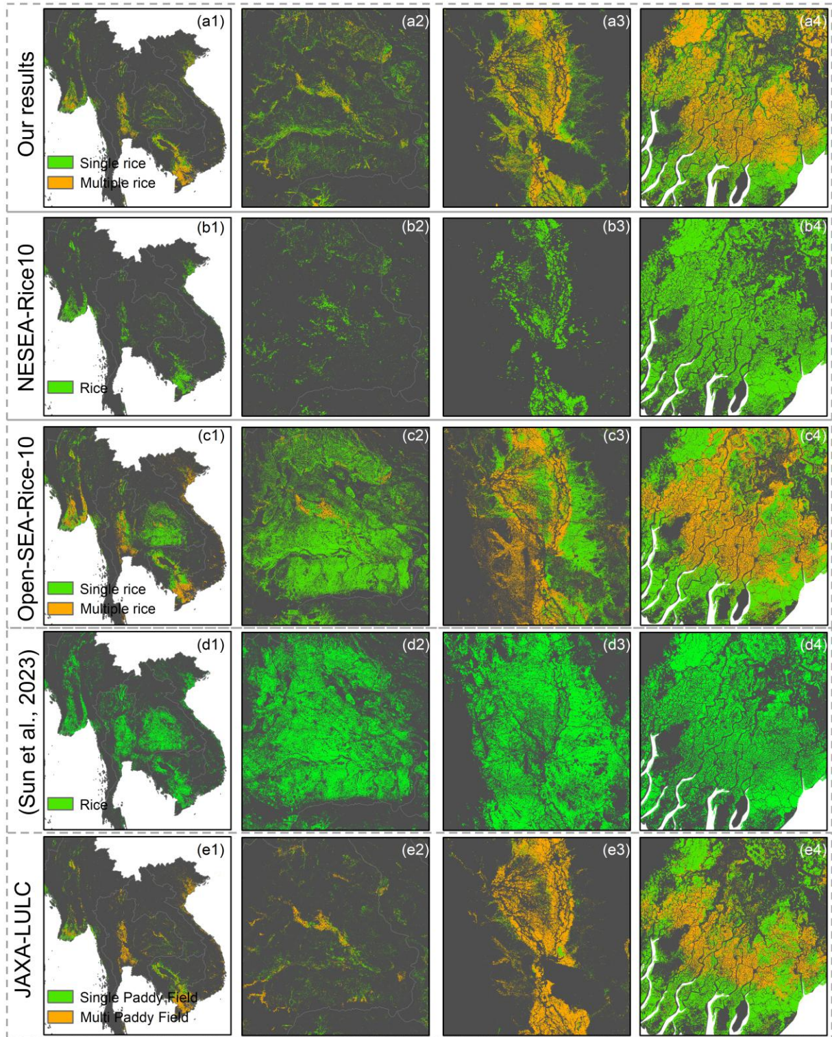
Figure. 6 Comparative analysis of single and multiple rice field Distribution in Southeast Asia. Panels (a1)-(a4) display results from our proposed method, (b1)-(b4) from NESEA-Rice10, (c1)-(c4) from Open-SEA-Rice-10, and (d1)-(d4) from Sun et al. (2023). Panels (e1)-(e4) show JAXA-LULC data, retaining the original land cover classifications of Single Paddy Field and Multi Paddy Field.
