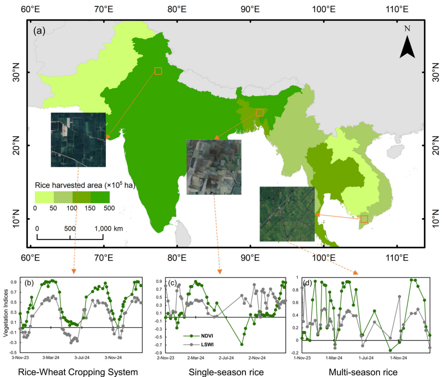
Figure Fig. 1. (a) Spatial distribution of rice harvested area in South and Southeast Asia ( \times 10^5 ha). Insets show example rice fields at the locations marked by orange squares. (b–d) Representative NDVI (green) and LSWI (gray) time series for (b) rice-wheat cropping system, (c) single-season rice, and (d) multi-season rice. The locations of the example pixels are indicated by arrows on the map. The administrative boundaries used in this map are derived from Natural Earth (public domain). They are used solely to delineate the spatial extent of the study areas for this rice mapping research and do not imply any official endorsement or acceptance of national borders. Rice harvested area data were obtained from the Food and Agriculture Organization (FAO). The high-resolution satellite imagery insets were provided by Google Earth.
