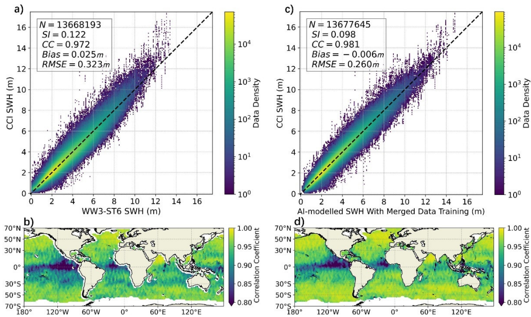
Fig. 8. Comparison between SWHs from numerical/AI wave models and CCI-sea state dataset for global ocean in 2020. (a) Scatter plot of SWHs from the NWM versus CCI-sea state. (b) Spatial distributions of CC between SWHs from NWM and CCI-sea state. (c, d) Same as (a, b), respectively, but for the AI wave model trained with ERA5 and subsequently fine-tuned using the 5-year fused dataset. Note that the year 2020 is excluded from the model training.
