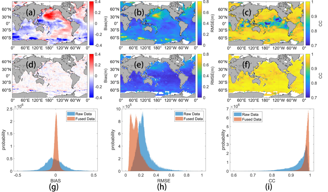
Fig. 6. Comparison between WW3-ST6 (forced by ERA5 winds) and WW3-ST4 (forced by CFSR winds) before and after data fusion is applied to both hindcasts using the same altimeter observations in January 2011. (a–c) Maps of bias, RMSE, and CC between the two hindcasts before data fusion. (d–f) Same as (a–c), but after fusion with altimeter observations. (g–i) Probability density functions of grid-point bias, RMSE, and CC, respectively, illustrating the overall improvement in consistency between the two hindcasts after fusion.
