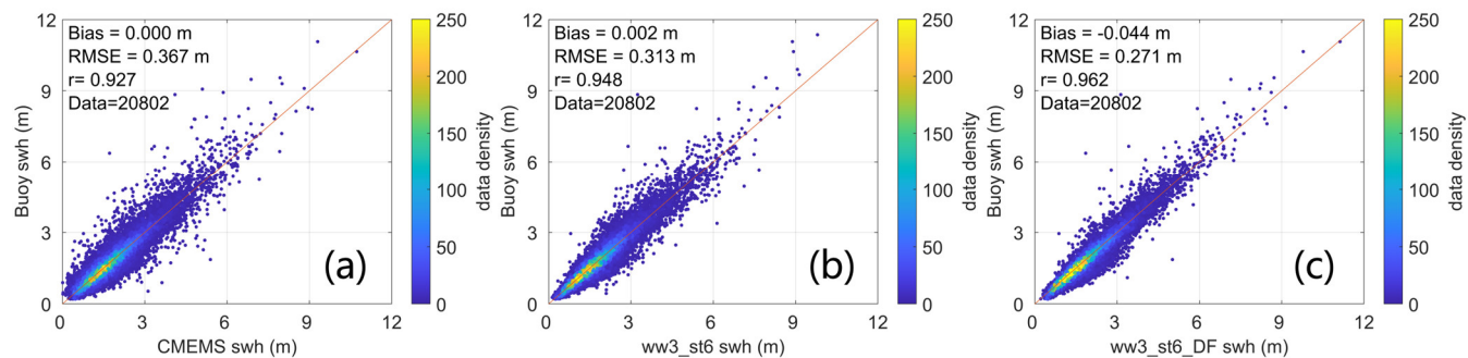
Fig. 2. Scatter plots comparing SWHs from buoy observations with those from (a) the CMEMS (Copernicus Marine Environment Monitoring Service) gridded dataset, (b) the WW3-ST6 dataset, and (c) the fused dataset (“two-sat” version) for instantaneous values at 12:00 UTC during the period 2010–2016. All gridded datasets were bilinearly interpolated to the buoy locations
