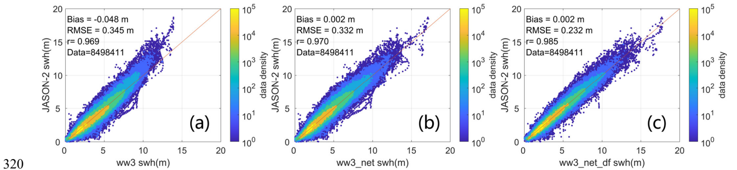
320 Fig. 3. Evaluation of the fused dataset using Jason-2 as an independent reference in 2011. (a) Comparison between the original WW3-ST6 hindcast and Jason-2. (b) Results after applying a one-dimensional look-up table correction to WW3-ST6 SWHs using CCI-Sea State data prior to fusion. (c) Comparison between the fused dataset (WW3-ST6 + remaining altimeters) and Jason-2. The fusion substantially reduces the RMSE and improves the correlation compared to both the original and bias-corrected hindcast.
