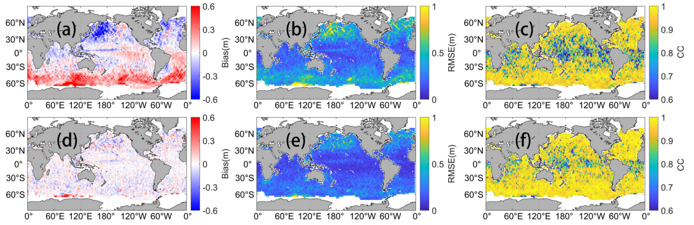
Fig. 4. Spatial distributions of SWH error metrics between WW3-ST6 and Jason-2 (a-c) before and (d-f) after fusing SWH data from CCI-Sea State in 2011: (a & d) bias, (b & e) RMSE, and (c & f) CC.
