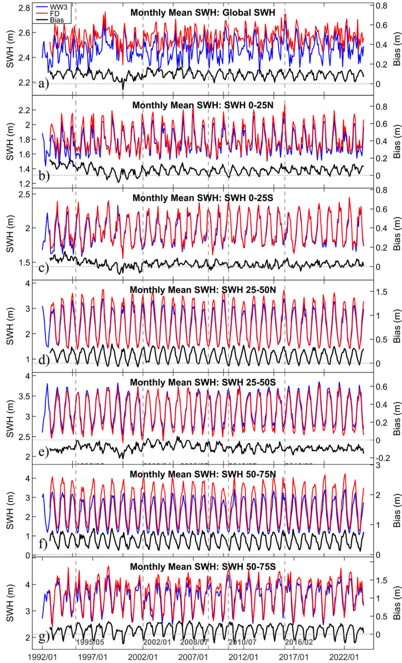
Fig. 5. Time series of monthly mean SWH from the WW3-ST6 hindcast background (blue), the “two-sat” fused dataset (red), and the fused-minus-background difference (black) during 1992–2023: (a) the global ocean, (b) 0–25°N, (c) 0–25°S, (d) 25–50°N, (e) 25–50°S, (f) 50–75°N, and (g) 50–75°S. Vertical dashed lines indicate the major satellite-transition times in the two-satellite configuration, as shown in Table 1.
