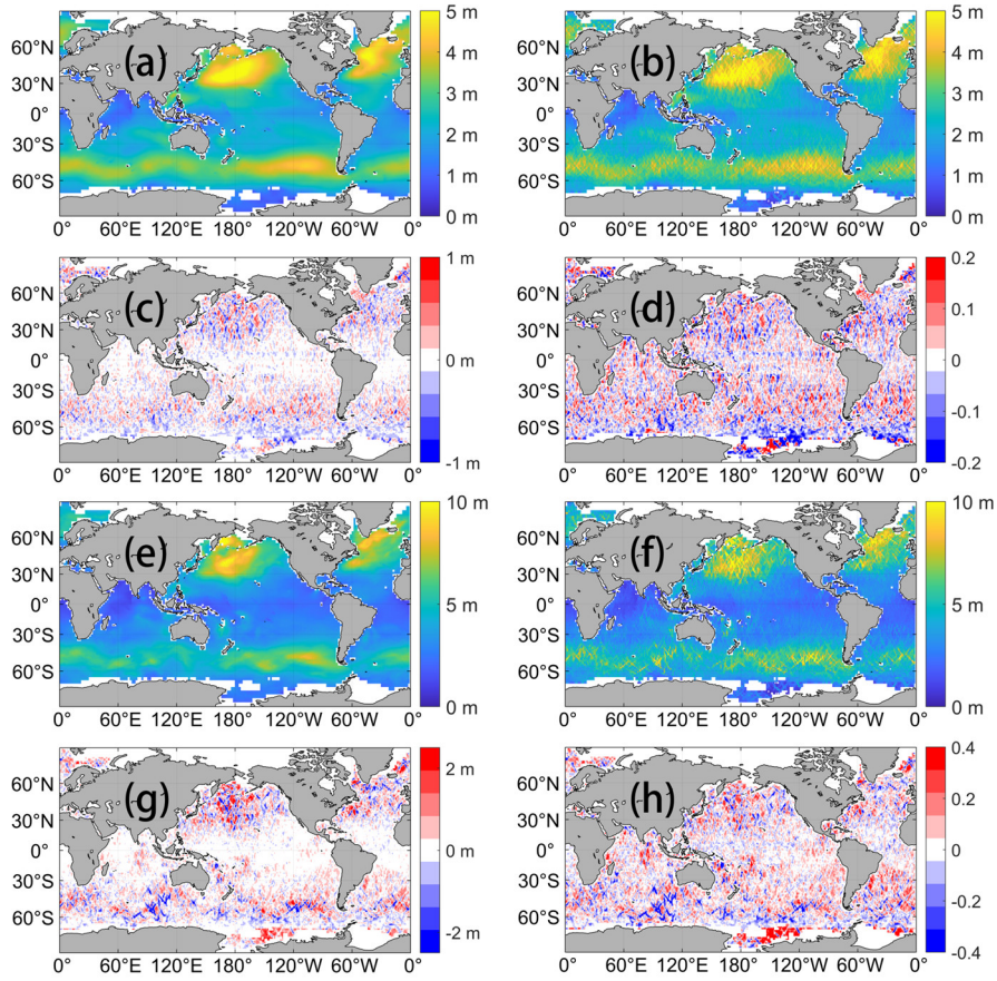
Fig. 7. Global distributions of the monthly mean SWH in January 2011 derived from (a) the fused dataset and (b) the original CCI-Sea State L4 dataset, as well as their (c) absolute difference and (d) relative difference. Panels (e–f) show the corresponding global distributions of the 95th-percentile SWH during the same period derived from (e) the fused dataset and (f) the original CCI-Sea State dataset, as well as their (g) absolute difference and (h) relative difference.
