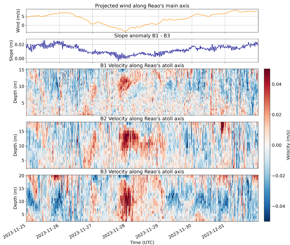
Figure 5: From top to bottom: ERA5 winds (18.5°S, 136.5°W) projected onto Reao's major axis (positive values indicate winds blowing from southeast toward northwest); Time-varying sea surface slope, computed from sea level anomalies between ADCP B1 and ADCP B3; positive values indicate higher water levels at B1 relative to B3; Profiles of projected current velocities along Reao's main axis (positive values indicate currents flowing toward the northwest along the same axis). Note that all variables are expressed as projections onto the atoll's main axis (Figure 3), which is oblique relative to geographic directions; therefore, the color scale represents along-axis flow components rather than strictly zonal or meridional directions
