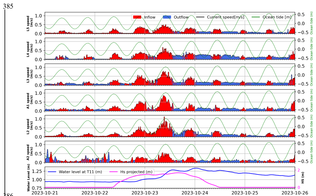
386 Figure 4: Current speed and direction (inflow in red, outflow in blue) recorded by Lowell-TCM4 L2, L3, 387 L4, L5) and Aquadopp (A1, A2) in hoa . Instruments A1 and L3 were positioned a few meters apart within 388 the same hoa . The ocean tide (recomposed from FES2012 global tidal harmonics at 18.75°S, 136.6°W) is shown as solid 389 green lines in each panel. The bottom panel displays the lagoon water level at T11 (blue) and ERA5 projected significant wave height 390 (pink, H_s at 18.75°S, 136.6°W) projected onto the direction normal to the southern rim (210°). 391 392
