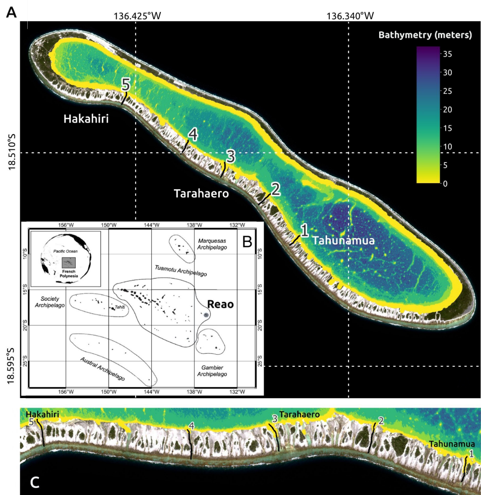
Figure 1: A) Map of Reao (A) with locality of the five main hoo (1-5). Background color refers to satellite-derived bathymetry retrieved from Sentinel-2 imagery (Copernicus Sentinel-2, 2021; Quéré et al., 2025a, 2025b) using the method of Amrari et al. (2021). B) Location of Reao within the French Polynesian archipelagos (Credit: Oriane Bruyère). C) Zoom on the southern rim and its hoo. Numbers indicate the 5 main hoo that were selected for instrumentation, Hoo n°3 (locally called Tarahaero), located
