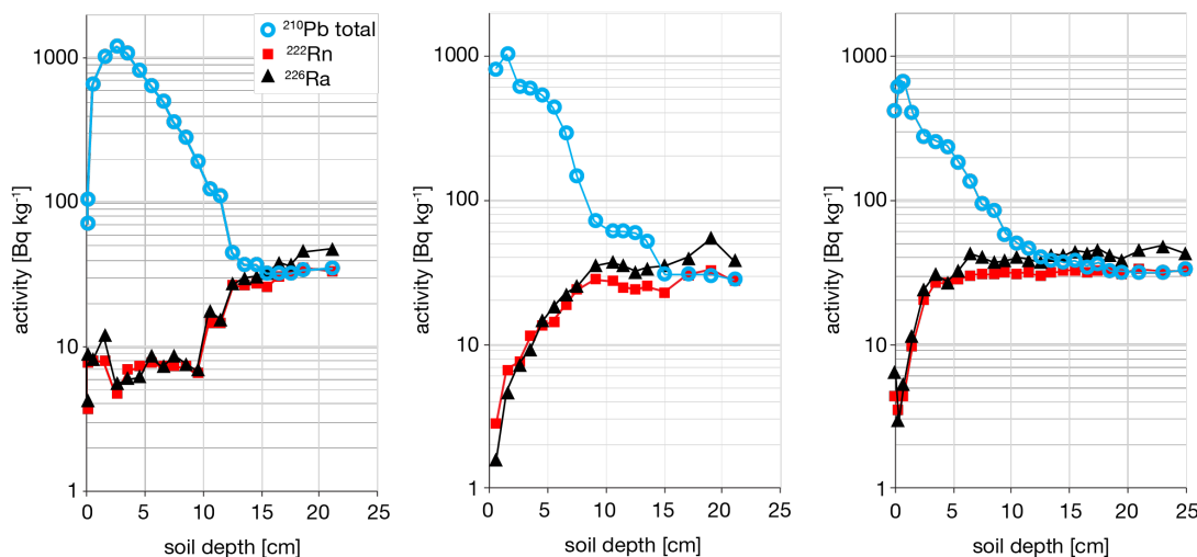
Figure 11. Defining excess ^{210}Pb in soils. (a) Hubbard Brook Experimental Forest (HuB01), (b) Experimental Lakes Area soil 302-1, (c) Harvard Forest LTER (HaF01). Total ^{210}Pb typically converges with ^{222}Rn at depth which indicates that ^{222}Rn is an appropriate estimate of supported ^{210}Pb .
