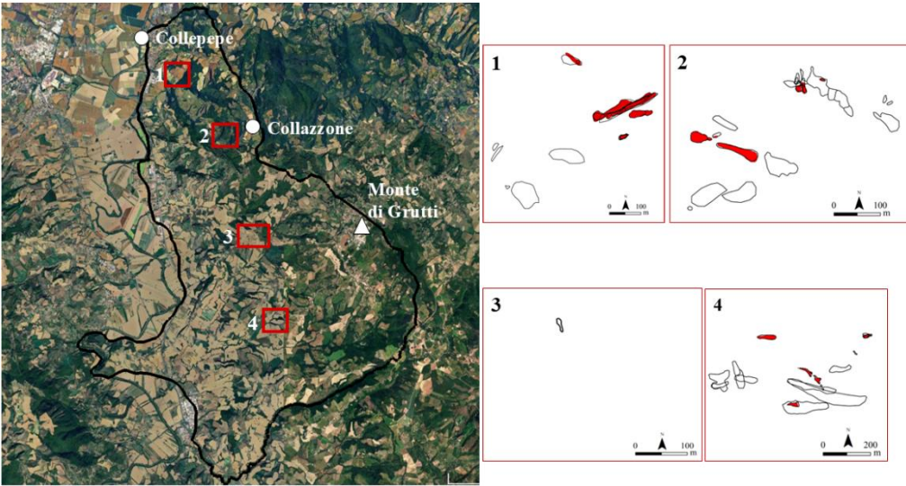
Figure 10: Collazzone study area: localization of the four geographical sectors. Maps data: © Google Earth 2026; images: © 2026 Airbus. An independent geomorphologist investigated the images of different times in the four sectors. In the four sectors black lines show the landslides included in the multi-temporal landslide inventory map. Colored polygons represent the landslides mapped by the external geomorphologist.
