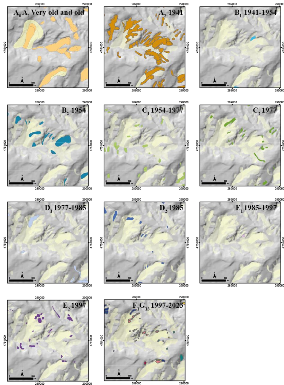
Figure 5: Enlargement of a portion of study area. The letters indicate the layers of the multi-temporal inventory map (table 1 and figure 4). The panels show: A 0 A 1 ) very old and old landslides; A 2 ) fresh landslides in 1941 photographs; B 1 ) landslides occurred between 1941 and 1954; B 2 ) fresh landslides in 1954 photographs; C 1 ) landslides occurred between 1954 and 1977; C 2 ) fresh landslides in 1977 photographs; D 1 ) landslides occurred between 1977 and 1985; D 2 ) fresh landslides in 1985 photographs; E 1 ) landslides occurred between 1985 and 1997; E 2 ) fresh landslides in 1997 photographs and F 1 G 13 landslides occurred from 1997 through 2023.
