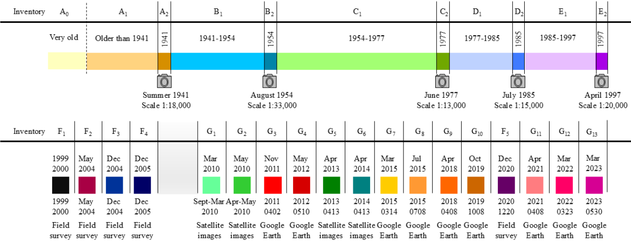
265 Figure 4: Timeline showing the age attributed at the landslide layers. See table 1 for explanation of the layers.
