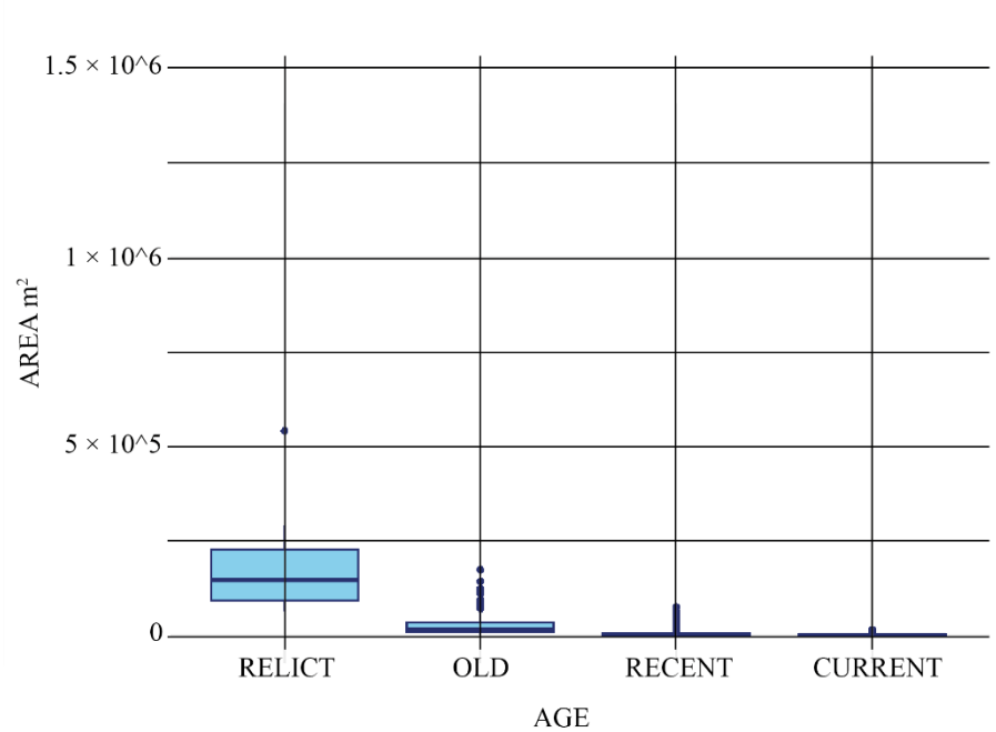
320 Figure 8: Plots summarizing landslide statistics. Landslide area grouped by relative age class (relict; old; recent and current); (b)
