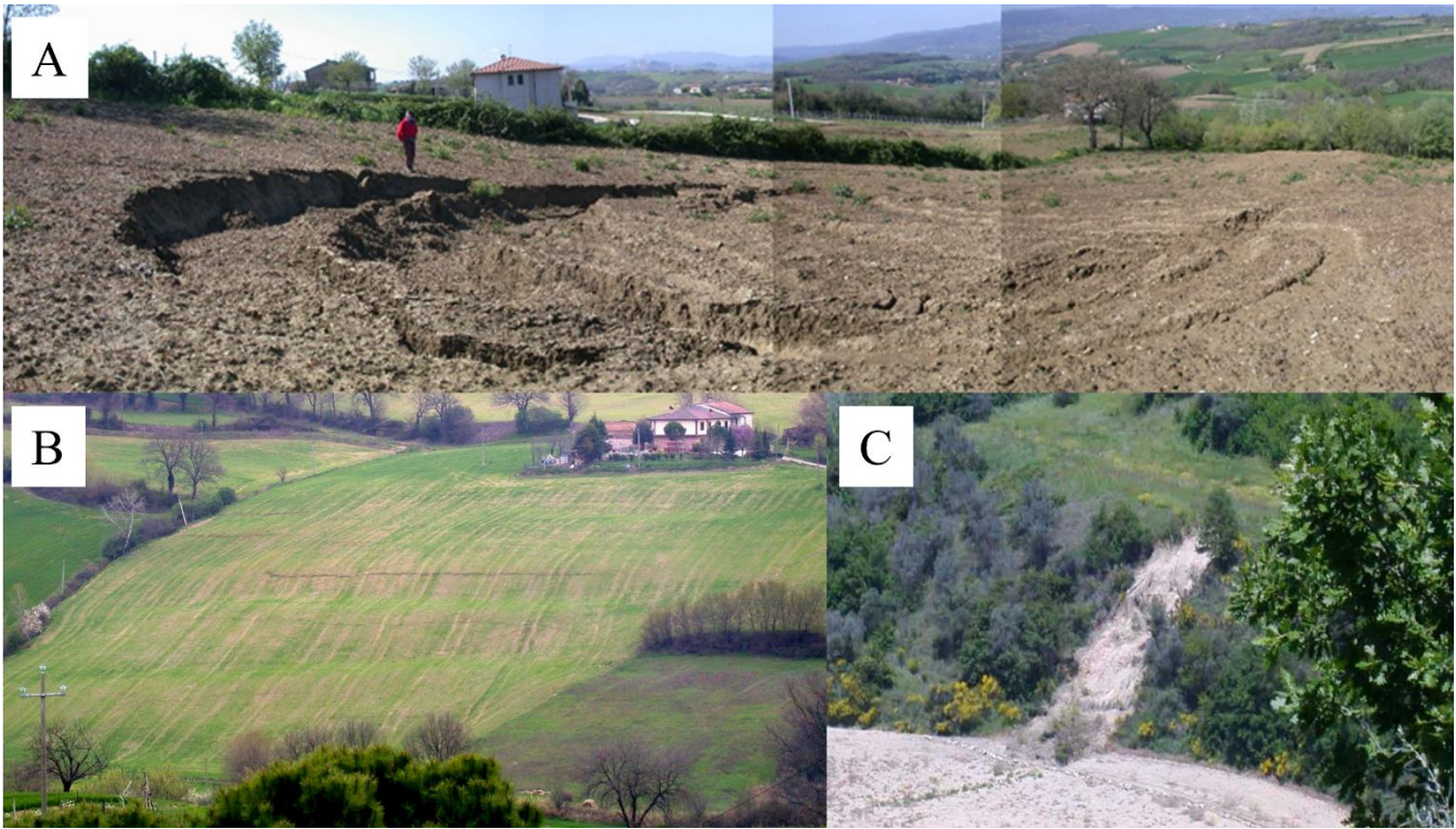
305 Figure 7: Examples of landslide depth. A) deep-seated slide; B) soil slide; C) earth flow. The photographs were taken by the CNR-IRPI.
