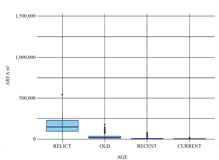
Figure 8: Plots summarizing landslide statistics. Landslide area grouped by relative age class (relict; old; recent and current); (b) Figure 9 shows landslide count (represented by a color gradient and labels) and cumulated area (proportional to circle sizes), grouped by relative age class and landslide type. Visual inspection of the plot reveals that relict and very old landslides are mainly represented by small landslides represented by flows which tend to be small and easily obliterated by erosion and subsequent failures. Further evidence is that a large portion of the total landslide area is occupied by few relict landslides, whereas the smallest landslides correspond to the current period, according to the results by Ardizzone et al. (2023). They suggested that a size threshold effect of previous landslides on subsequent landslides.
