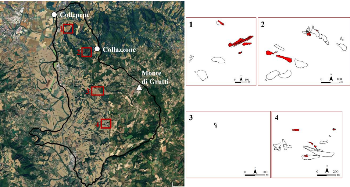
350 Figure 10: Collazzone study area: localization of the four geographical sectors. Maps data: © Google Earth 2026; images: © 2026 Airbus. An independent geomorphologist investigated the images of different times in the four sectors. In the four sectors black lines show the landslides included in the multi-temporal landslide inventory map. Colored polygons represent the landslides mapped by the external geomorphologist.
