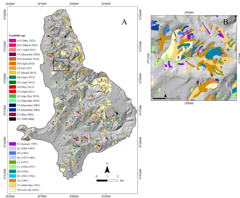
220 Figure 3: Collazzone study area: multi temporal landslide inventory map. The landslides are represented by relative age. The black rectangle (A) shows the location of the enlargement of the map showing the abundance of the landslides over time (B).
