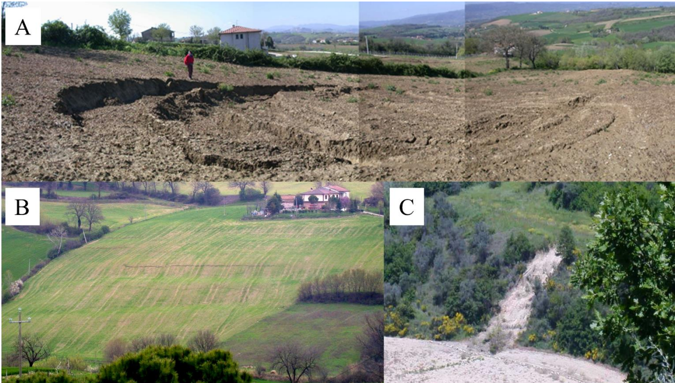
Figure 7: Examples of landslide depth. A) deep-seated slide; B) soil slide; C) earth flow. The photographs were taken by the CNR-IRPI.
