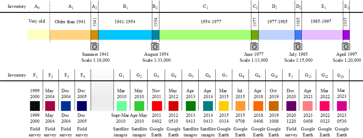
Figure 4: Timeline showing the age attributed at the landslide layers. See table 1 for explanation of the layers.
