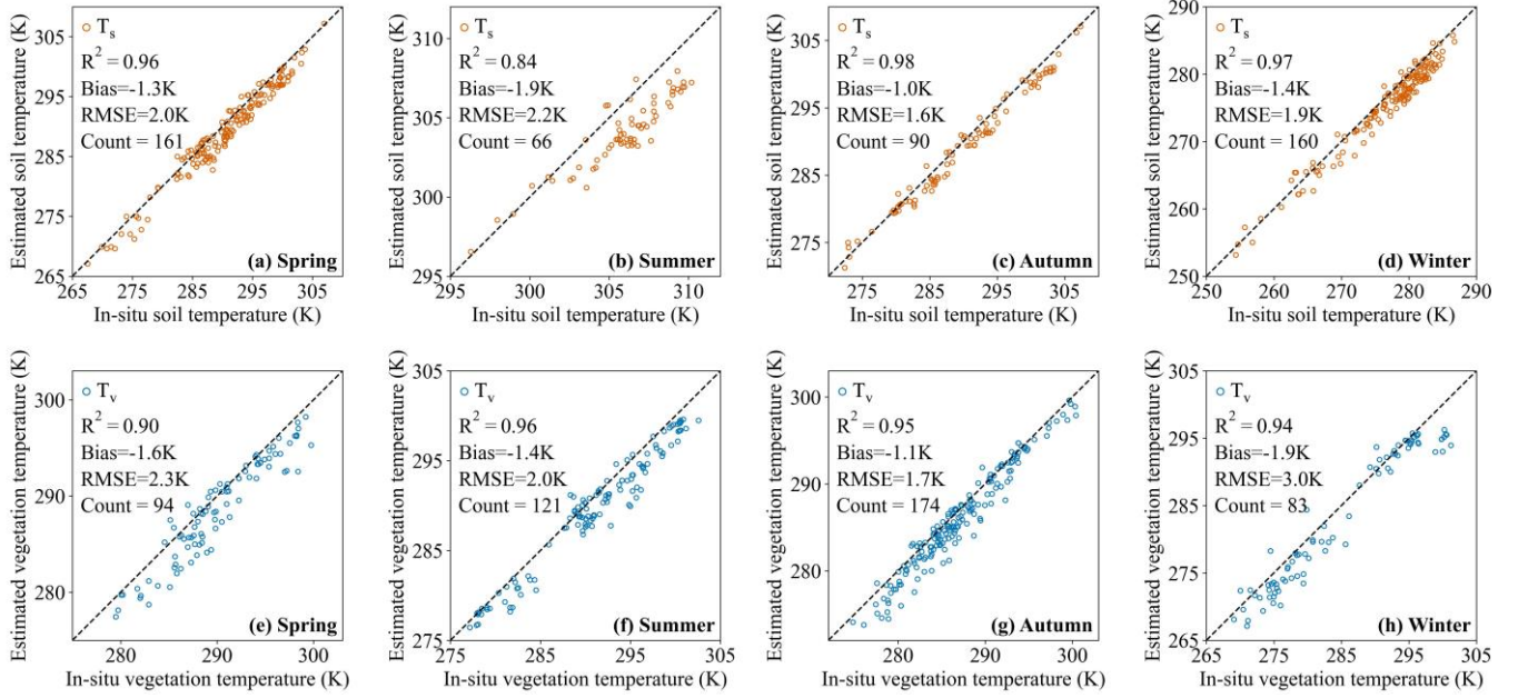
Figure 3: Validation of GloSVeT against in situ measurements across different seasons. Panels (a–d) show soil temperature ( T_s ), and panels (e–h) show vegetation temperature ( T_v ). The dashed line represents the 1:1 reference line. The Count value in each panel denotes the number of matched site-month records, and the corresponding numbers of independent sites for panels (a–h) are 14, 5, 12, 16, 16, 13, 20, and 15, respectively.
