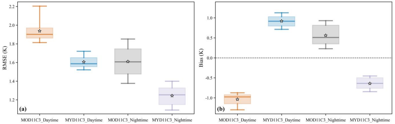
350 Figure 2: Internal closure check of GloSvET. Boxplots show the distributions of monthly global (a) RMSE and (b) Bias between reconstructed mixed-pixel LST and the corresponding original MODIS LST during 2003–2023 at the four MODIS overpass times. Stars denote the mean values, and the dashed line in panel (b) indicates zero Bias.
