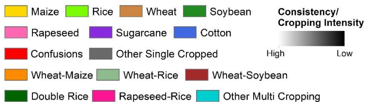
Figure 11. Comparisons of our results and other crop maps (more complex cropping systems) in the year 2020.
