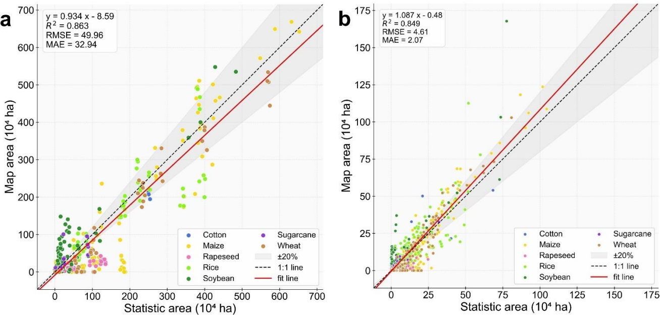
390 Figure 9. Consistency between our crop maps and crop statistics: (a) ADM1 level for 2018–2021, and (b) ADM2 level for 2020.
