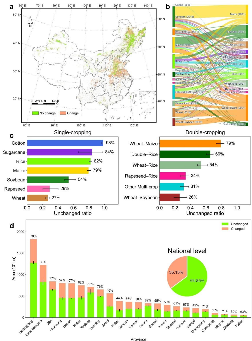
Figure 6 Cropping pattern changes between 2018 and 2021 in China. (a) spatial distribution of changed cropping patterns; (b)Flows of cropland transitions among cropping patterns; (c) unchanged ratio of single- and double-cropping systems; (d) Provincial average unchanged and changed cropland areas.
