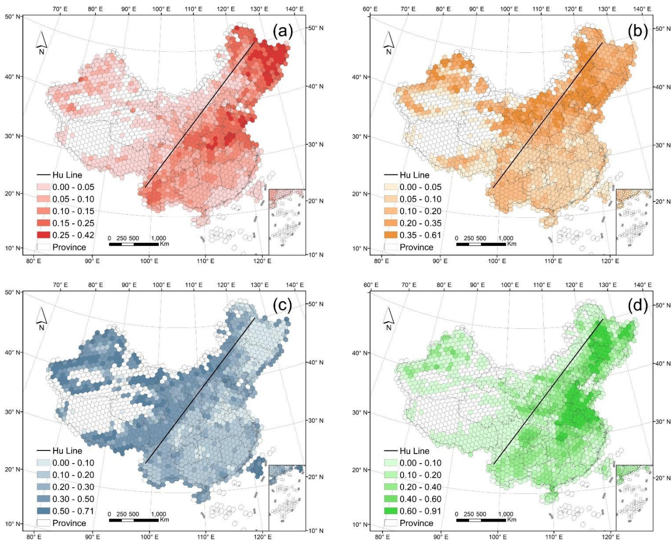
Figure 3. Proportional distribution of cropland and uncertain classes (Confused, Low-consistency, Unlabelled). Fig 3a, Proportional distribution of Confused areas. Fig 3b, Proportional distribution of Low-consistency areas. Fig 3c, Proportional distribution of Unlabelled areas. Fig 3d, Proportional distribution of Cropland.
