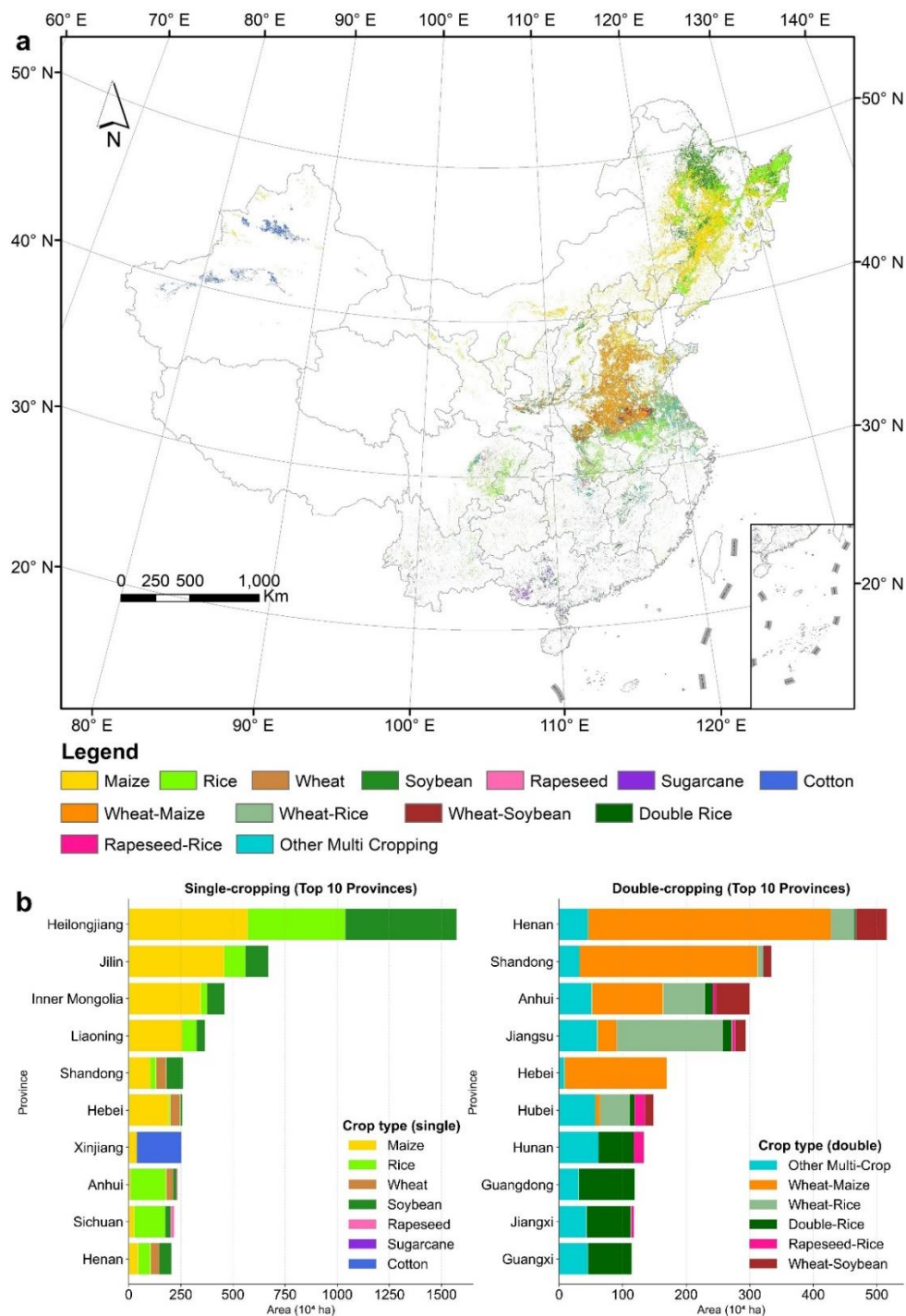
325 Figure 5 Our maps of Cropping Pattern in China (year 2020 as an example). (a) spatial distribution of cropping patterns; (b) crop area aggregated at the province level.
