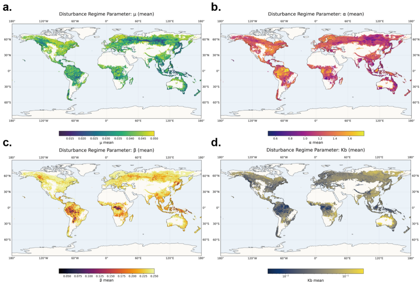
Figure 4. Global patterns of predicted disturbance regime parameters. The four panels show the gridded global maps of ensemble means for (a) \mu , (b) \alpha , (c) \beta , and (d) K_b . Each parameter is displayed with a distinct color scale to highlight its unique spatial patterns.
