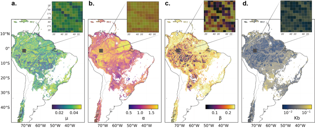
300 Figure 3. Example of the Tile-Level Dataset for a region in the Amazon basin. The four panels show the spatial distribution of the mean predicted (a) Disturbance Rate ( \mu ), (b) Gap-size Distribution \alpha , (c) Disturbance Severity \beta , and (d) Background Mortality K_b . Each colored square represents a single 25 \times 25 km landscape tile. The inset in each panel provides a magnified view of a 0.25^\circ \times 0.25^\circ area, illustrating how multiple high-resolution tiles are nested within the area of a single grid cell from the gridded global product.
