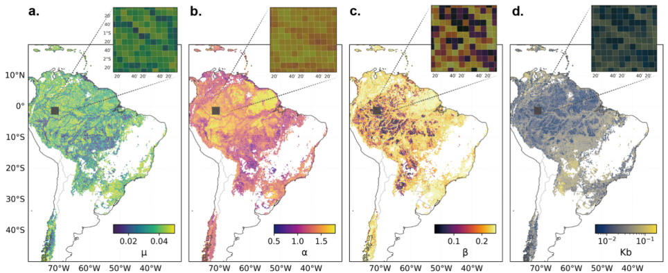
Figure 3. Example of the Tile-Level Dataset for a region in the Amazon basin. The four panels show the spatial distribution of the mean predicted (a) Disturbance Rate \mu , (b) Gap-size Distribution \alpha , (c) Disturbance Severity \beta , and (d) Background Mortality K_b . Each colored square represents a single 25 \times 25 km landscape tile. The inset in each panel provides a magnified view of a 2.5^\circ \times 2.5^\circ region, illustrating the spatial arrangement of multiple 25 \times 25 km tiles.
