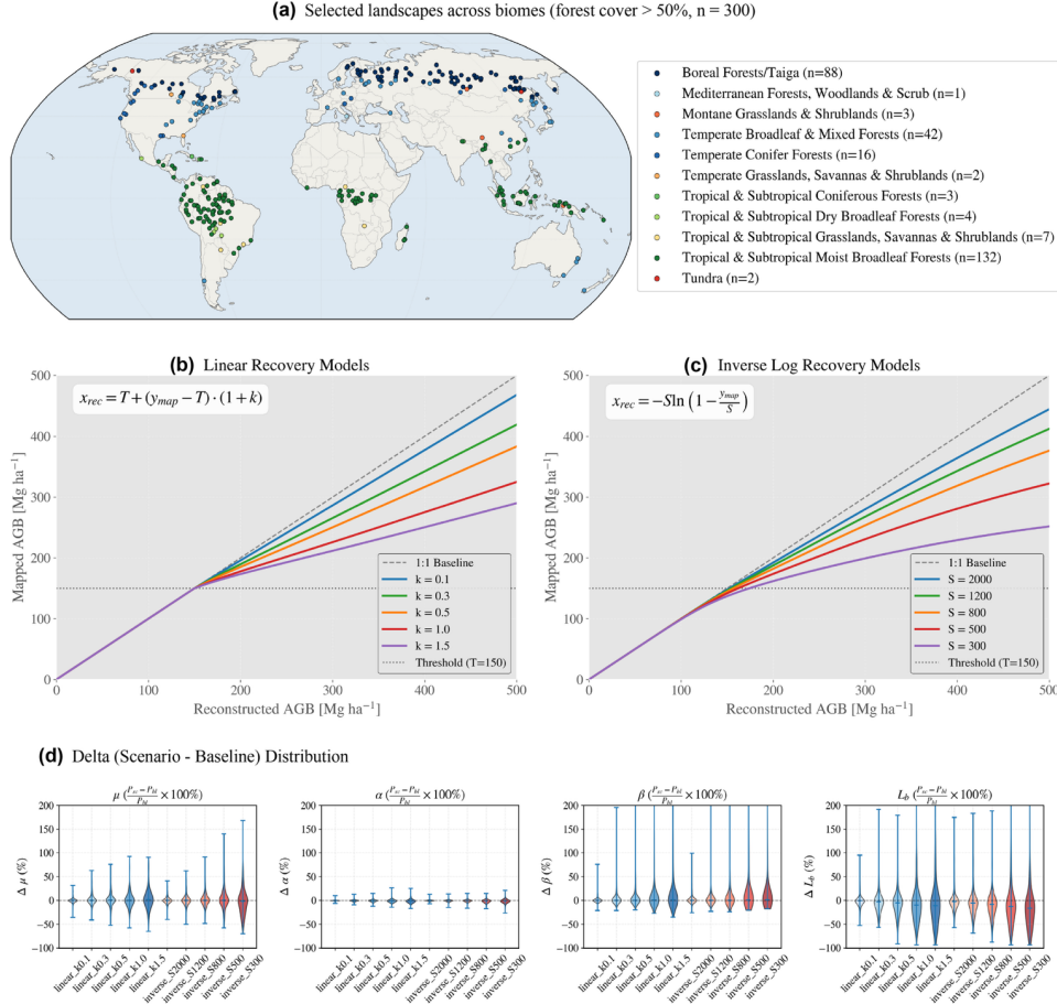
Figure 9. Sensitivity of predicted DRPs to potential dampening of spatial variance across global landscapes. (a) Geographic distribution of the 300 randomly selected baseline landscapes (forest cover > 50%) across major biomes. (b, c) Mathematical configurations for the (b) linear and (c) inverse logarithmic recovery models used to synthetically inject variance for AGB values exceeding high-biomass thresholds. The linear model uses a proportional scaling parameter k \in [0.1, 1.5] while the inverse model uses a parameter S \in [300, 2000] . Both methods apply a continuous sigmoid weight function to smoothly blend the original and recovered above-ground biomass (AGB). (d) Multi-panel violin plots displaying the relative percentage changes ( \Delta P = \frac{P_{sc} - P_{bl}}{P_{bl}} \times 100\% , where sc denotes the reconstructed AGB and bl denotes the mapped
