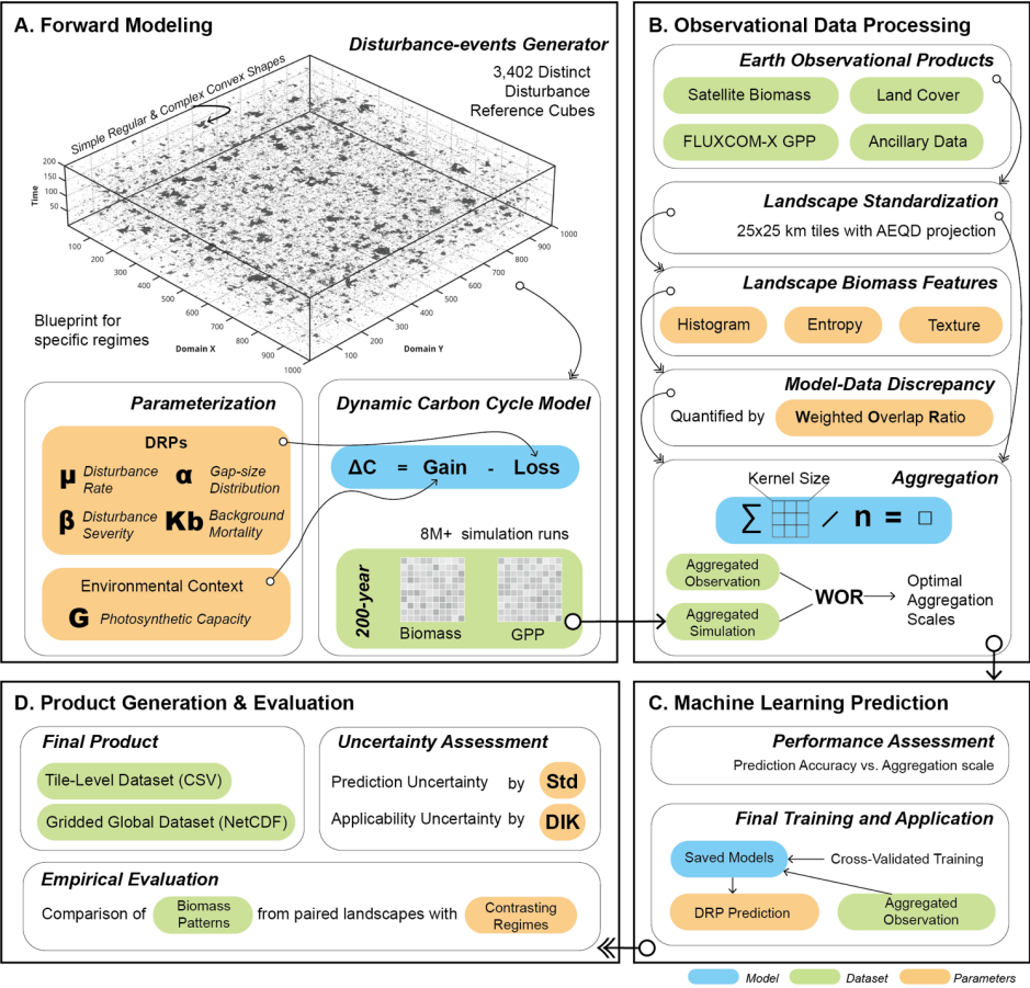
140 Figure 1. Conceptual workflow of the disturbance regime prediction framework. The framework is organized into four stages. (A) Forward Modeling: A synthetic dataset is created by simulating how known disturbance regimes ( \mu , \alpha , \beta , K_b ) produce unique biomass patterns. (B) Observational Data Processing & Discrepancy Analysis: Global satellite biomass product is processed into standardized tiles, and the discrepancy between the simulated and observed data is resolved using a spatial aggregation strategy. (C) Machine Learning Prediction: A Random Forest model is trained on the aligned synthetic data and 145 applied to the observed data to predict disturbance regimes. (D) Product Generation & Evaluation: The tile-level and gridded global datasets are produced and then evaluated for uncertainty and plausibility.
