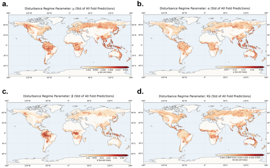
Figure 5. Comprehensive prediction of uncertainty of disturbance regime parameters. The four panels show the global gridded maps of the comprehensive prediction of uncertainty (std_all_folds) for each parameter. This metric represents the standard deviation of all cross-validation fold predictions from all landscape tiles within each 0.25° grid cell, thereby integrating both model ensemble uncertainty and sub-grid spatial heterogeneity. Higher values, indicated by warmer colors on a shared color scale, represent greater overall uncertainty. The number of landscape tiles contributing to each grid cell is provided in the tile_count layer of the dataset (see Supplementary Information).
