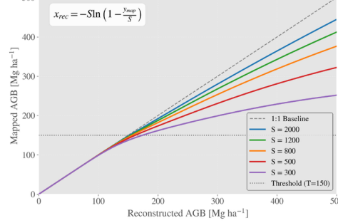
(c) Inverse Log Recovery Models
