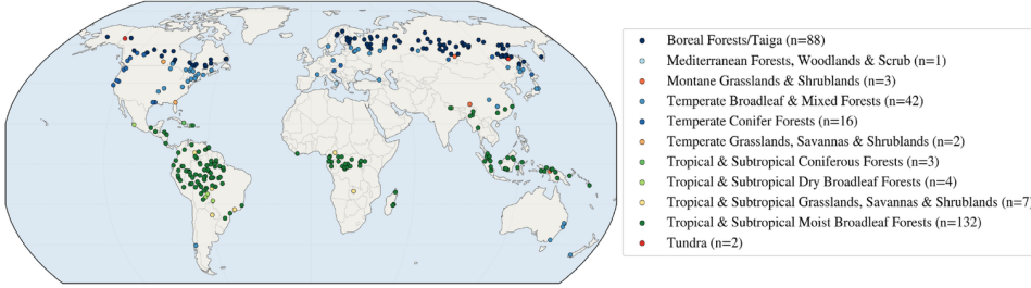
(b) Linear Recovery Models
