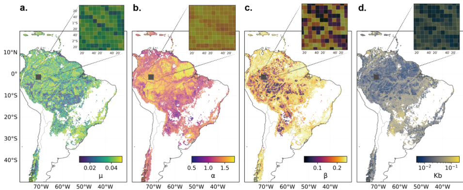
Figure 3. Example of the Tile-Level Dataset for a region in the Amazon basin. The four panels show the spatial distribution of the mean predicted (a) Disturbance Rate ( \mu ), (b) Gap-size Distribution \alpha , (c) Disturbance Severity \beta , and (d) Background Mortality K_b . Each colored square represents a single 25 \times 25 km landscape tile. The inset in each panel provides a magnified view of a 0.25° \times 0.25° area, illustrating how multiple high-resolution tiles are nested within the area of a single grid cell from the gridded global product.
