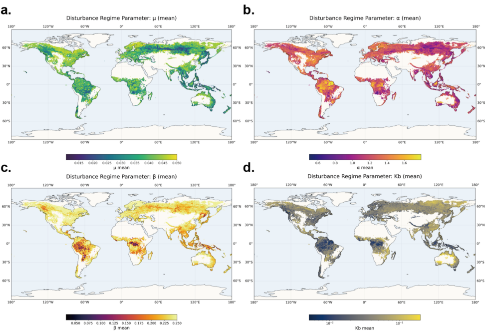
485 Figure 4. Global patterns of predicted disturbance regime parameters. The four panels show the gridded global maps of ensemble means for (a) \mu , (b) \alpha , (c) \beta , and (d) K_b . Each parameter is displayed with a distinct color scale to highlight its unique spatial patterns.
