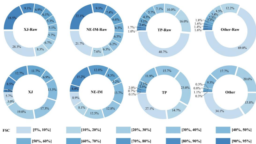
Figure 6: Distributions of tile-level mean FSC values before and after quality control. The upper and lower panels show the mean FSC distributions of the original and post-QC AI-ready samples, respectively, for the four sub-regions.
