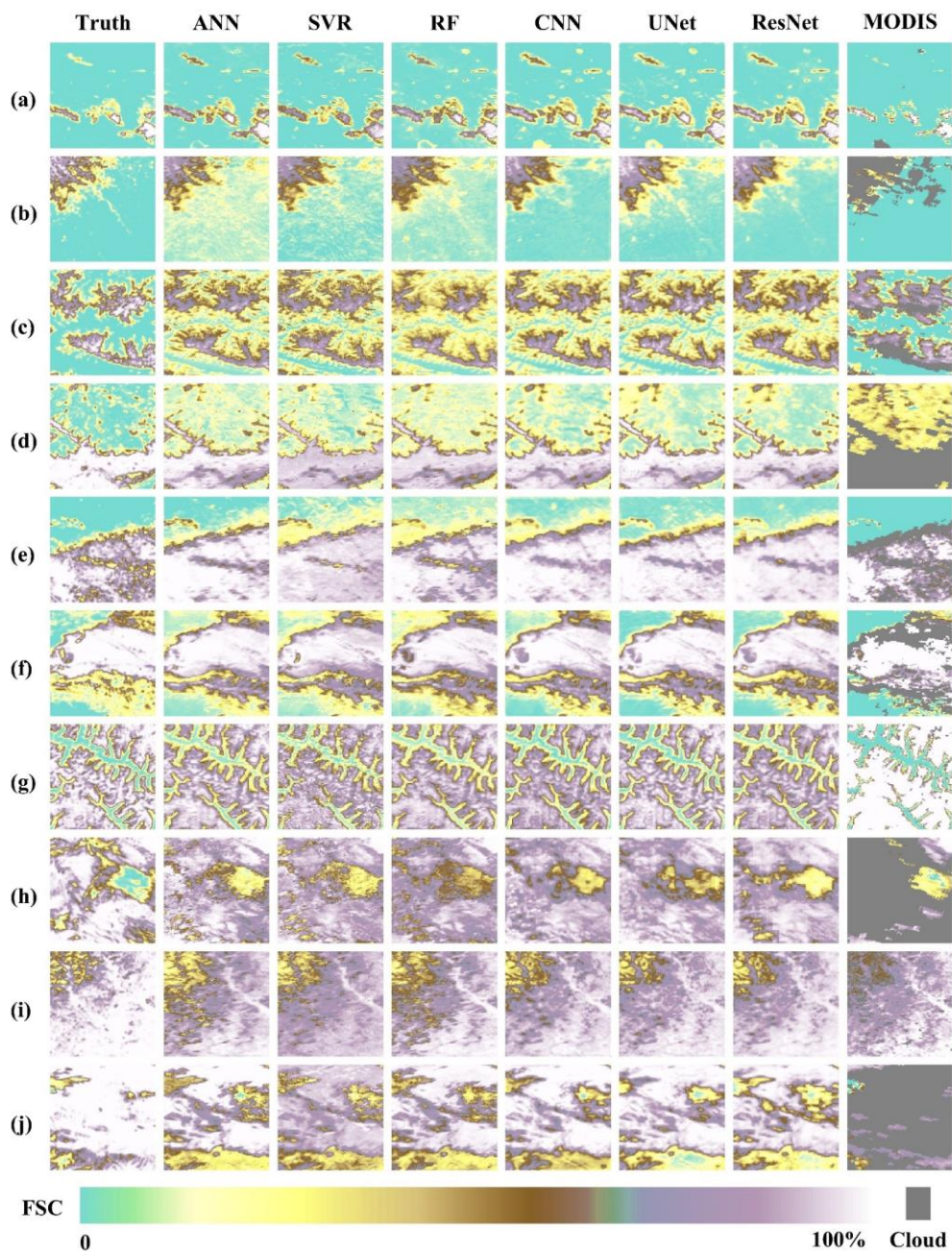
520 Figure 12: Same as Figure 9, but samples from the testing dataset.
