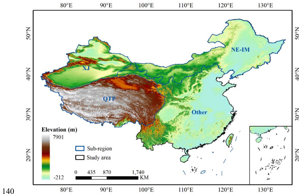
Figure 1: Overview of the study area. The entire study domain is divided into four subregions: Xinjiang (XJ), Qinghai-Tibetan Plateau (QTP), Northeast-Inner Mongolia (NE-IM), and Other regions.
