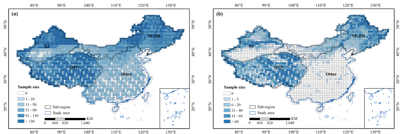
365 Figure 5: Spatial and snow condition completeness of the MODIS FSC sample dataset. (a) and (b) show the spatial distribution of the original and the post-QC AI-ready FSC samples, respectively.
