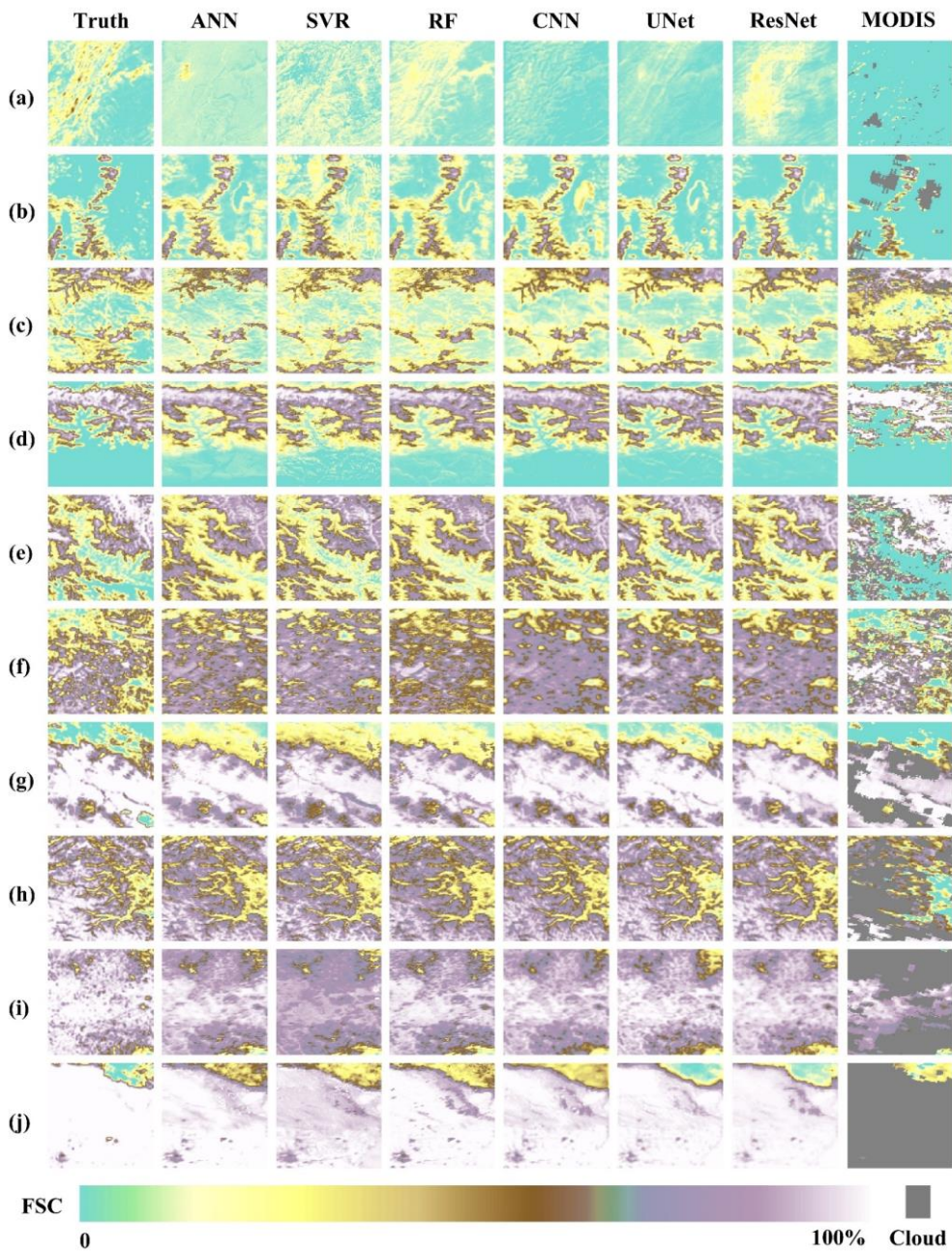
Figure 11: FSC distributions of the reference truth (sample labels, first column), six benchmark models, and the MODIS standard FSC product (last column) for example training samples. Panels (a)-(j) represent different snow cover conditions, spanning the full FSC range of [0-10%], [10-20%], ..., [90-100%], respectively.
