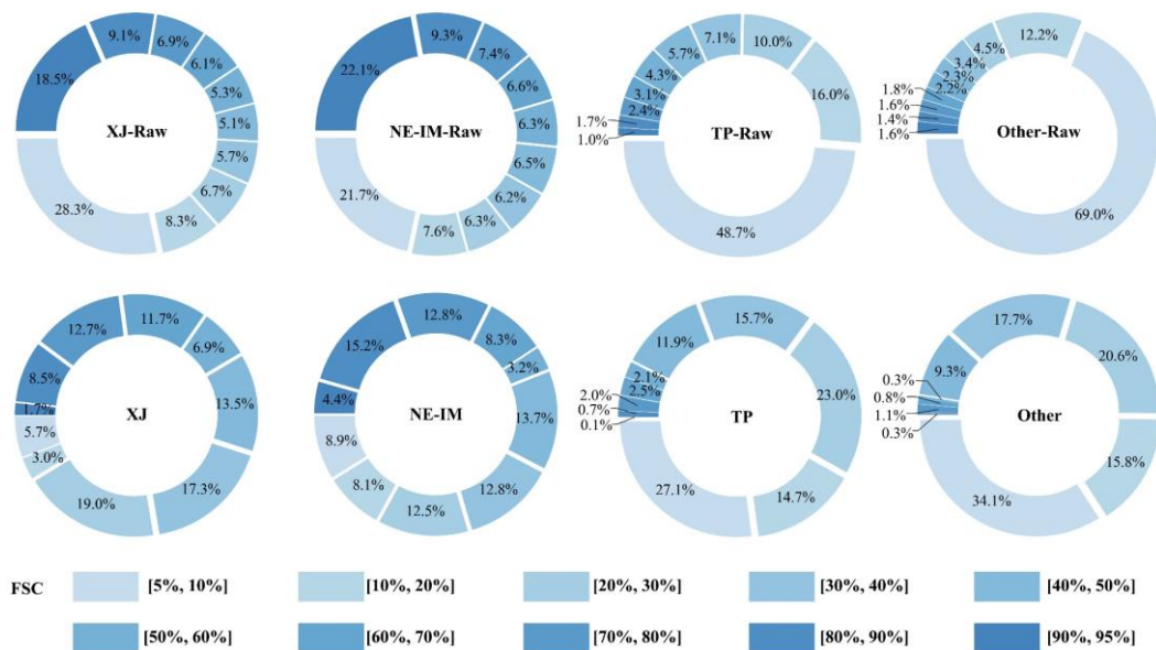
370 Figure 6: Distributions of tile-level mean FSC values before and after quality control. The upper and lower panels show the mean FSC distributions of the original and post-QC AI-ready samples, respectively, for the four sub-regions.
