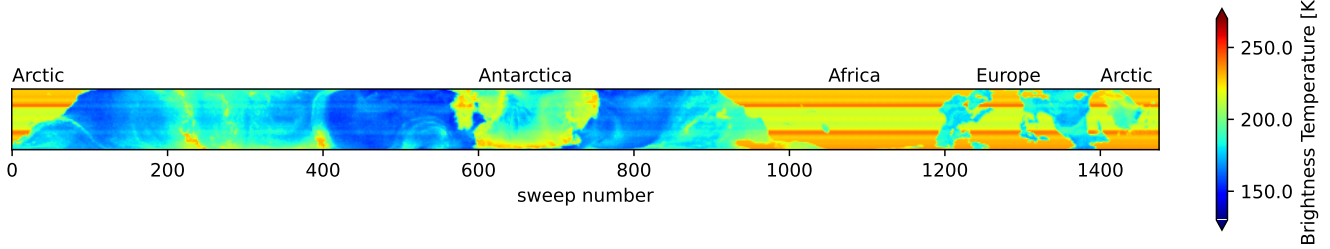
Figure 1. Example of the types of swaths the swath filter is meant to detect. In this swath, T_B over land and ice is constant along track, as the true T_B is above 220 K.
