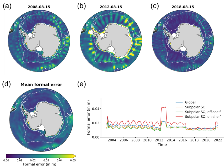
Figure 9: Daily formal error maps for one August day in (a) 2008 (Envisat only), (b) 2012 (CryoSat-2 only) and (c) 2018 (CryoSat-2, SARAL and Sentinel-3A). (d) Time-averaged daily formal error map over the full period. (e) Spatially averaged formal error time series, for several subdomains: south of 50°S in blue, subpolar Southern Ocean in orange, off-shelf subpolar Southern Ocean in green and on-shelf subpolar Southern Ocean in red. The subpolar Southern Ocean is south of the white dashed contour in the maps; the off-shelf/on-shelf separation is defined by the 1000 m bathymetric contour shown as a white full contour.
