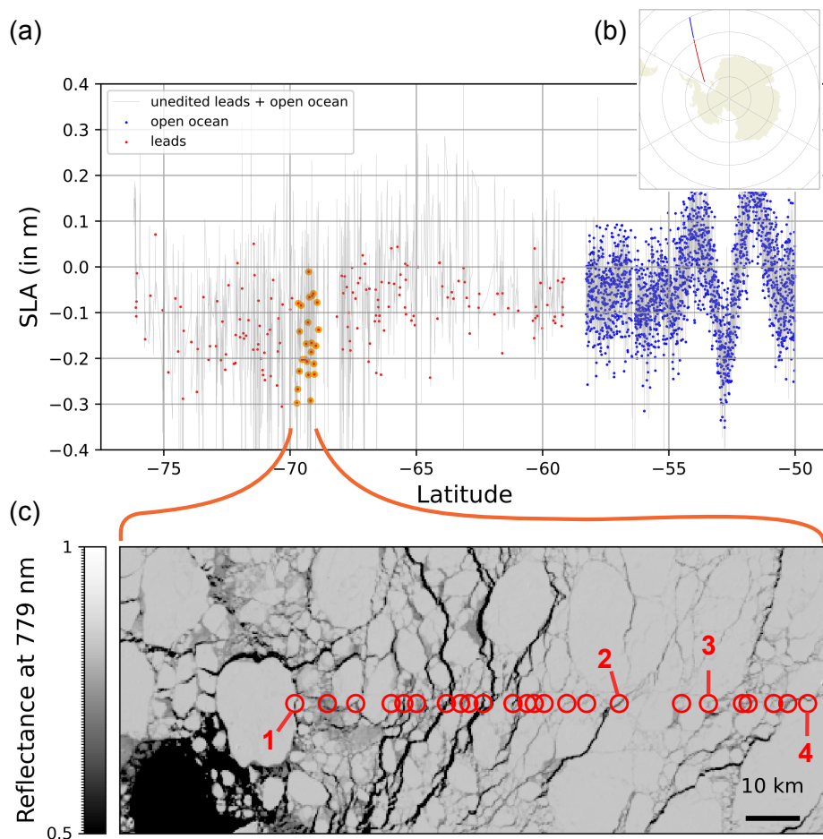
Figure 4: (a) SLA from one Envisat pass, on 11 October 2003 . Blue points are edited SLA from open-ocean waveforms. Red points are edited SLA from lead waveforms. The gray line aggregates SLA estimates from open-ocean or lead waveforms, before the editing. (b) Trajectory of the along-track data shown in (a). (c) Surface reflectance at 779 nm along the trajectory, measured by MERIS. SLA estimates shown in orange in panel a are collocated on the MERIS swath. Points labelled 1 to 4 are discussed in the text.
