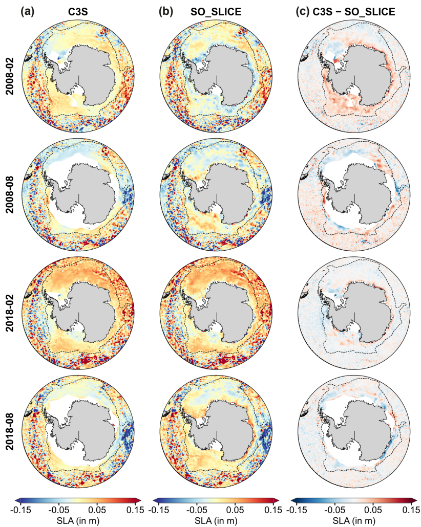
Figure 5: Monthly SLA fields relative to the 2003–2021 period from (a) C3S and (b) SO_SLICE, and (c) the difference between C3S and SO_SLICE. Each row corresponds to a specific month, from top to bottom: February 2008, August 2008, February 2018 and August 2018.
