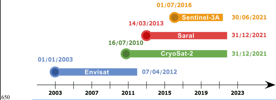
Figure 1: Satellite missions timeline, with the start and end dates of data merging into SO SLICE indicated as colored text (dd/MM/YYYY).
