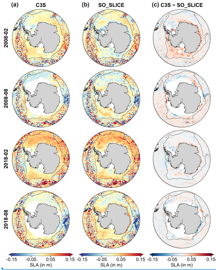
Figure 5: (a) Monthly SLA fields relative to the period 2003–2021 from C3S (b) Monthly SLA fields relative to the period 2003–2021 from SO_SLICE (c) Difference between C3S and SO_SLICE. Each row corresponds to a specific month, from top to bottom: February 2008, August 2008, February 2018 and August 2018.
