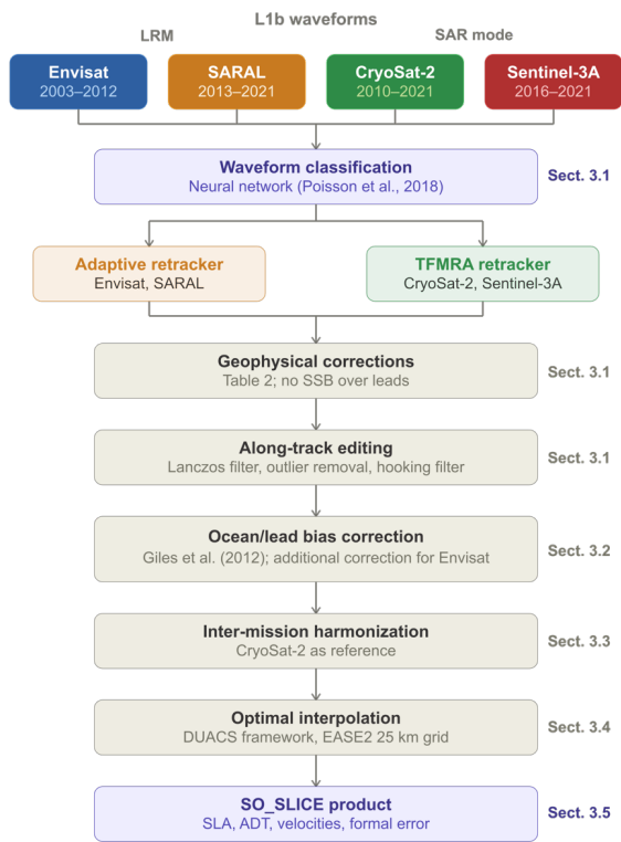
Figure 3: Data processing pipeline of SO SLICE, from the L1b waveforms to the final gridded product. Each key step has its associated box and is discussed in the referred subsection.
