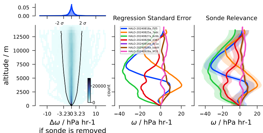
Figure 6. Histogram of the error \epsilon_\omega , with profiles from all circles where any sonde is removed from its circle in lower panel (left). Regression standard error for seven arbitrary circles (middle). Range of minimum and maximum estimate if a sonde is removed from circle calculation for the same circles (right).
