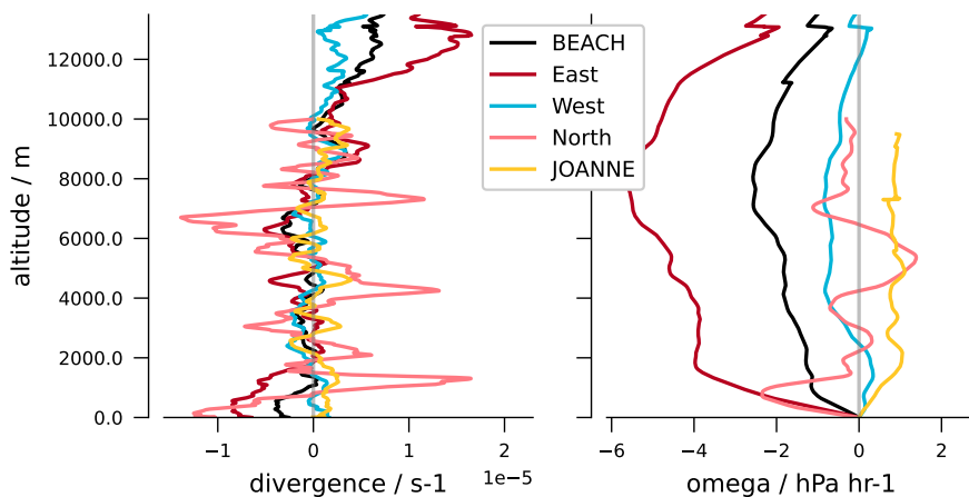
Figure 10. Average divergence (left) and \omega (right) for the full campaign, as well as split into East and West Atlantic. The average profiles from the JOANNE dataset showing typical characteristics for the winter trades in the Western Atlantic are added for comparison. BEACH Level 4 data is used for this plot.
