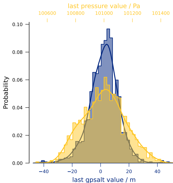
Figure 4. Distribution of surface pressure and gpsalt values from all sondes. (xrange alt: 100m, xrange p: 10hPa
