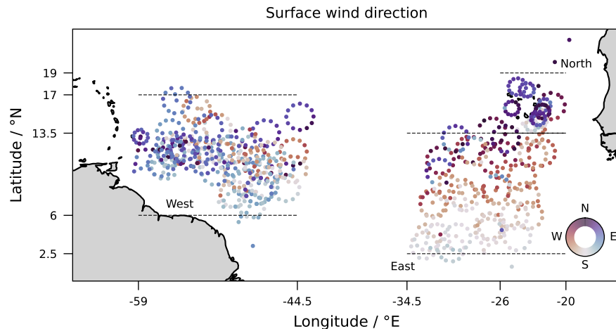
Figure 7. Mean wind direction in the lowest 50m for all sondes. Level 3 data is used for this plot.
