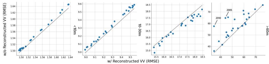
Fig. 14. RMSE differences between models with and without reconstructed VV. Cropped from Fig. 9 of the original manuscript.
