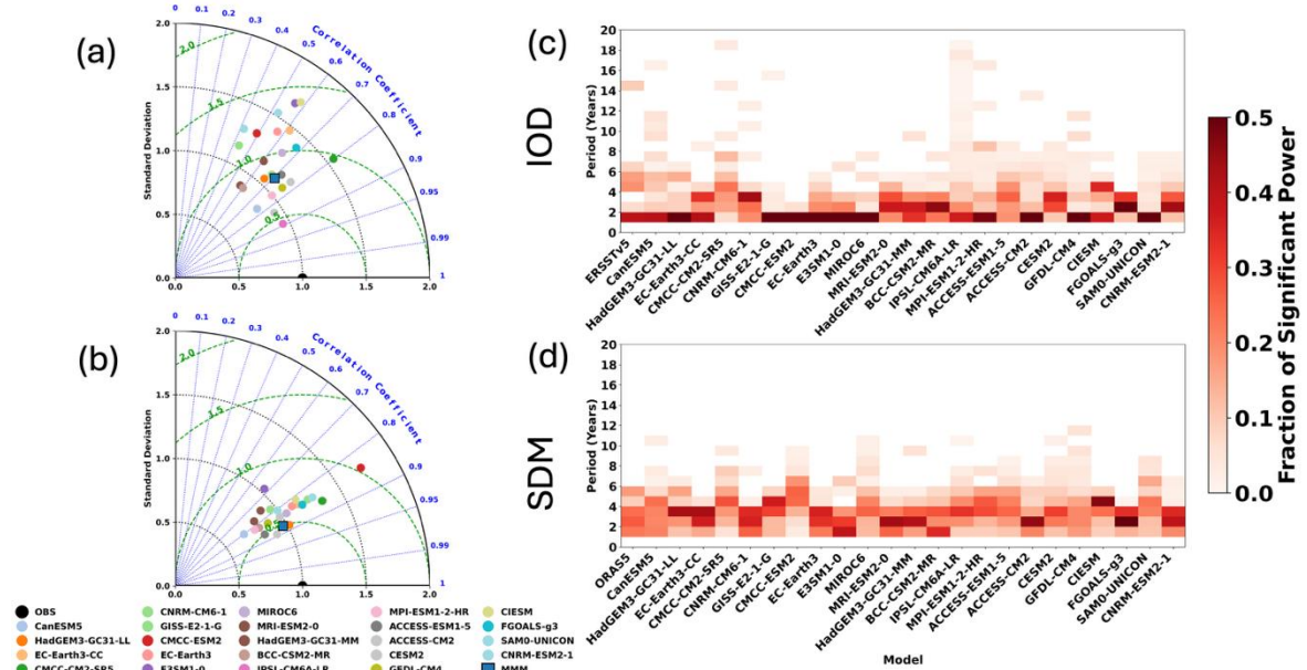
Fig. 7 Taylor diagram for regression based spatial pattern of (a) IOD from ERSSTv5 (b) SDM from ORAS5, 23 CMIP6 models and MMM. (c, d) Power spectrum of normalised time series for (c) IOD and (d) SDM climate mode indices from observation/reanalysis (ORAS5) and 23 CMIP6 models. The power is plotted for values above the threshold (mean + standard error) after performing power analysis using a Monte Carlo-based significance test.
