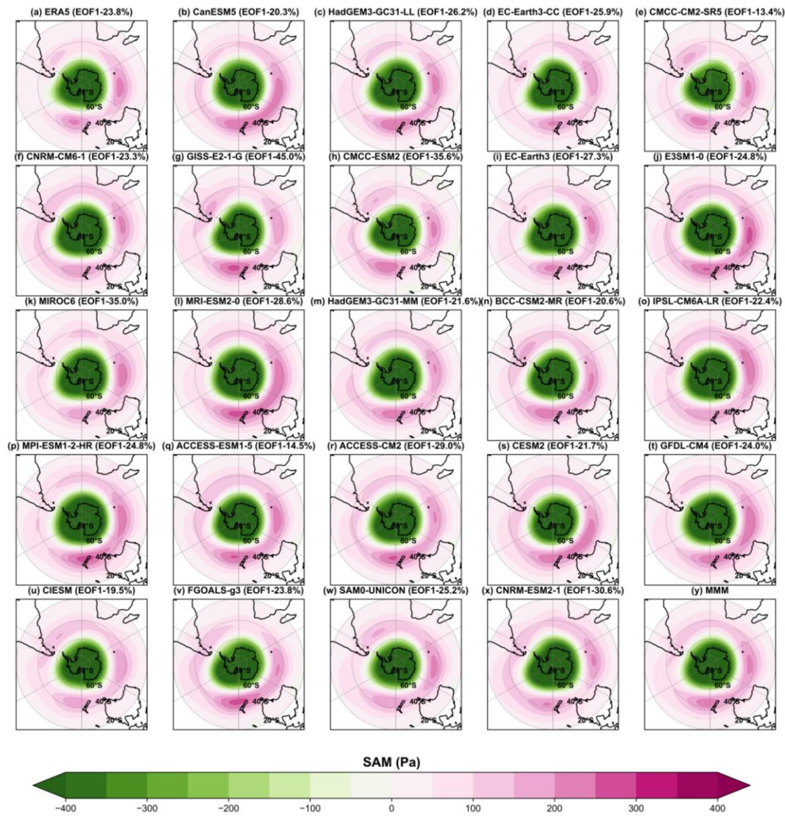
Fig. 10 Spatial pattern of regression-derived atmospheric response for the Southern Annular Mode (SAM). Values are sea level pressure anomalies (in Pa) regressed against the EOFPC (SAM) time series from (a) ERA5, (b-x) 23 CMIP6 models and (y) MMM. Here MMM represents the average of spatial pattern of regression from 23 CMIP6 models. The bracketed text and numbers in black are the mean variance explained by the EOF representing SAM between observation and models.
