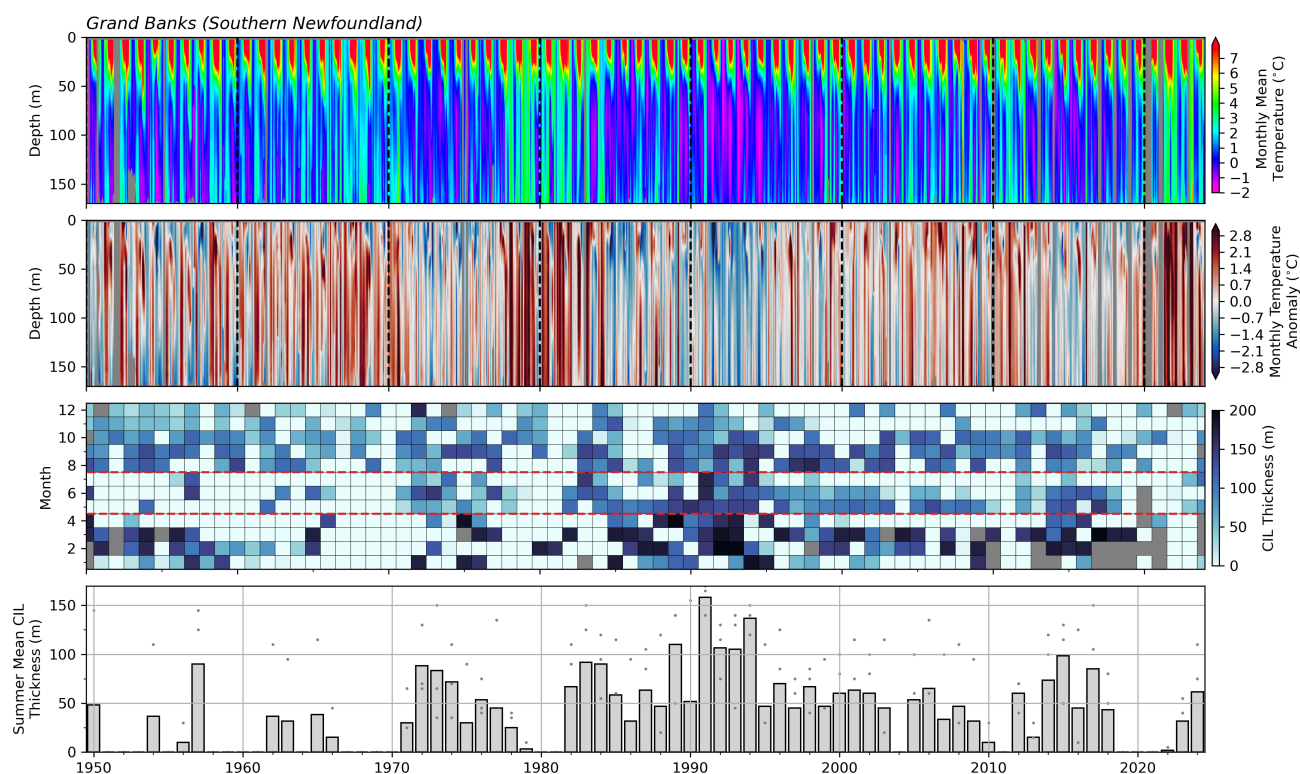
Figure 8. Grand Banks (Southern Newfoundland) temperature Hovmöller diagram (first row), temperature anomaly Hovmöller diagram calculated from the 1991-2020 climatology (second row), monthly CIL thickness (third row), and summer (May to July) mean CIL thickness (fourth row) from 1950 to 2024. The months of May, June, and July are used to calculate the summer mean CIL thickness are outlined by a dashed red line (third row). The grey grid cells in the third row represent missing data. The grey dots in the bottom figure show all available measurements for the summer mean CIL thickness for a particular year. The area of interest used to calculate all metrics is shown in Fig 1. The CIL is defined as all depths where temperature is less than 0 °C. For many months, the CIL thickness is 0 m, therefore making the grey dots not visible.
