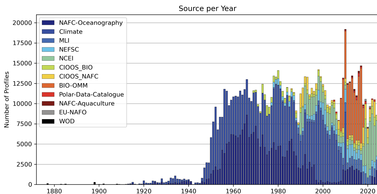
Figure 3. Number of profiles associated with each CASTS source (1873-2023) using the CASTS source variable. The source and its corresponding colour are given in the legend in the top left corner.
