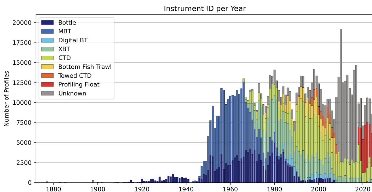
Figure 2. Number of occurrences for each instrument type per year (1873-2023) using the CASTS instrument identification variable. The instrument identification of each cast and its corresponding colour is given in the legend in the top left corner. Profiles with an empty or unique instrument identification were categorized as unknown. The large number of unknown profiles from 2008 to 2018 are associated with the BIO-OMM data source where instrument identification is not provided.
