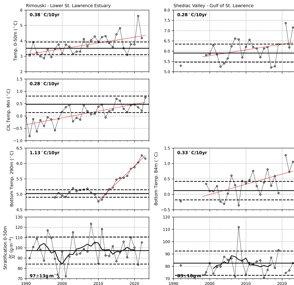
Figure 7. Depth-averaged (0-50m) annual mean of temperature (top row) reconstructed from monthly anomalies for Rimouski (left column) and Shediac Valley (right column). The associated linear trend for both stations is shown in red, with the trend written in the top left corner. The CIL minimum temperature and linear trend for Rimouski are shown in the second row. The bottom temperature at Rimouski and Shediac Valley is shown in the third row, taken at 290 m and 84 m depth respectively. The linear trend from Rimouski was calculated from 2010 to 2023 and 1998 to 2023 for Shediac Valley. The annual mean stratification between 0 and 50 m reconstructed from monthly anomalies are also presented for both stations (bottom row). The mean stratification over the 1990-2010 period is also provided in the bottom left corner. In all panels, the yearly average is shown by the white dots and thin black line. The mean reconstructed temperature, CIL temperature, and stratification over the 1990-2010 period are given by the solid black horizontal line, while one standard deviation about the mean is shown by the dashed lines.
