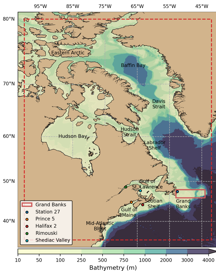
Figure 1. Bathymetric map of the NW Atlantic and Eastern Arctic. The CIL area and the five DFO AZMP historical oceanographic stations are also given and labeled by the legend in the bottom left corner. Locations referenced in the paper are also labeled directly on the map. The dashed red line shows the CASTS domain.
