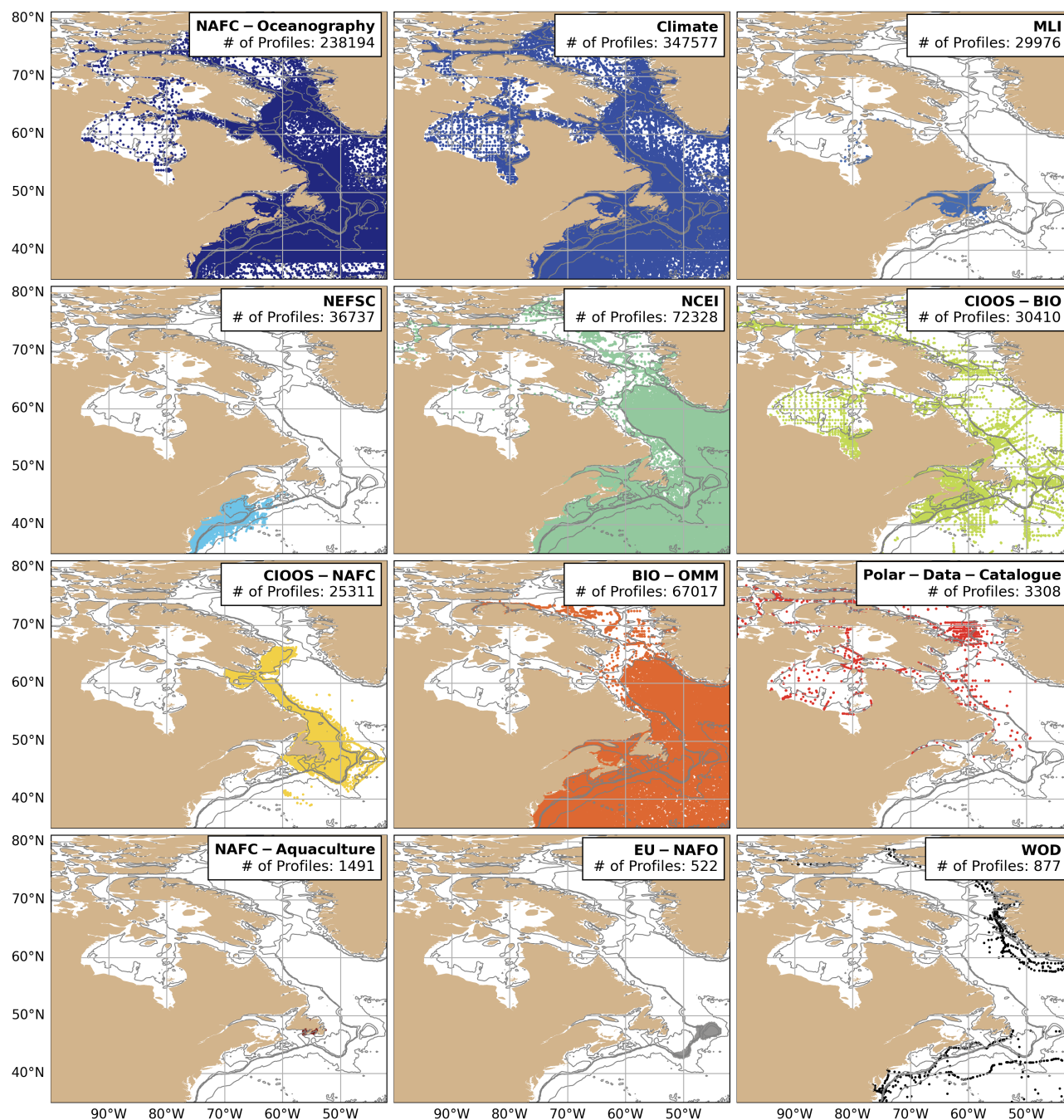
Figure 4. Distribution of profiles organized by source (1873-2023) using the CASTS source variable. The name of the source and the number of profiles associated are given in the top right corner of each subplot. The lines of constant latitude and longitude are also provided. Isobaths are shown at 100 m, 500 m, 1000 m, and 4000 m.
