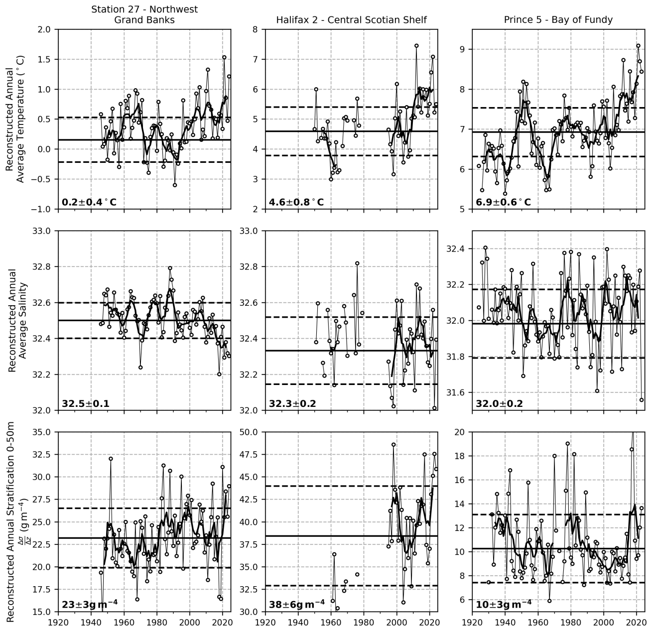
Figure 6. Depth-averaged annual mean of temperature (top row) and salinity (middle row) reconstructed from monthly anomalies for Station 27 (0-176 m), Halifax 2 (0-150 m), and Prince 5 (0-50 m). The annual mean stratification between 0 and 50 m reconstructed from monthly anomalies is also presented (bottom row). In all panels, the yearly average is shown by the white dots and thin black line. The five-year running average is shown by the thick black line. The mean temperature anomaly, salinity anomaly, and stratification over the 1950-2000 period are given by the solid black horizontal line. One standard deviation about the mean is shown by the dashed lines. The mean temperature, salinity and stratification over the 1950-2000 period is also provided in the bottom left corner.
