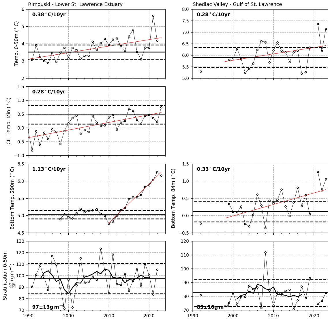
Figure 7. Depth-averaged (0-50 m) annual mean of temperature (top row) reconstructed from monthly anomalies for Rimouski (left column) and Shediac Valley (right column). The associated linear trend for both stations is shown in red, with the trend written in the top left corner. The CIL minimum temperature and linear trend for Rimouski are shown in the second row. The bottom temperature at Rimouski and Shediac Valley is shown in the third row, taken at 290 m and 84 m depth respectively. The linear trend from Rimouski was calculated from 2010 to 2023 and 1998 to 2023 for Shediac Valley. The annual mean stratification between 0 and 50 m reconstructed from monthly anomalies are also presented for both stations (bottom row). The mean stratification over the 1990-2010 period is also provided in the bottom left corner. In all panels, the yearly average is shown by the white dots and thin black line. The mean reconstructed temperature, CIL temperature, and stratification over the 1990-2010 period are given by the solid black horizontal line, while one standard deviation about the mean is shown by the dashed lines.
