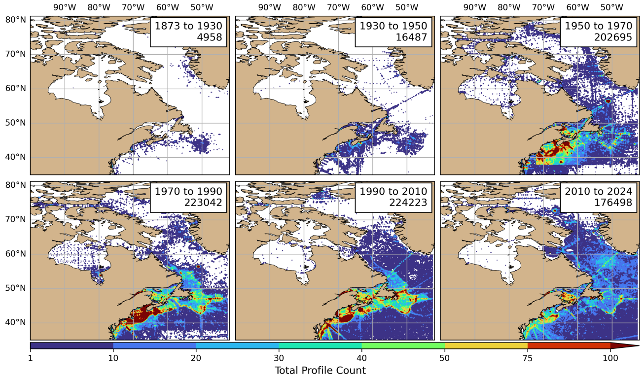
Figure 5. Total number of profiles, binned into 0.25 degree length grid cells using CASTS from 1873 to 1929, 1930 to 1949, 1950 to 1969, 1970 to 1989, 1990 to 2009, and 2010 to 2024. Areas where no casts are present are shown in white. The lines of constant latitude and longitude are also provided. The time period and total number of casts are shown in the top right corner.
