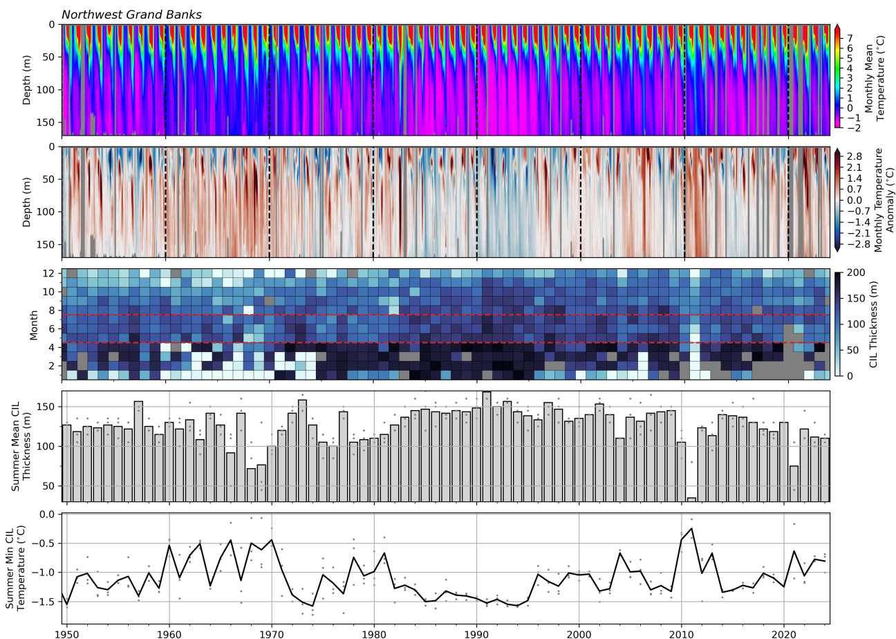
Figure 8. Northwest Grand Banks temperature Hovmöller diagram (first row), temperature anomaly Hovmöller diagram calculated from the 1991-2020 climatology (second row), monthly CIL thickness (third row), summer (May to July) mean CIL thickness (fourth row), and summer mean minimum CIL temperature (fifth row) from 1950 to 2024. The months of May, June, and July are used to calculate the summer mean CIL thickness and mean minimum CIL temperature are outlined by a dashed red line (third row). The grey grid cells in the third row represent missing data. The grey dots in the bottom two rows show all available measurements for the summer mean CIL thickness and summer mean minimum CIL temperature respectively for a particular year. The area of interest used to calculate all metrics is shown in Fig 1. The CIL is defined as all depths where temperature is less than 0 °C. For many months, no CIL is present, therefore making the grey dots not visible. The colour-map used in the first row is not perceptually uniform and was primarily chosen to highlight the CIL layer clearly (i.e. light purple colour).
