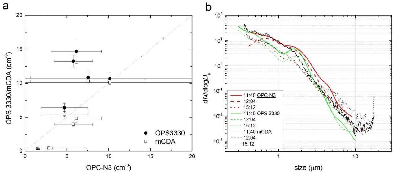
Figure 6. Drone backpack OPC-N3 particulate matter measurements against reference instruments OPS (model 3330, TSI Inc.) and the mCDA (Palas GmbH). Panel a) total aerosol concentration, b) particle number size distribution, both measured within the range of each instrument.
