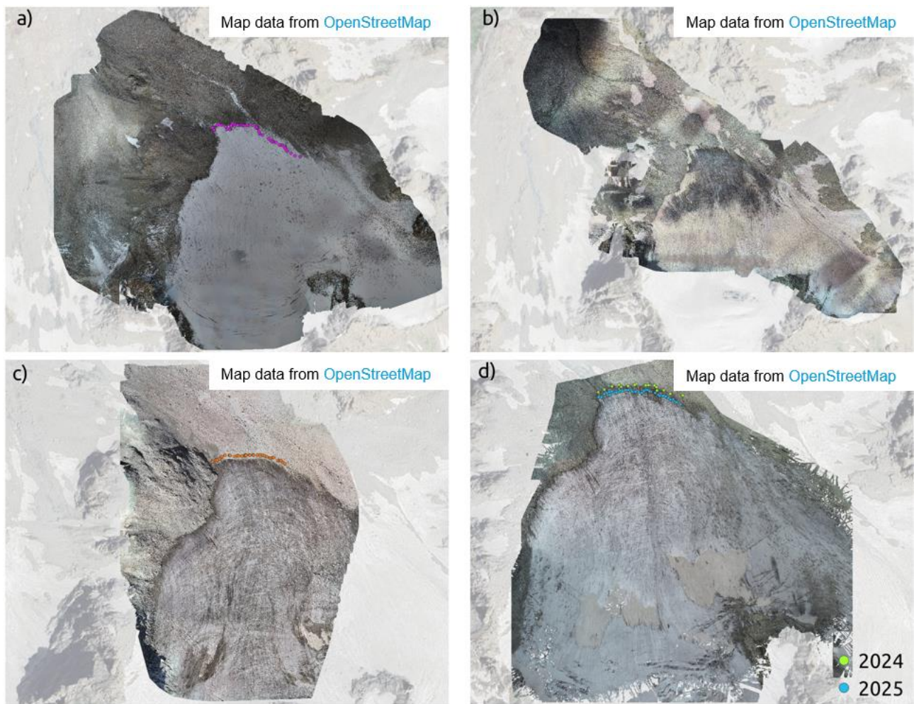
Figure 6. Orthomosaic overlays of GGP generated by Pix4D software for each year: a) 2018, b) 2019, c) 2023 and d) 2024. Ice front locations collected with GPS-surveys from different expedition years. Background image available through OpenStreetMaps.
