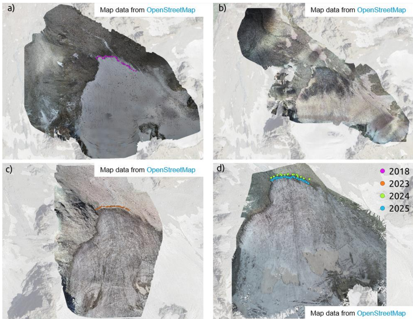
300 Figure 6. Orthomosaic overlays of GGP generated by Pix4D software for each year: a) 2018, b) 2019, c) 2023 and d) 2024. Ice front 305 locations collected with GPS-surveys from different expedition years. Background image available through OpenStreetMaps.
