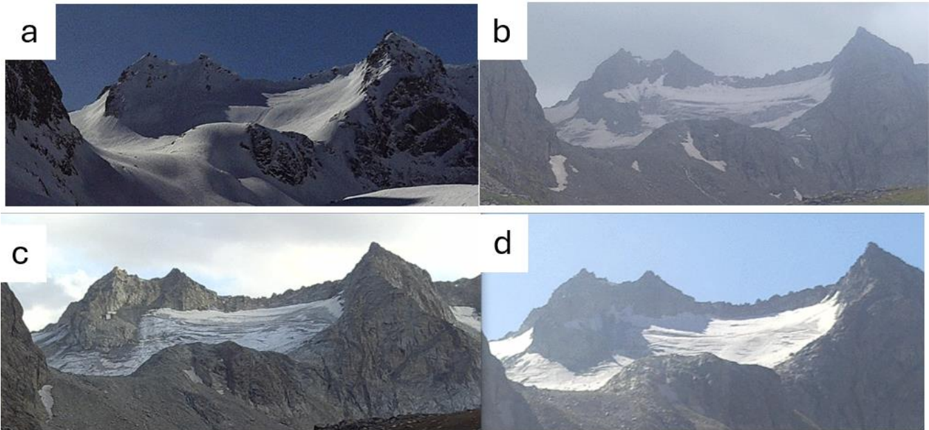
Figure 7. Snow conditions at GGP on a) 31.3.2024 (maximum snow conditions), b) 18.8.2024 (minimum snow conditions), c) 4.9.2023, and d) 4.9.2024.
