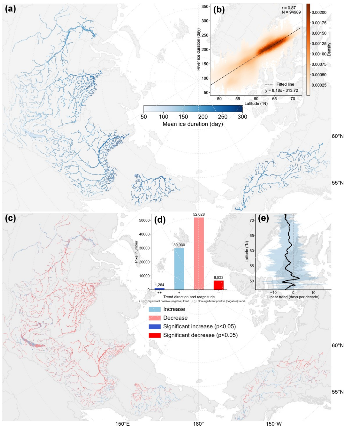
430 Figure 9: Spatial patterns and temporal trends in river ice duration. (a) Spatial distribution of mean ice duration over the 24-year record. (b) Latitudinal relationship between ice duration and geographic latitude. (c) Trends in ice duration estimated with the Theil–Sen slope; significance assessed with the Mann–Kendall test (significant pixels, p < 0.05 , highlighted). (d) Frequency distribution of trend directions and significance. (e) Latitude-wise distribution of mean linear trends in ice duration. The background map is from HydroBASINS dataset (Lehner and Grill, 2013).
