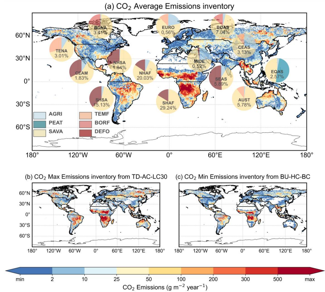
Figure 2. Spatial patterns and regional composition of global biomass burning CO 2 emissions (mean of 2003–2023). (a) Spatial distribution of the annual mean CO 2 emission flux estimated from the mean of the eight inventories in this study. The embedded pie charts show the emission composition for 14 major regions, where: 1) the number in the pie chart indicates the percentage of that region's emissions relative to the global total; and 2) the sectors of the pie chart represent the proportional contribution of six major fire types to the region's total emissions. (b) and (c) show the spatial emission patterns corresponding to the inventory with the highest global total annual emissions (TD-AC-LC30) and the lowest global total annual emissions (BU-HC-BC) among the eight inventories over the entire study period, respectively.
