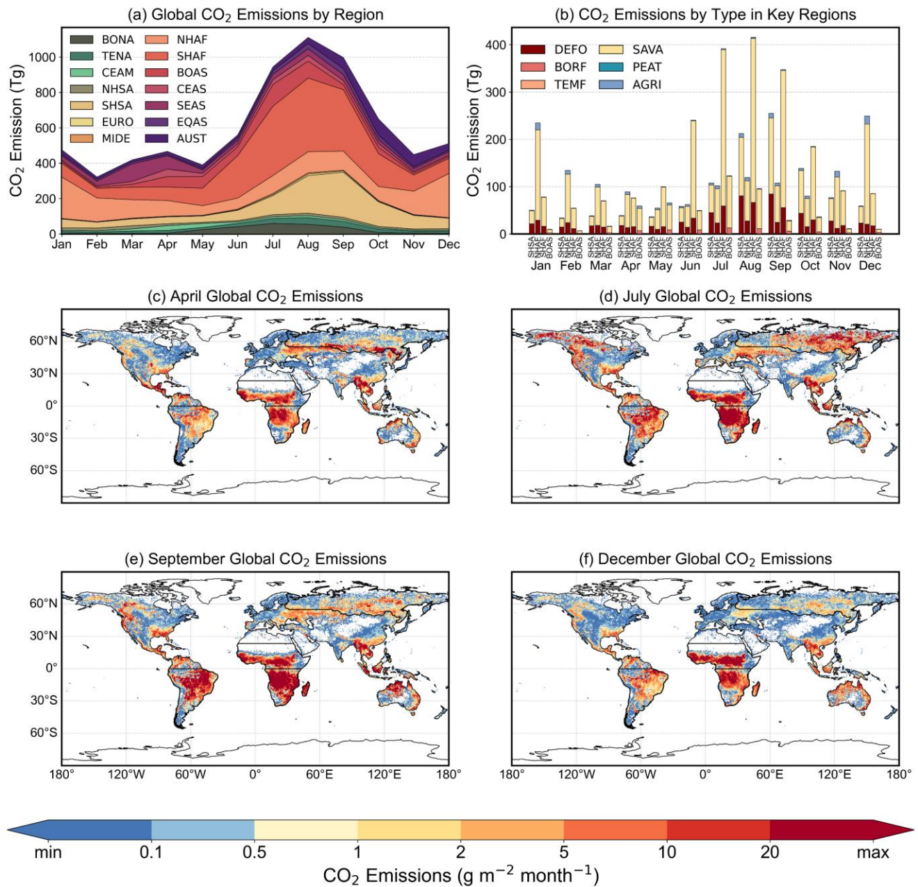
422 Figure 3. Seasonal cycle and spatial dynamics of global biomass burning CO 2 emissions (mean of 2003–2023). 423 (a) Global monthly emissions partitioned by source region. (b) Monthly emissions for the four primary 424 contributing regions, showing the composition by fire type. (c–f) Spatial distribution of mean monthly 425 emission flux during key seasonal phases: April, July, September, and December. 426
