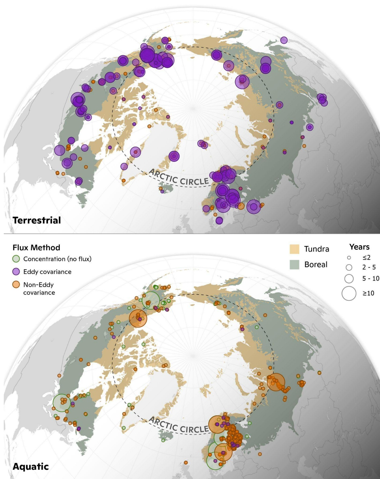
Fig. 1. Numbers of site-months for terrestrial CO 2 and CH 4 flux sites, and aquatic CO 2 and CH 4 flux sites across the Arctic-boreal region. The number of months represented by circles refers to
