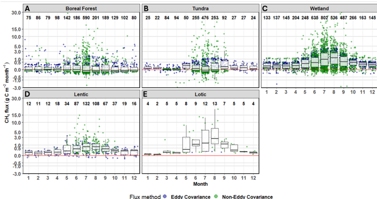
Fig. 8. Monthly CH 4 fluxes across key terrestrial and aquatic classes together with the number of site-months. Note that y axes follow a pseudo-log scale. The tundra classes characterize non-wetland ecosystems in the tundra biome (i.e., dry and moist tundra).
