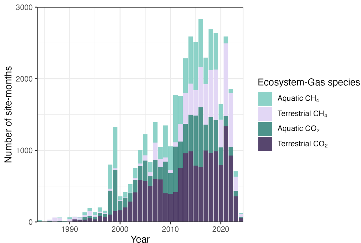
Fig. 3. The number of CO 2 and CH 4 flux site-months across years. Numbers of observations are shown as stacked bars for each year. If a site-month measured both CO 2 and CH 4 , it is counted as separate site-months in the figure (1 CO 2 site-month and 1 CH 4 site-month). The distribution of sites with more recent data is less comprehensive (2022 as an example). This does not imply these sites discontinued data collection, but rather that the data were not made available at the time of this synthesis
