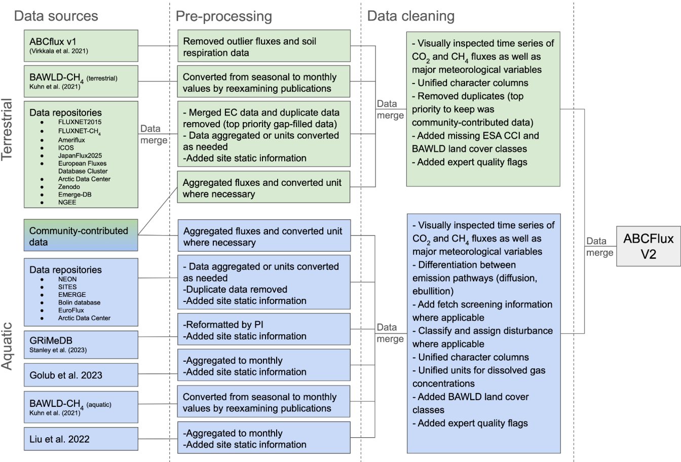
Fig. 2. Flowchart representing the main data compilation steps to produce ABCFlux v2. Note that repositories are listed based on the direct source of data acquisition; for example,
