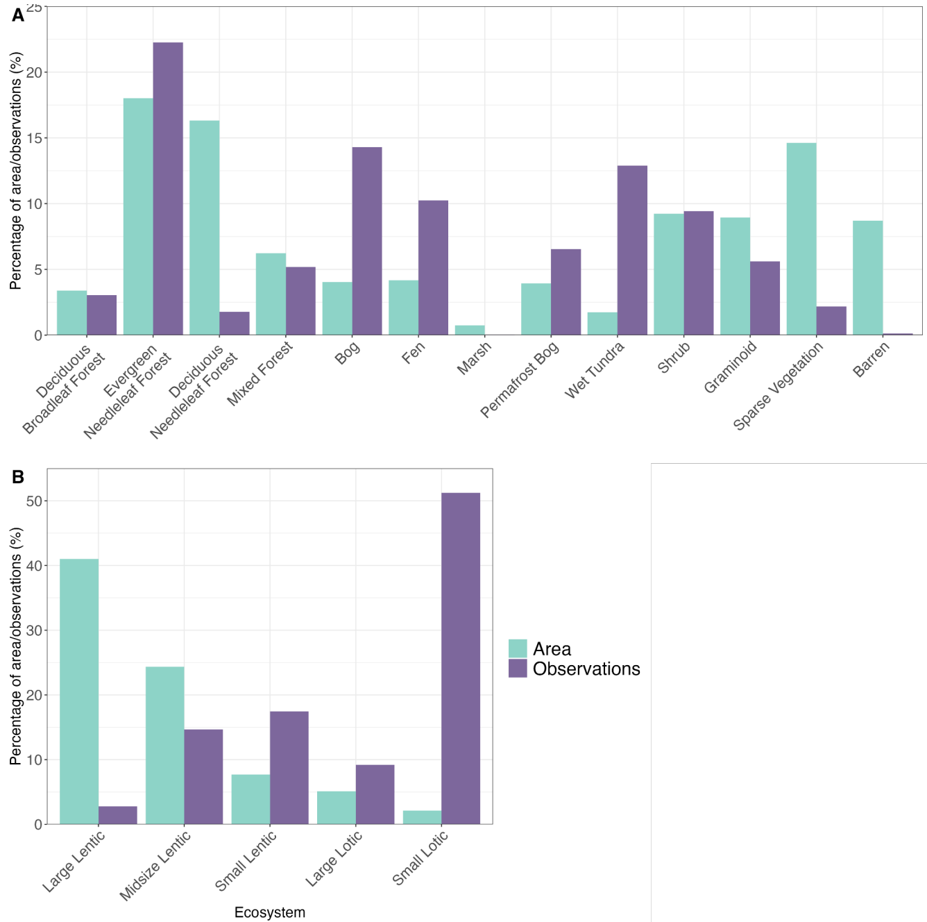
1115 Fig. 6. The coverage of monthly flux observations and areas of key terrestrial (A) and aquatic (B) ecosystem types from the ESA land cover model. Aquatic concentration site-months are included in the figure. Some observations were left unclassified due to the lack of descriptive data and are not shown in the figure. There are 61 site-months of data from marshes, resulting in their proportion appearing nearly zero in the figure.
