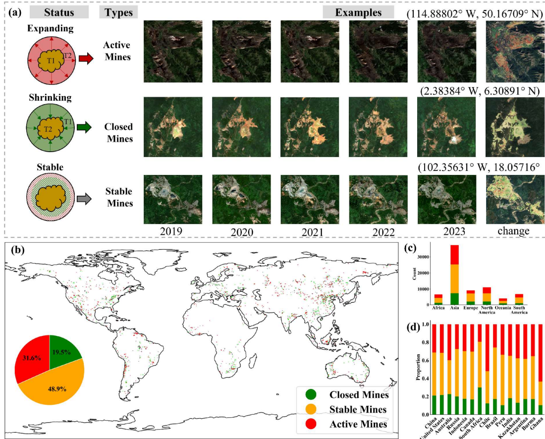
Figure. 8 (a) Classification of development status of mining areas in the recent five years: active, undefined stable, closed. While the figure illustrates the period 2019–2023. (b) Global distribution of three types of mining areas. For the change maps corresponding to each development status category, two distinct change directions are denoted by specific colors: Red pixels indicate a land cover transition from non-mining-related types to mining-related types, representing the expansion of mining areas. Green pixels indicate the inverse transition—from mining-related land cover types to non-mining-related types—representing the shrinkage of mining areas. (c) Continental counts of mining areas types (d). Type structures of the top 15 countries (sorted by total mining areas descendingly).
