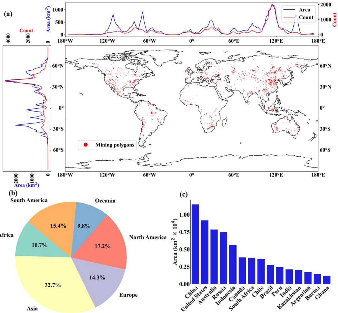
Figure. 5 Global distribution and characteristics of mining polygons. (a) Global distribution of mining polygons and their latitudinal/longitudinal statistics of area and count. Given the visualization effect, the centroids of the polygons are used for display here instead of the actual shapes of the polygons. (b) Continental proportion of the global mining polygons area. (c) Mining polygons area in the top 10 countries in terms of total mining area.
