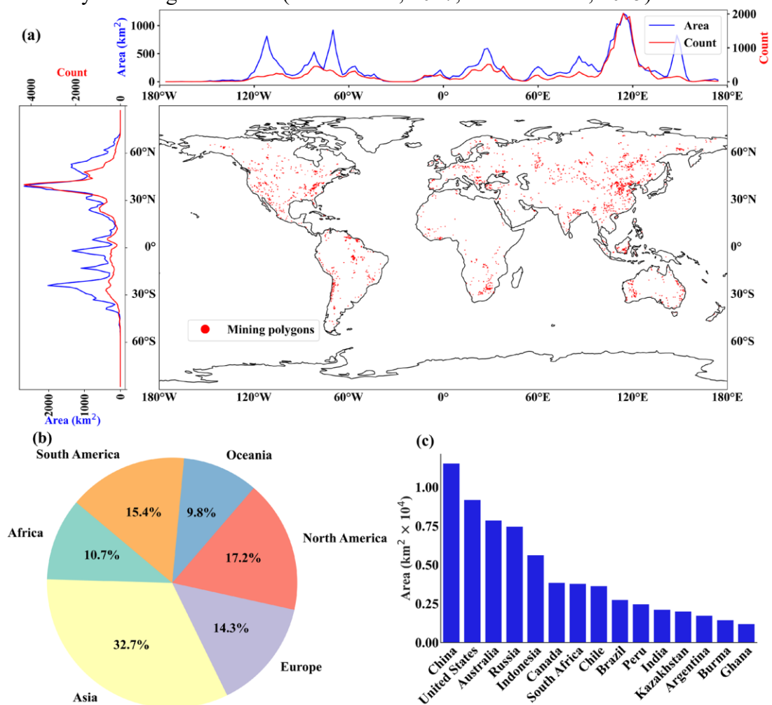
Figure. 4-5 Global distribution and characteristics of mining polygons. (a) Global distribution of mining polygons and their latitudinal/longitudinal statistics of area and count. Given the visualization effect, the centroids of the polygons are used for display here instead of the actual shapes of the polygons. (b) Continental proportion of the global mining polygons area. (c) Mining polygons area in the top 10 countries in terms of total mining area.
