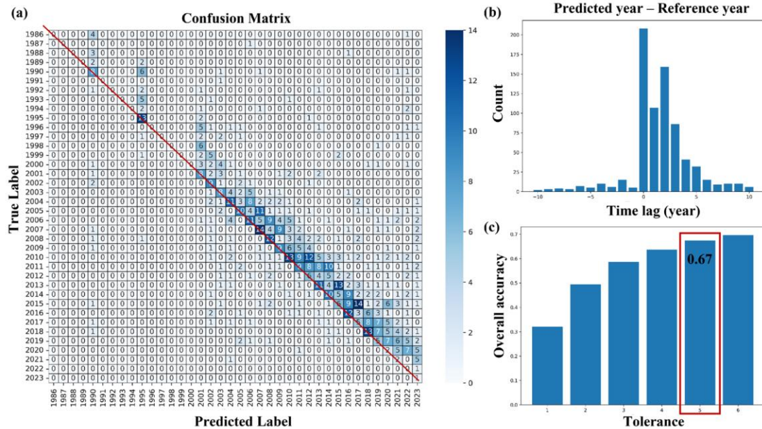
Figure. A6 A7 Validation results. (a) Confusion matrix between predicted and reference change years; (b) Histogram of temporal lags between predicted and reference years; (c) Cumulative accuracy progression with increasing tolerance thresholds, validating the robustness of the \pm 5 -year criterion.
