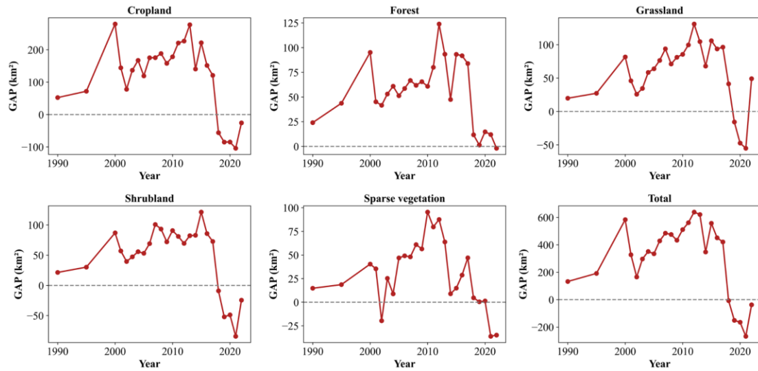
Figure. A4-A5 Annual reclamation and damage of five land cover types across continents. To ensure the continuity of the graph, the values for 1990, 1995, and 2000 represent the average annual changes over five-year intervals.
