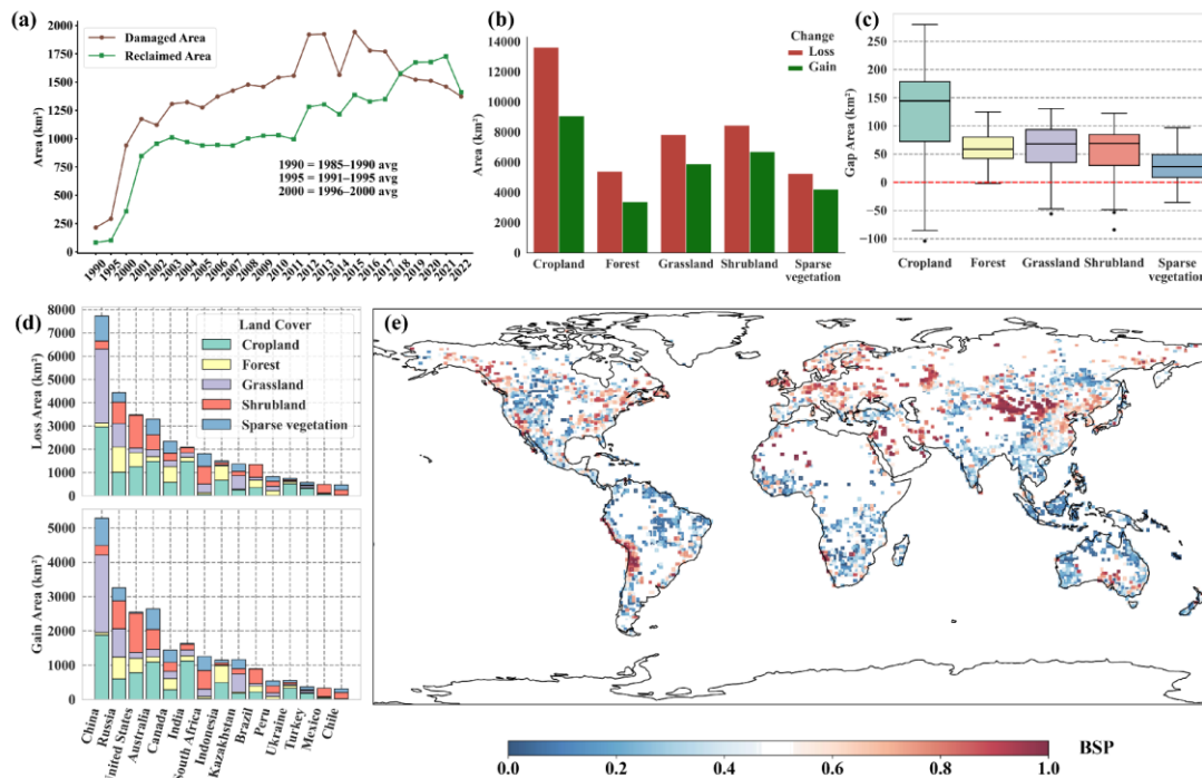
Figure. 6-7 (a) Annual land disturbance and reclamation area of global surface mines (1985-2022). To ensure the continuity of the graph, the values for 1990, 1995, and 2000 correspond to the average annual changes over five-year intervals—specifically, they represent the five-year averages for the periods 1985–1990, 1991–1995, and 1996–2000, respectively. (b) Gain and loss of land cover types during mining disturbance events. (c) Boxplot of "gap" for land cover types (gap = loss - gain). (d) Losses and gains of five land cover types in the top 15 countries ranked by total area of land with changes. (e) Percentage of bare surface area in global mining areas, aggregated to 100 km resolution (2022).
