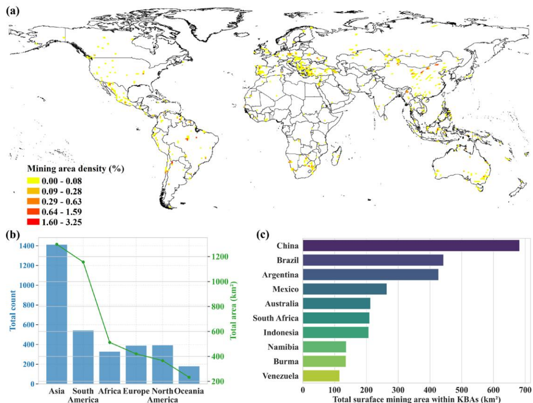
Figure. 5-6 Global distribution and characteristics of mining polygons within KBAs. (a) Global mining density within KBAs in a 100 km grid. Mining area density is calculated as the proportion of mining area within 100 x 100 km (10,000 km 2 ) grid cells. Data was aggregated using the Interrupted Goode Homolosine equal-area projection to ensure accurate area calculations. The map is displayed using the PlateCarree projection. The
