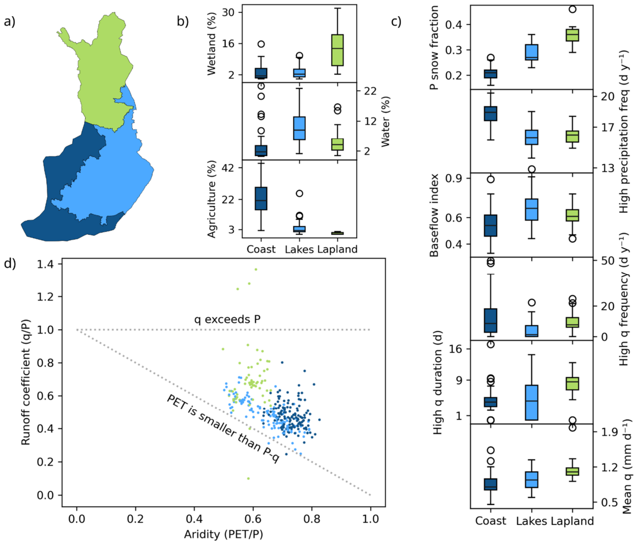
335 Figure 3. a) Map of the colours used to mark hydrological regions for the rest of the figure b) Variation in land cover between regions c) Variation in climate and discharge regime between regions. Baseflow calculated with the methodology of Ladson et al. (2013) d) Gauges plotted by runoff ratio and aridity. Inspiration for the figure from figure 2 of Coxon et. al. (2020)
