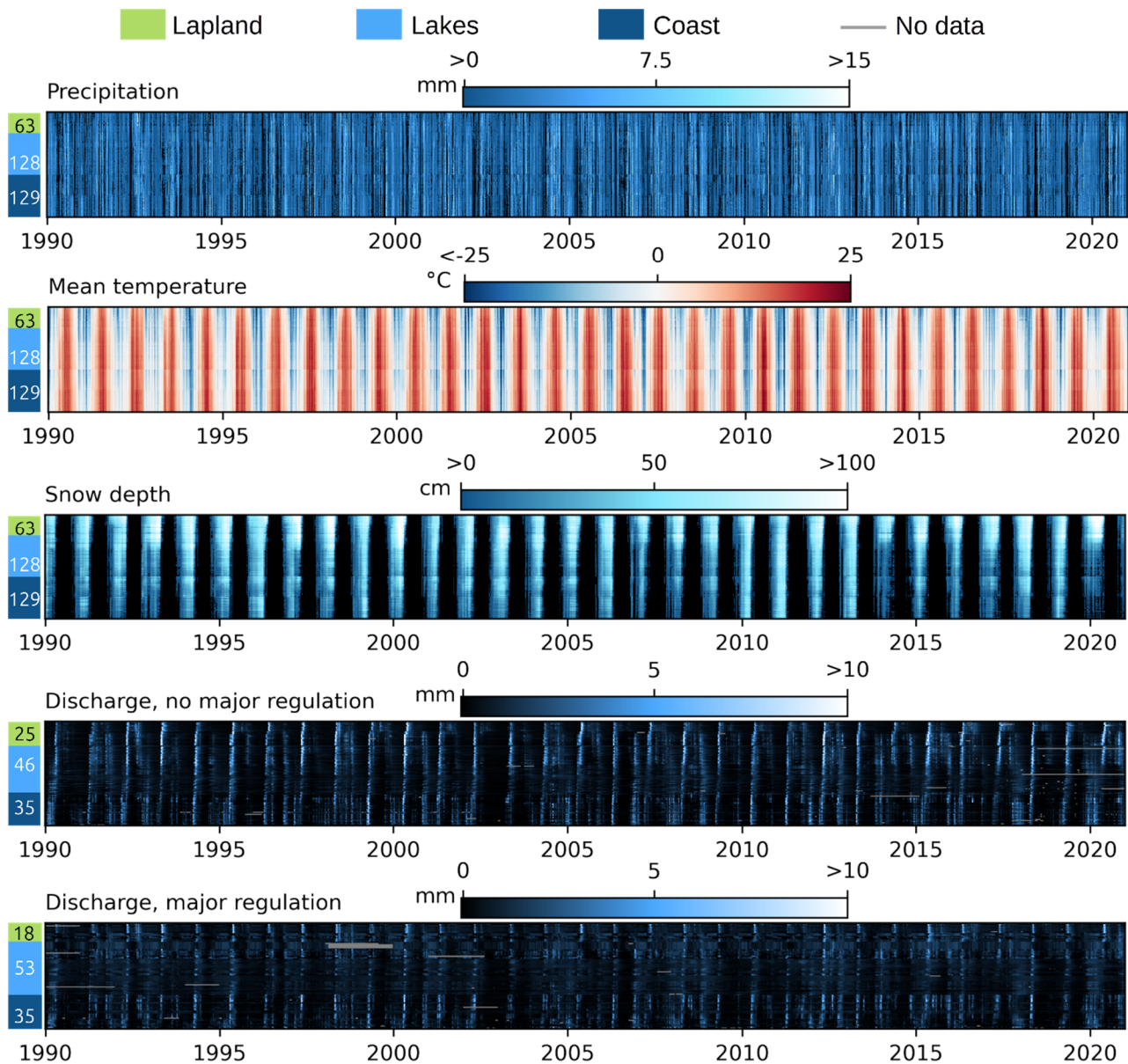
345 Figure 4. Key hydrometeorological time series for the years 1990–2020. One row of pixels corresponds to the time series of one catchment, and one column of pixels to state of all catchments at the same four-day period (resampled from one day values due to resolution limitations of the figure). Catchments have been vertically sorted first into hydrological regions (Lapland, Lakes or Coast) and then by mean temperature, placing colder catchments at the top of each region. The hydrological region bar on the left shows the region of the catchments on its right, as well as number of catchments per region. For visual clarity, only gauges with fewer than 800 missing days during the period 350 were chosen for plotting specific discharge and catchments with major regulation were plotted separately. The value ranges do not show the full ranges of the variables to place emphasis on typical behaviour of catchments instead of extremes. Full ranges are described in Appendix B. Precipitation and snow depth are shown as black when they have been zero to distinguish them from days with values slightly above zero
