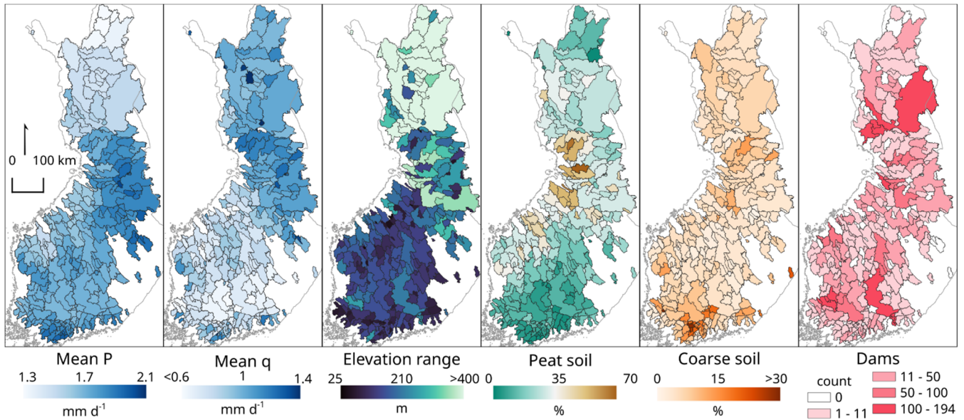
365 Figure 5. Multiple attributes exhibit great spatial variation over Finland. It should be noted that color scale for daily mean specific discharge starts from 0.6 \text{ mm d}^{-1} , because the anomalously low discharges of gauge 3727 ( 0.19 \text{ mm d}^{-1} ) would have made variation of other catchments harder to see. Similarly, shown elevation range was capped at 400 m (max. 804 m) to keep variation outside of Lapland visible and coarse soil percentage was capped at 30 % (max. 48 %) due to a few small outlier catchments covered by major glaciofluvial deposits.
