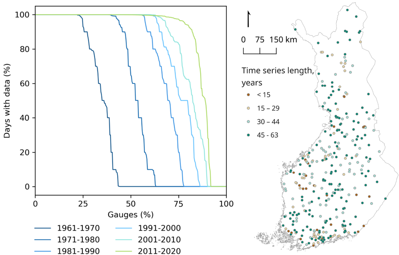
225 Figure 2. Time series length of hydrologic observations in CAMELS-FI. The number of gauges has increased gradually over the years, but some have also been decommissioned.
